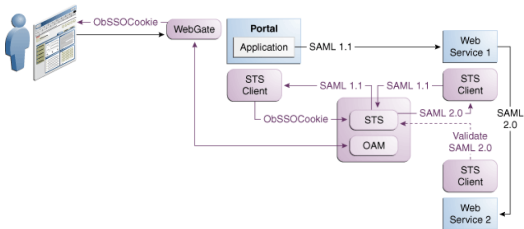
Figure 41-5 Web Services SSO
