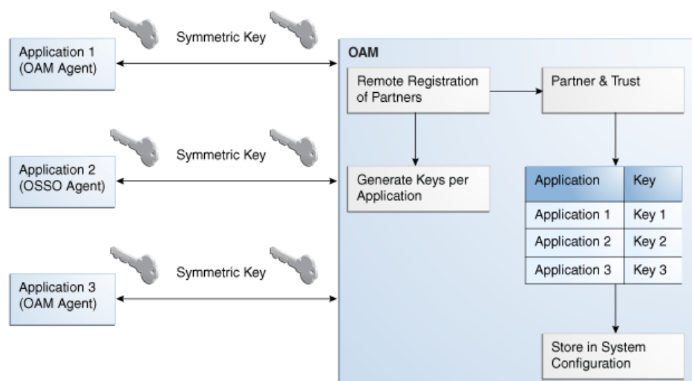
Figure 15-5 Key Generation
