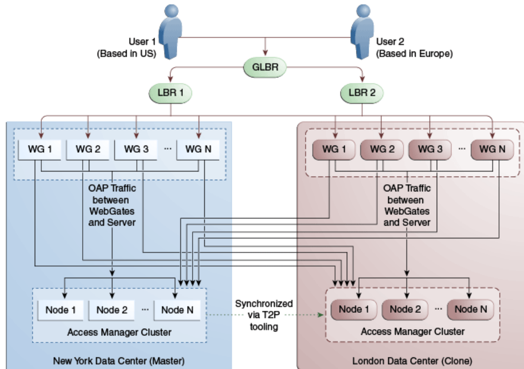
Figure 17-9 Active-Active Topology
