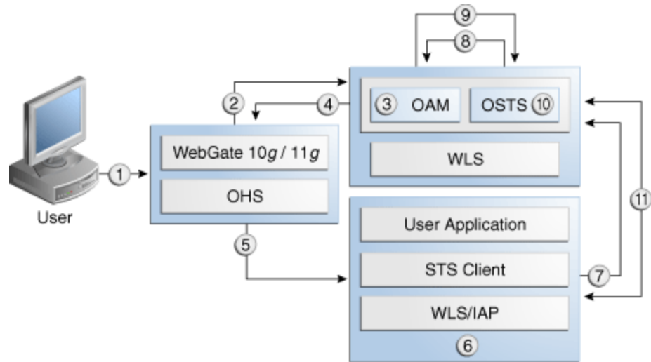
Figure 42-5 Identity Propagation Processing
