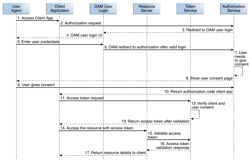
Figure 52-1 OAuth 3-Legged Flow Diagram
