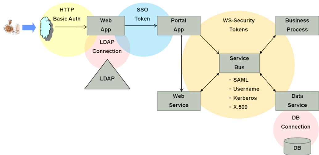
Figure 55-1 End to End Identity Context Process
