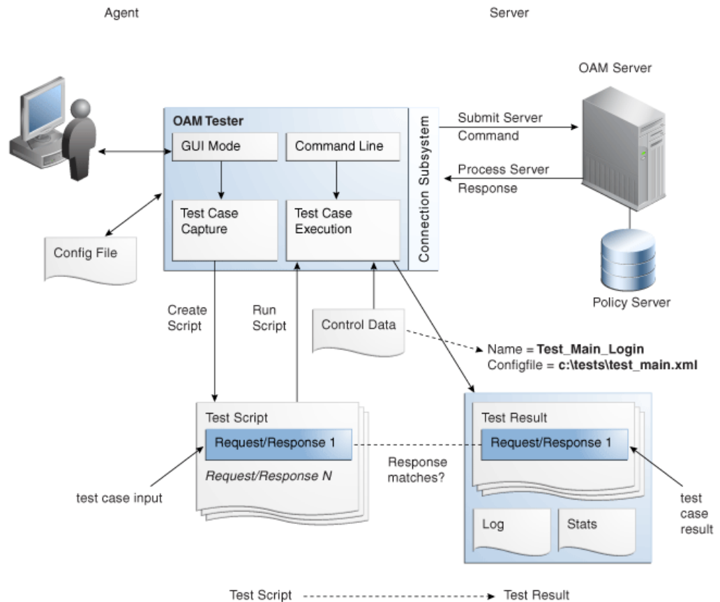
Figure 26-2 User Interactions with the Access Tester
