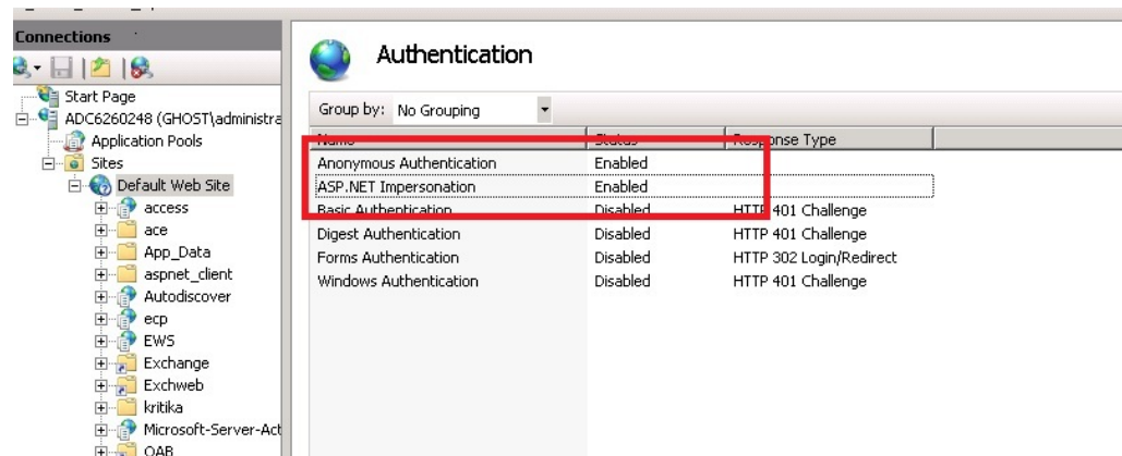
Figure 60-4 Impersonation Authentication
