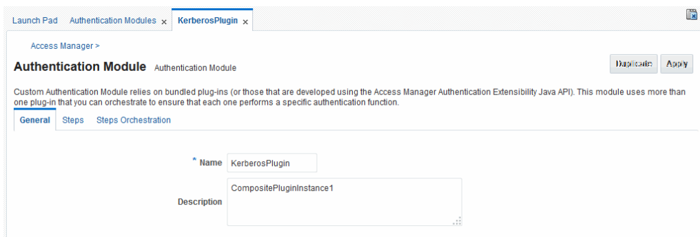
Figure 22-13 KerberosPlugin
