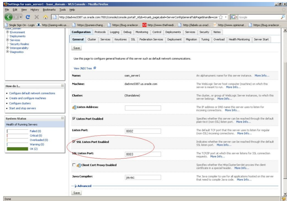
Figure 23-6 Enable SSL
