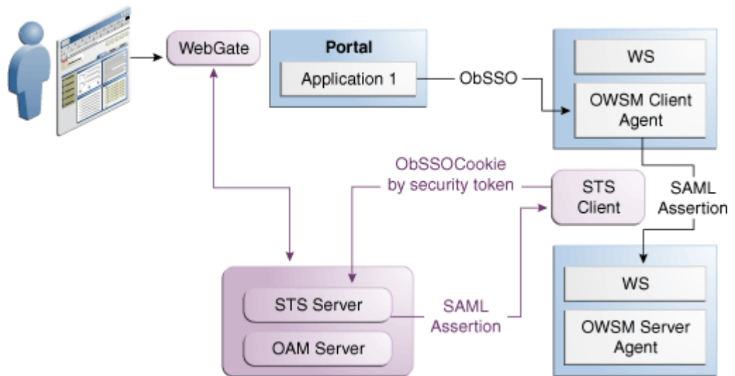
Figure 41-3 Token Translation at a Centralized Authority
