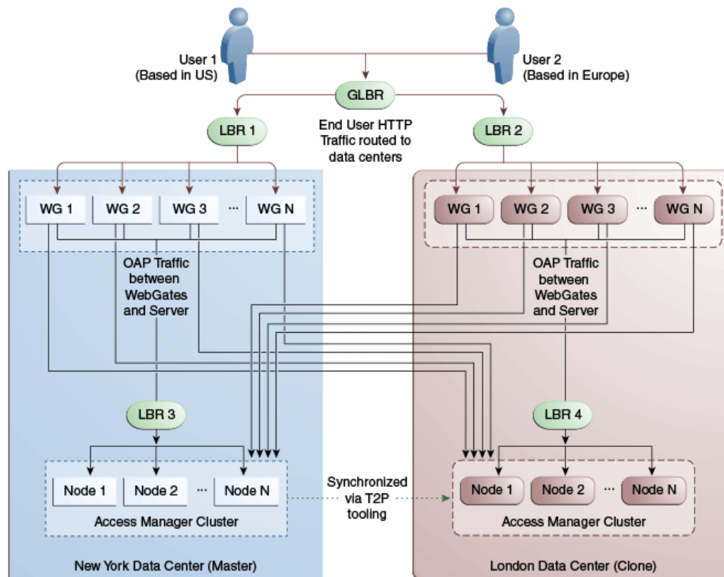
Figure 17-11 Load Balancing Access Manager Components
