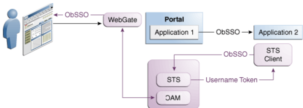
Figure 41-4 Translating Tokens Behind a Firewall
