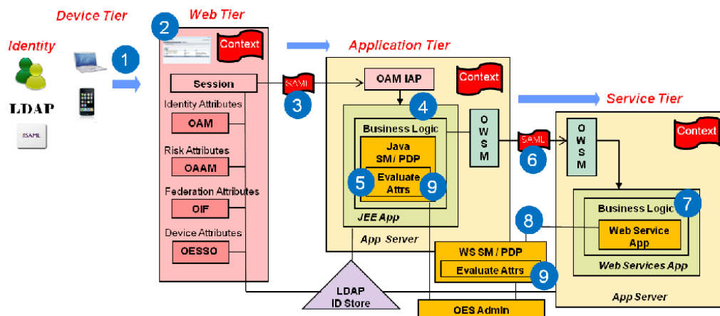
Figure 55-3 Identity Context Process Flow
