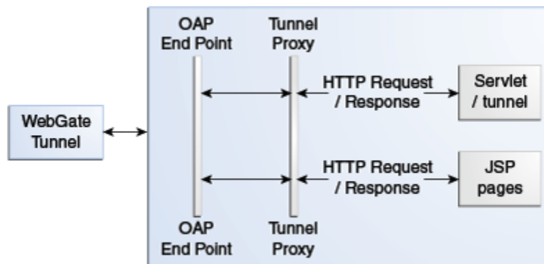
Figure 23-5 OAP Tunneling with DCC
