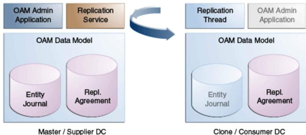
Figure 19-1 Replication Flow
