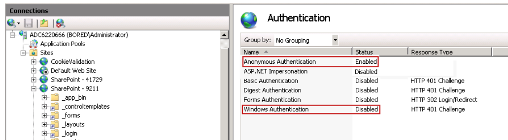
Figure 59-5 Impersonation Authentication
