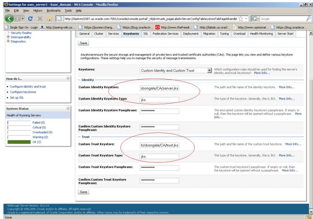
Figure 23-7 Keystore Configuration
