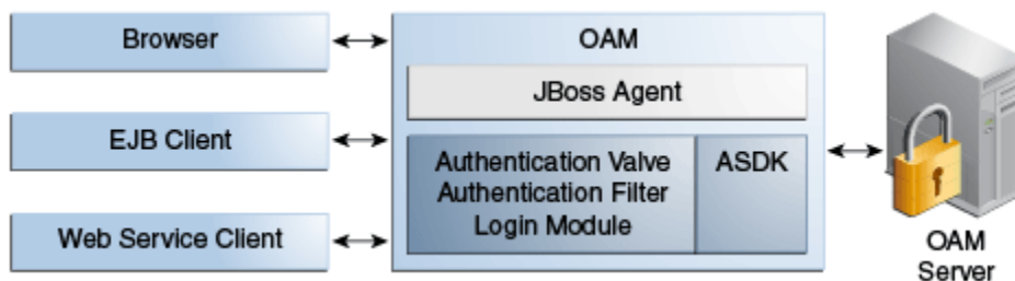
Figure 58-1 Various Clients Deployed on JBoss Application Server
