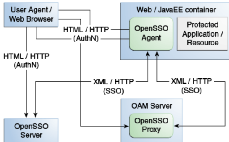
Figure 28-1 Typical Deployment with OpenSSO and Access Manager
