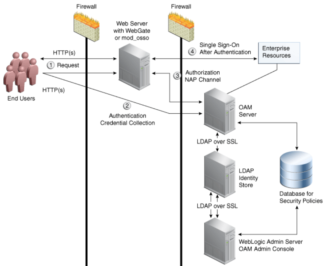
Figure C-1 Communication Channels for OAM Servers and WebGates
