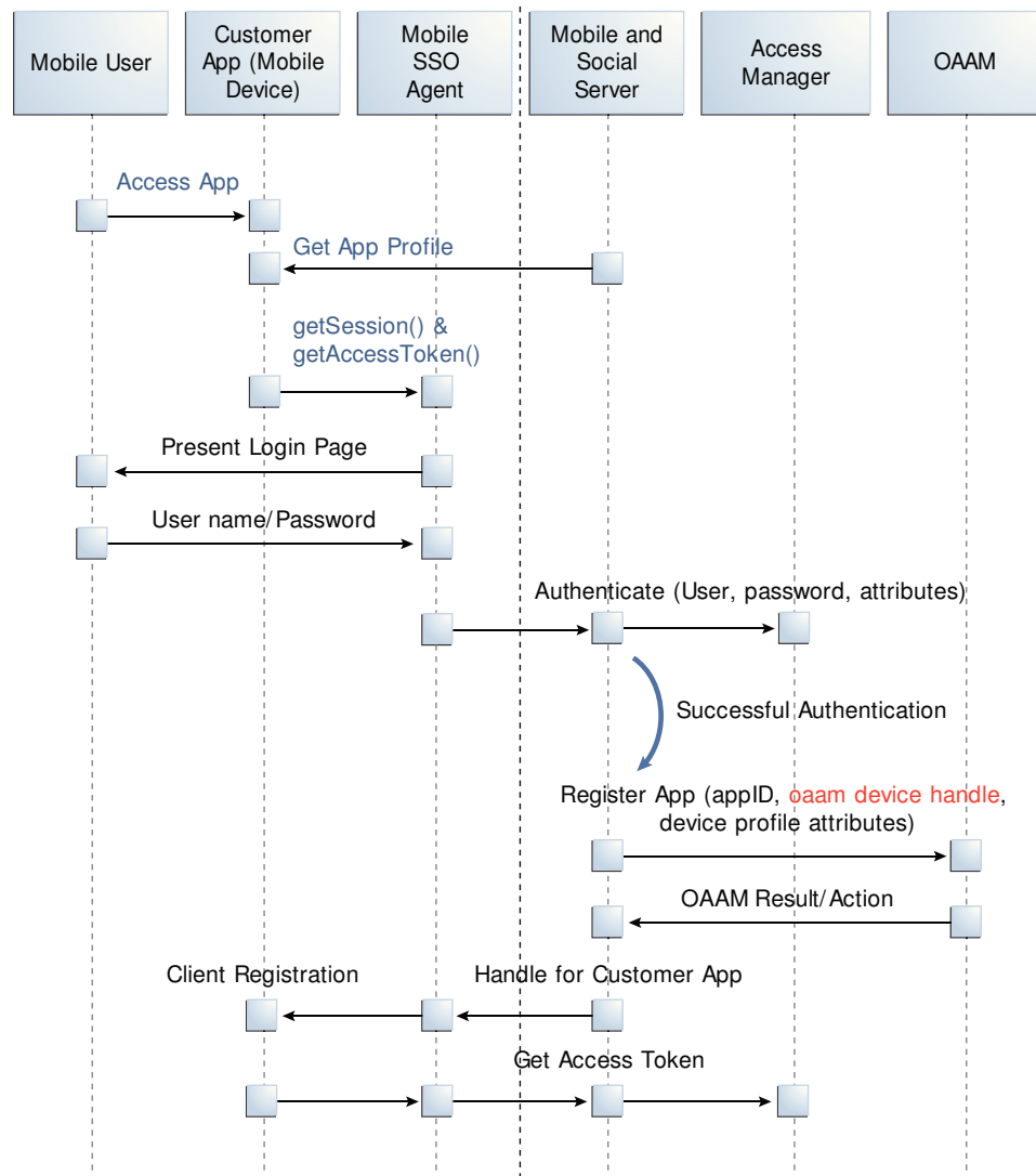
Figure 48-2 Mobile SSO Agent Requests Access Token from Access Manager
