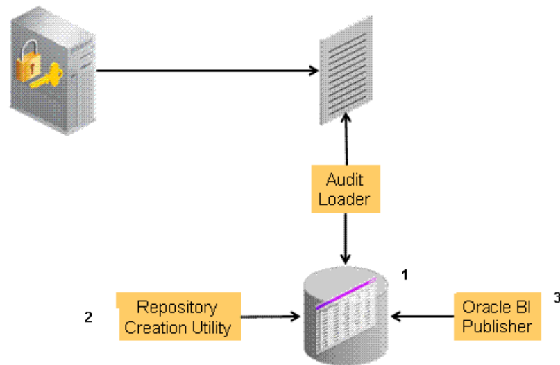
Figure 8-1 Audit to Database Architecture
