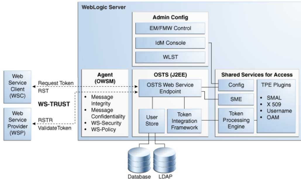
Figure 41-1 Security Token Service Architecture
