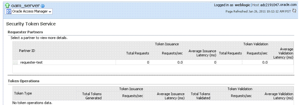
Figure 12-13 STS Component Metrics for an Individual OAM Server Instance
