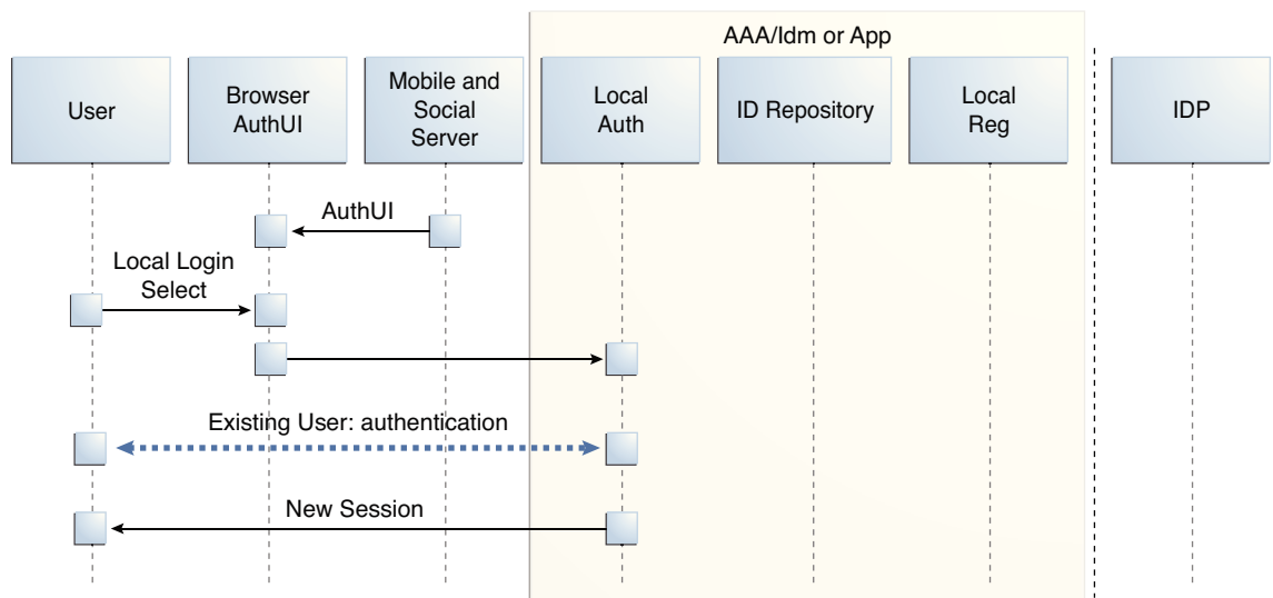
Figure 48-12 Authenticating a User Locally
