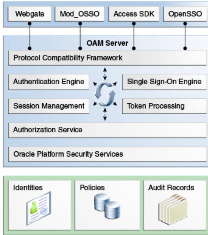
Figure 1-2 Access Manager 11g Components and Services
