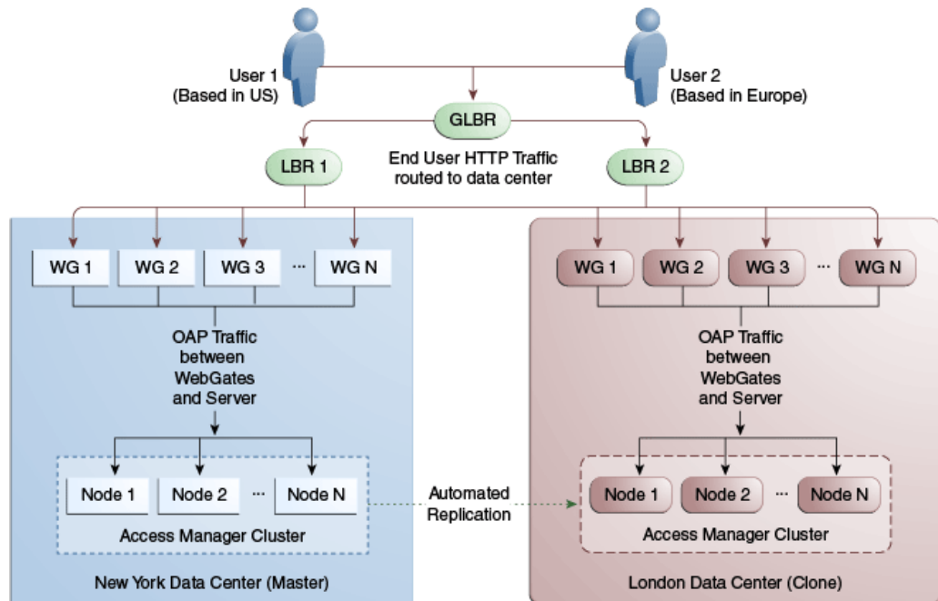
Figure 17-8 Traditional MDC Deployment
