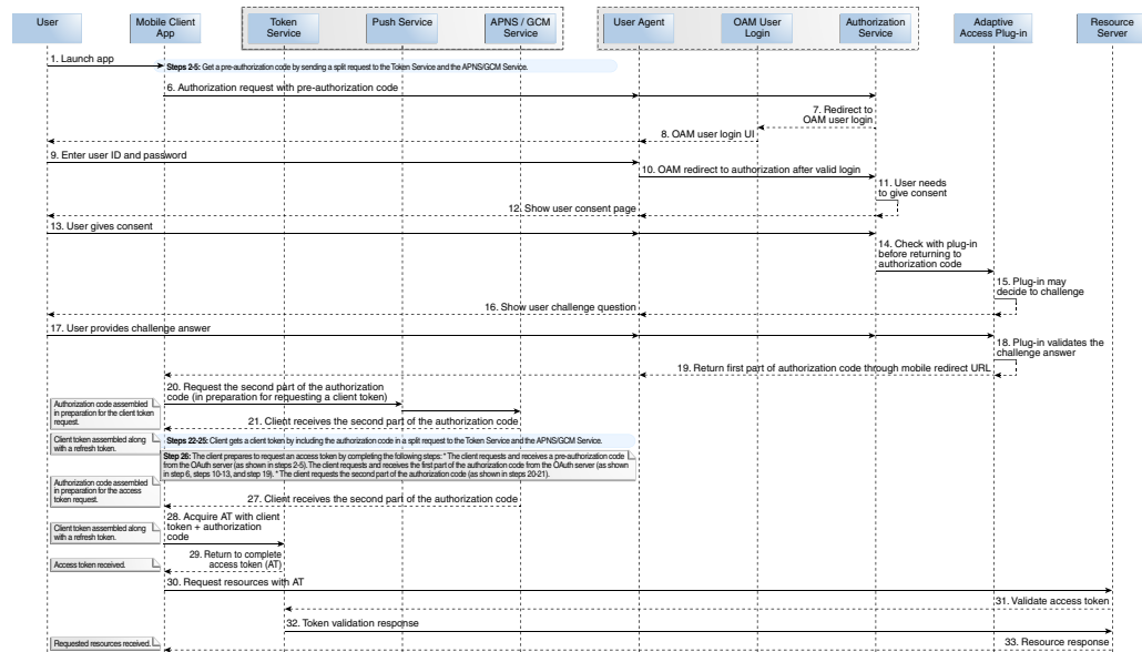
Figure 52-3 The Complete Mobile App Authorization Request Flow
