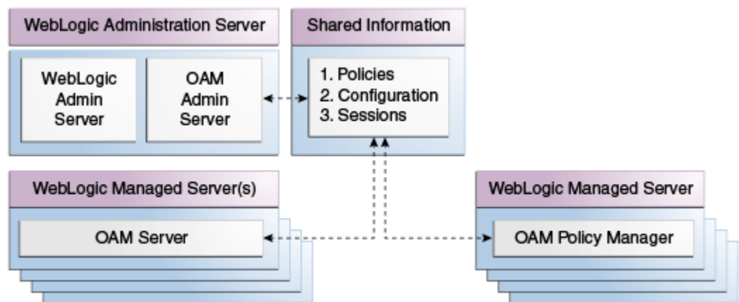
Figure 1-3 Access Manager 11g Component Distribution
