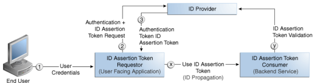
Figure 42-3 Process Flow During Identity Propagation
