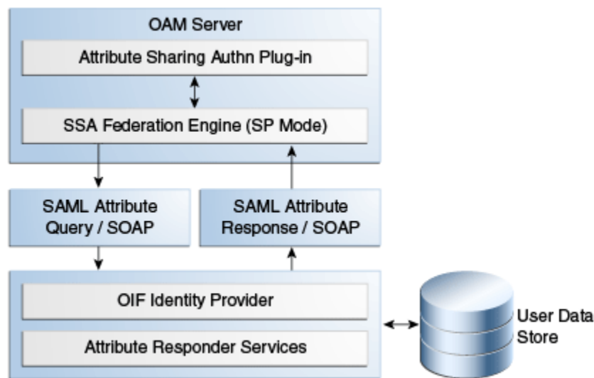
Figure 38-4 Attribute Sharing Plug-in Design
