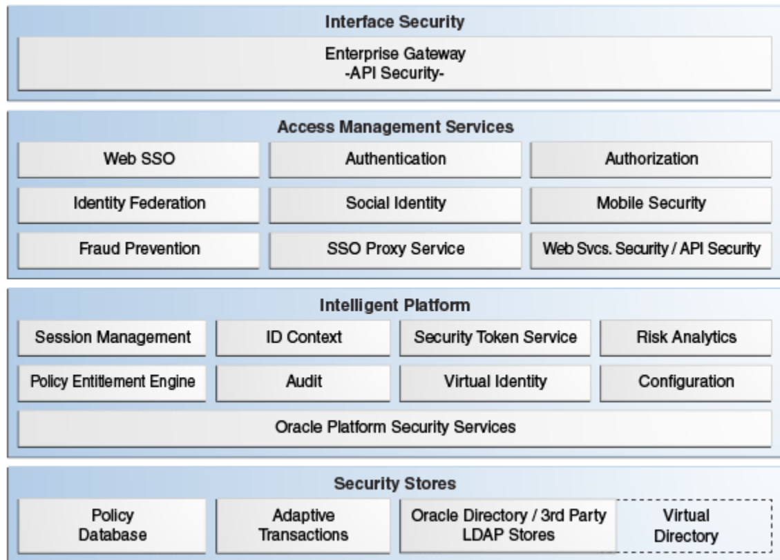
Figure 1-1 Oracle Access Management Overview
