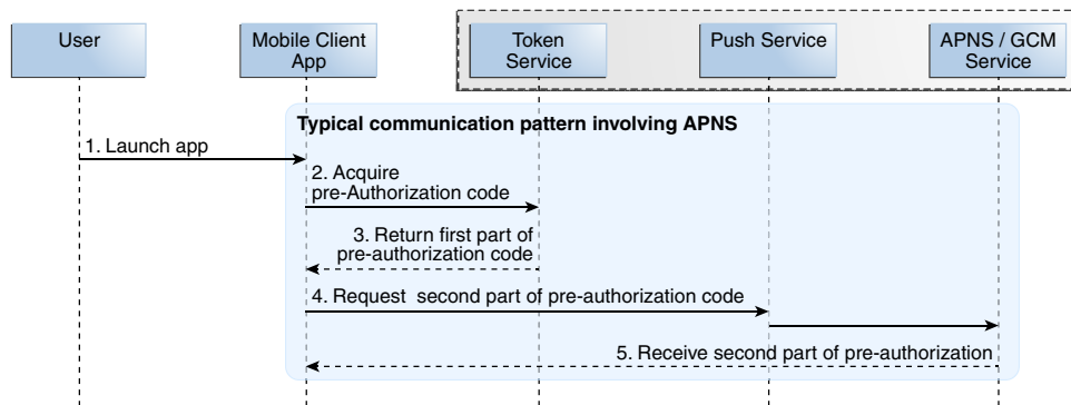
Figure 52-2 Using a Split Request to get a Client Verification Code
