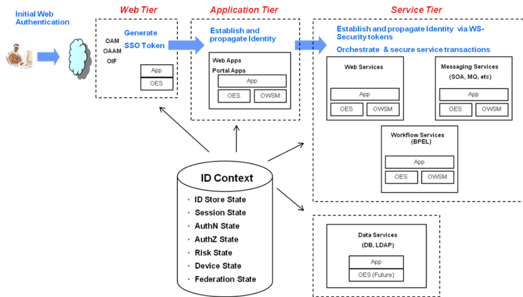
Figure 55-2 End To End Identity Context Process Components
