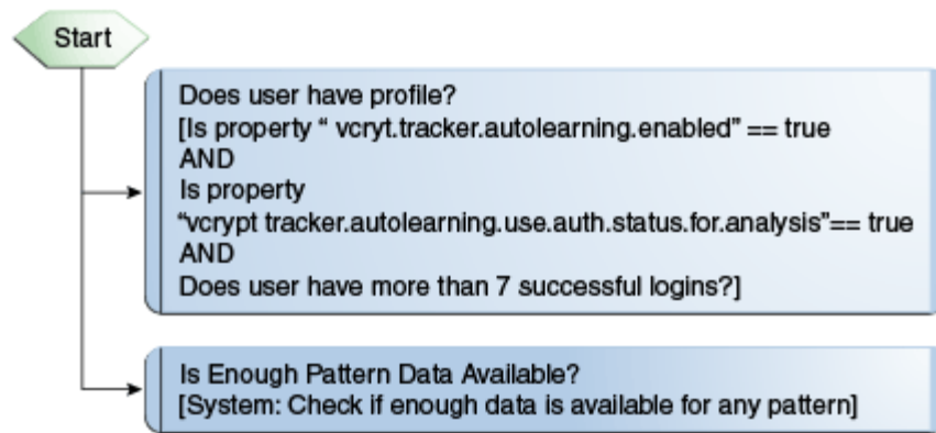
Figure 10–18 Autolearning (Pattern-Based) Policy: OAAM Does User Have Profile Flow
