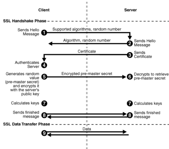
Figure 6–1 SSL Handshake
