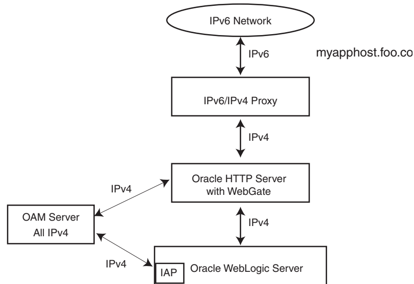
Figure 15–1 Simple Authentication with the IPv6/IPv4 Proxy
