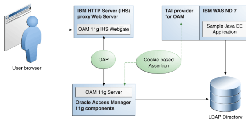
Figure 6-3 Components and Process Flow with OAM 11g and the IAP
