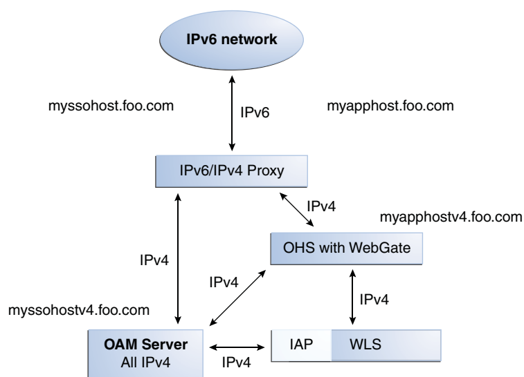
Figure 15–1 IPv6 with Access Manager and Challenge Redirect
