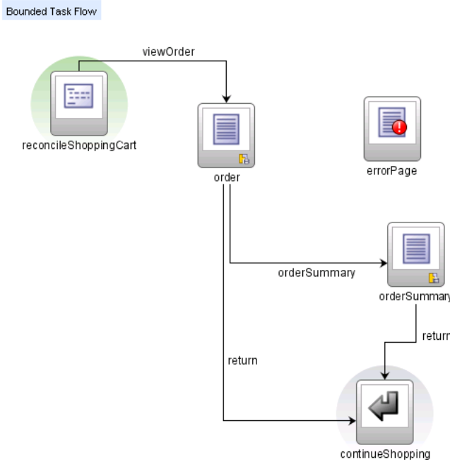
Figure 19–1 Checkout Bounded Task Flow in Fusion Order Demo Application
