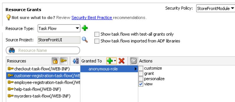
Figure 35–5 Granting to anonymous-role in the Overview Editor
