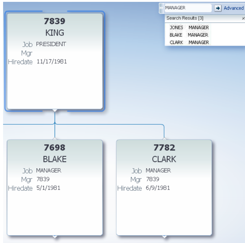
Figure 33–83 Hierarchy Viewer Search Results
