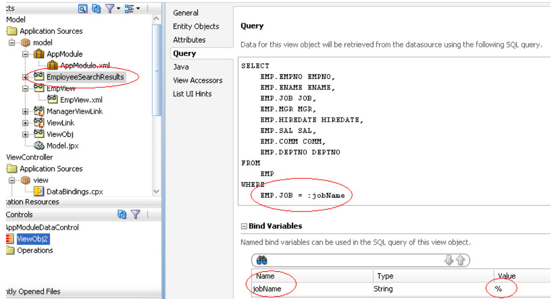
Figure 33–81 EmployeeSearchResults View Object
