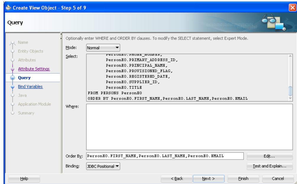
Figure 5–6 Create View Object Wizard, Query Page
