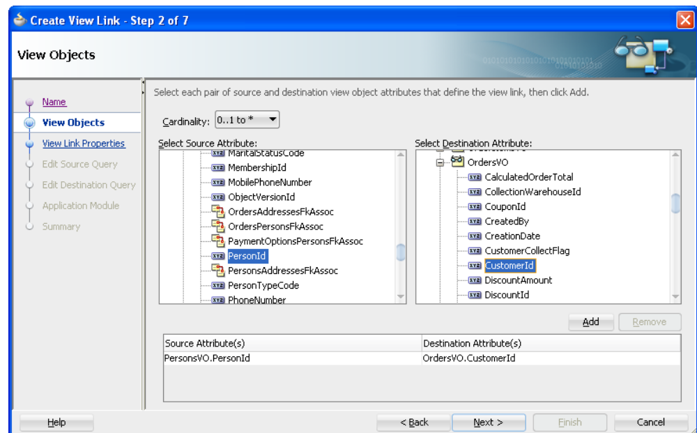
Figure 5–25 Defining Source/Target Attribute Pairs While Creating a View Link
