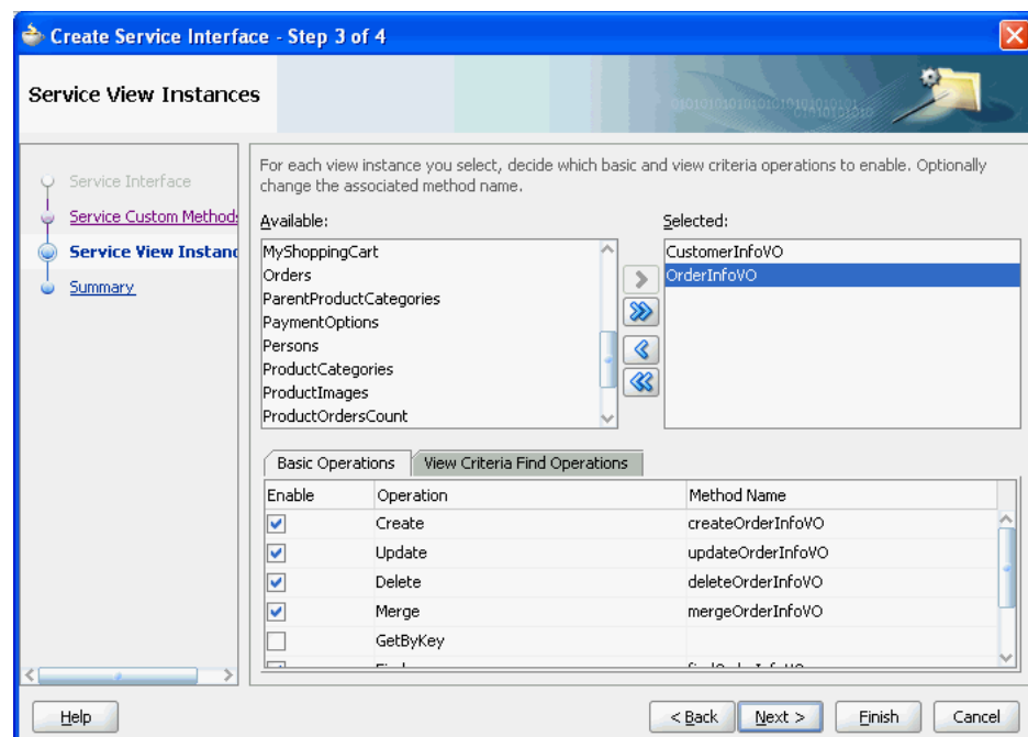
Figure 11-1 View Instances and CRUD Operation Selection
