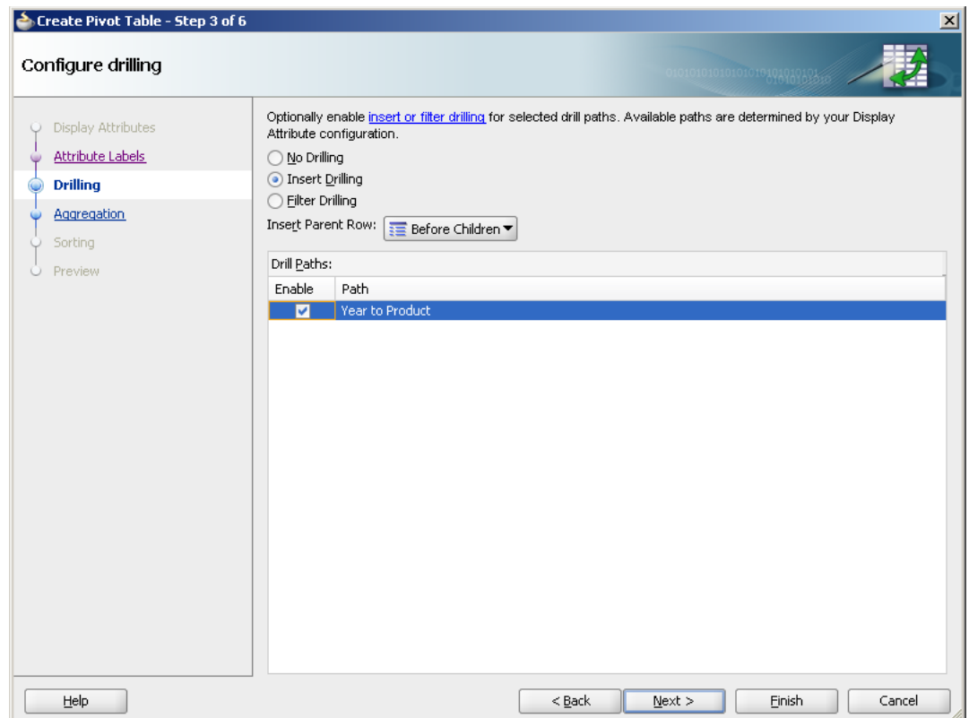
Figure 33–30 Configure Drilling Page of Create Pivot Table Wizard
