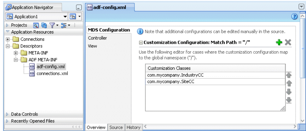
Figure 39-3 adf-config.xml Overview Editor
