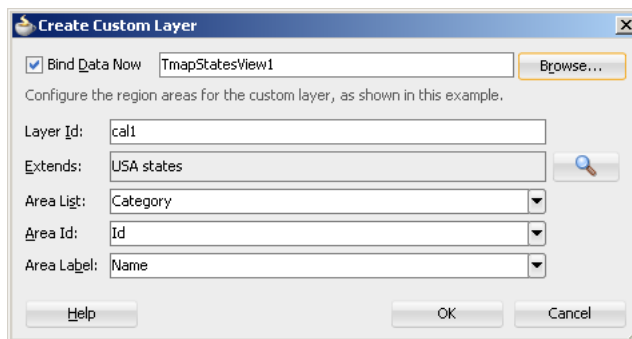
Figure 33–65 Create Custom Layer Dialog
