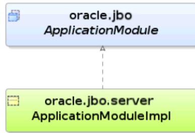
Figure 3–4 ADF Business Components Separate Interface and Implementation
