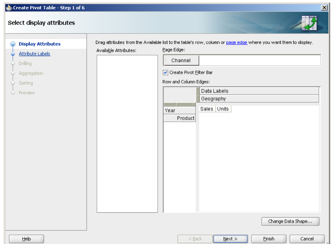
Figure 33–26 Select Display Attributes Page of Create Pivot Table Wizard
