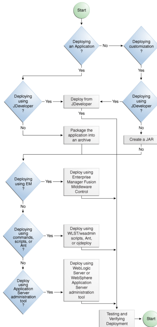
Figure 41–5 Application Deployment Flow Diagram
