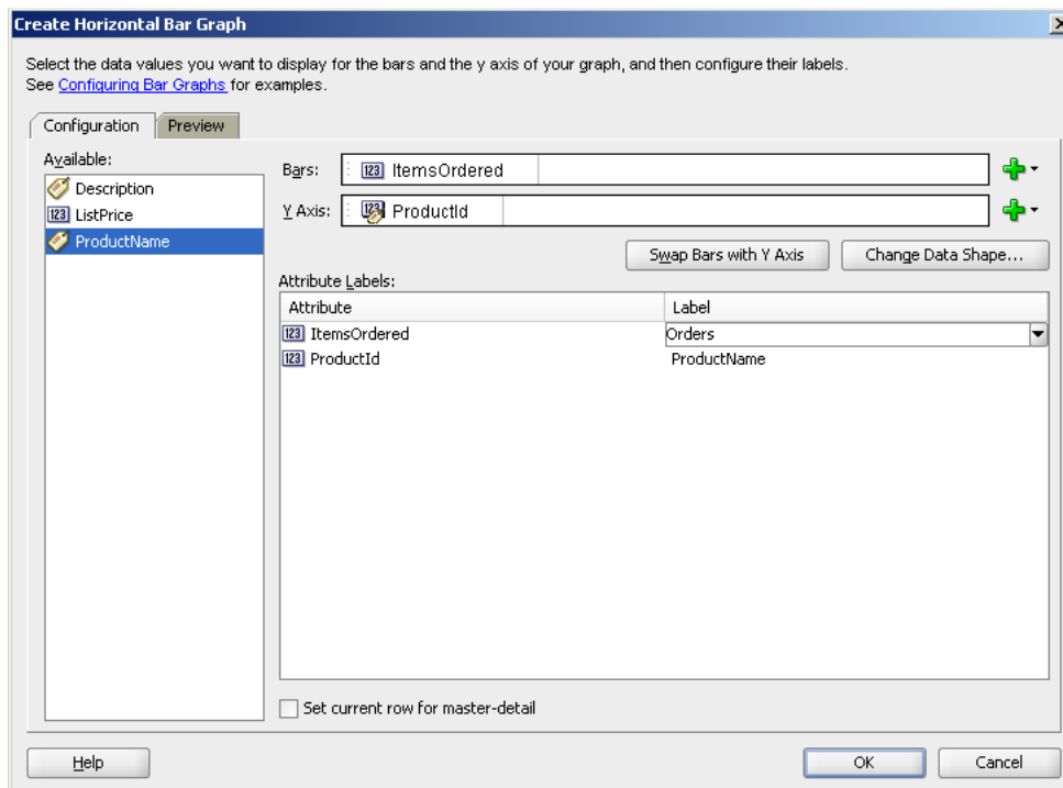
Figure 33–4 Create Horizontal Bar Graph Dialog for ProductOrdersCount
