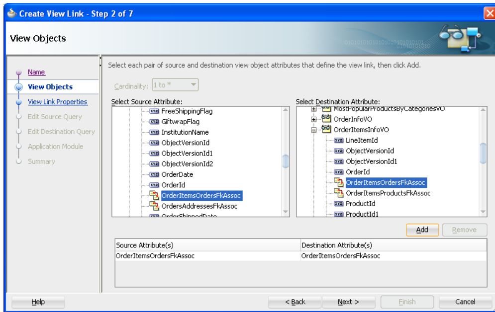
Figure 5–24 Master and Detail Related by an Association Selection
