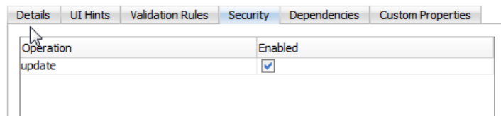
Figure 35-12 Permission Enabled on update Operation for an ADF Entity Object Attribute
