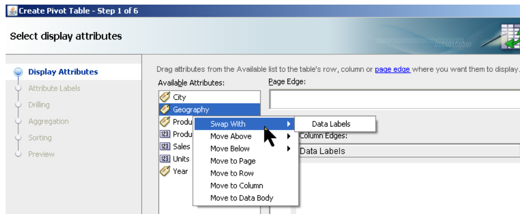
Figure 33–25 Display Attributes Context Menu
