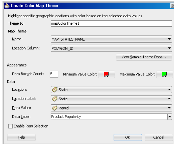
Figure 33–43 Create Color Map Theme for Product Popularity By State
