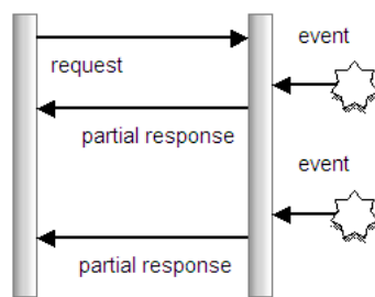
Figure 45-3 Streaming Mode
