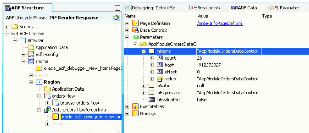
Figure 36-43 Parameters Selected for the ADF Data Window
