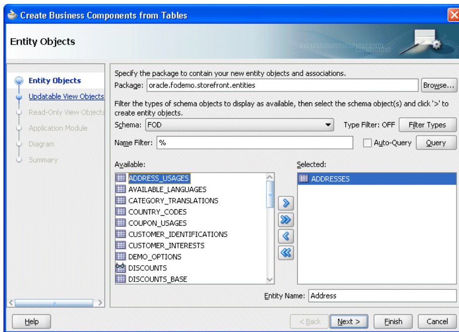
Figure 4-2 Create Business Components from Tables Wizard, Entity Objects Page
