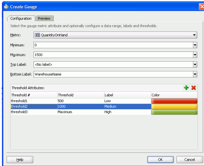
Figure 33–21 Create Gauge Dialog for Warehouse Inventory Gauge Set
