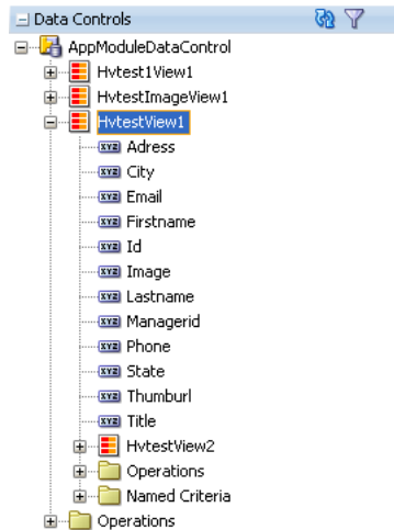
Figure 33–77 Data Collection for Personnel Organizational Chart
