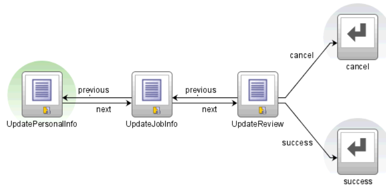
Figure 22–2 Task Flow Return Activities in Called Bounded Task Flow
