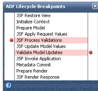
Figure 36–24 ADF Lifecycle Phase Breakpoints Enabled in the ADF Lifecycle Breakpoints Window
