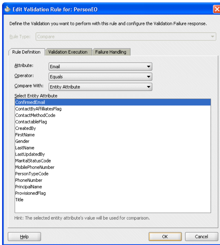
Figure 7–2 Compare Validator Using an Entity Object Attribute
