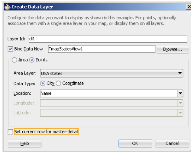
Figure 33–53 Create Point Data Layer Dialog
