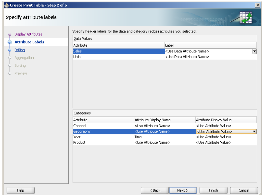
Figure 33–27 Specify Attribute Labels Page of Create Pivot Table Wizard
