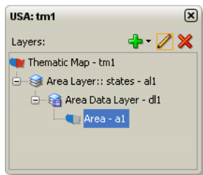
Figure 33–50 Thematic Map Layer Browser
