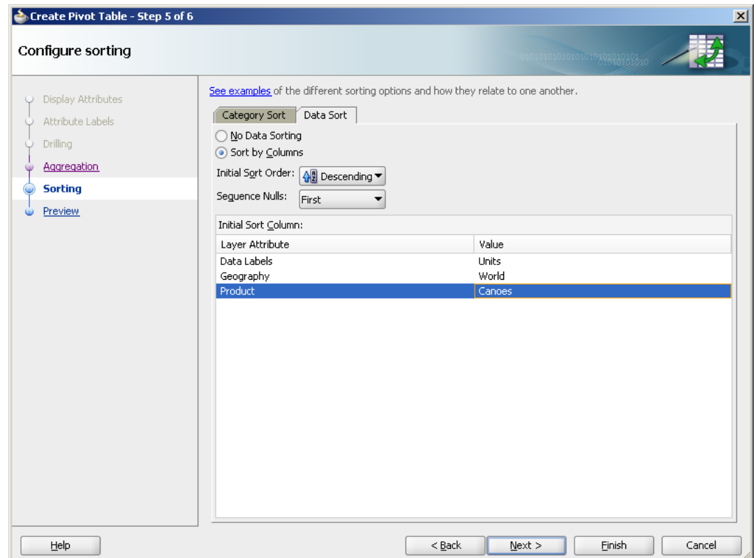
Figure 33–35 Data Sort Page of the Create Pivot Table Wizard
