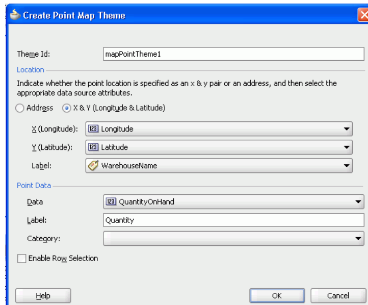
Figure 33–40 Create Point Map Theme Dialog for Warehouse Inventory Levels
