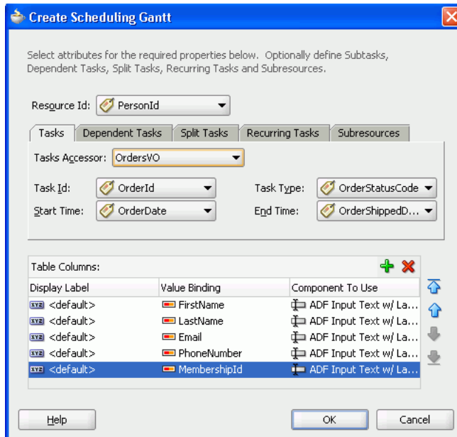
Figure 33–75 Create Scheduling Gantt Dialog
