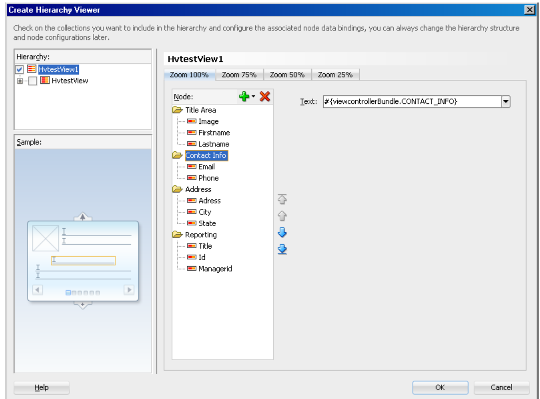
Figure 33–79 Create Hierarchy Viewer Dialog
