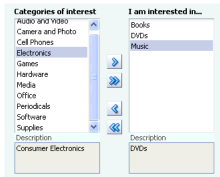
Figure 30–7 SelectManyShuttle Component
