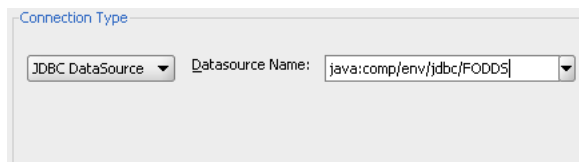
Figure 9–10 JDBC DataSource Connection Type Setting in Edit Business Components Configuration Dialog
