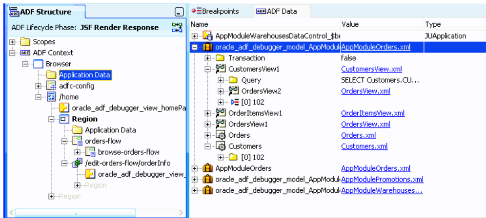
Figure 36–47 Application Data for ADF Business Components Business Services
