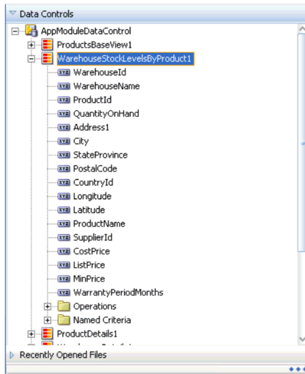
Figure 33–39 Data Collection for Warehouse Stock Levels
