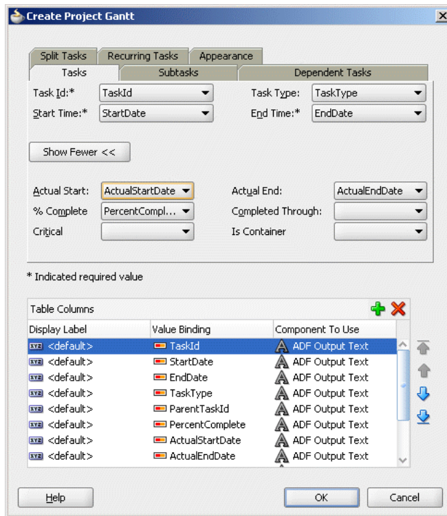
Figure 33–69 Create Project Gantt Dialog for Orders Shipped
