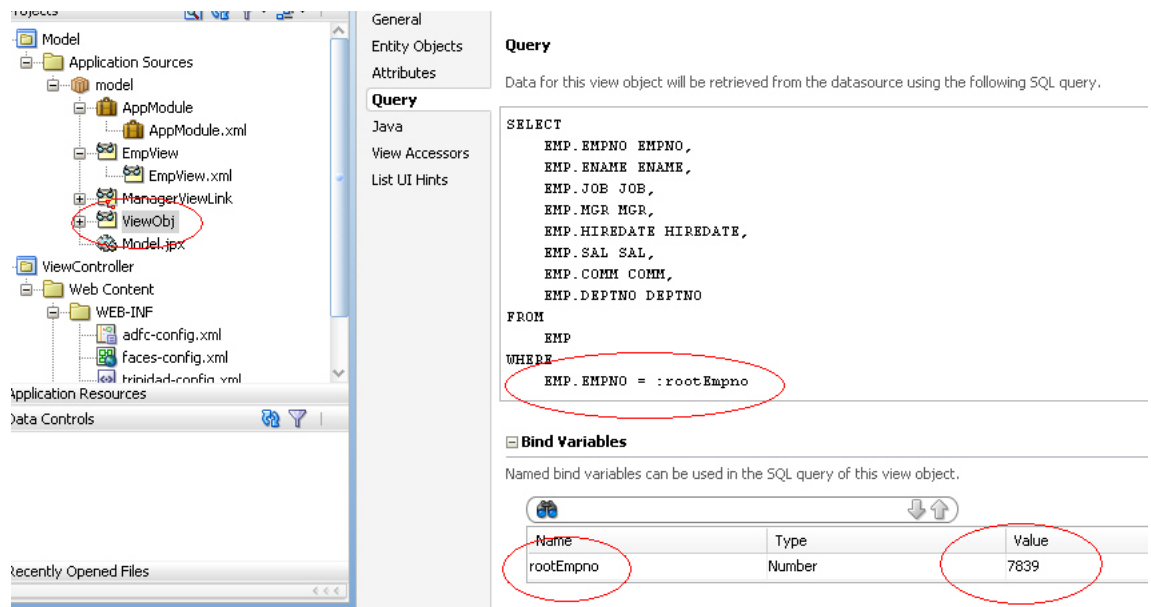
Figure 33–80 Root Node Query
