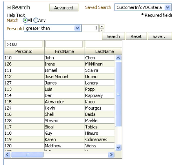
Figure 31–22 Query Search Form with Filtered Table
