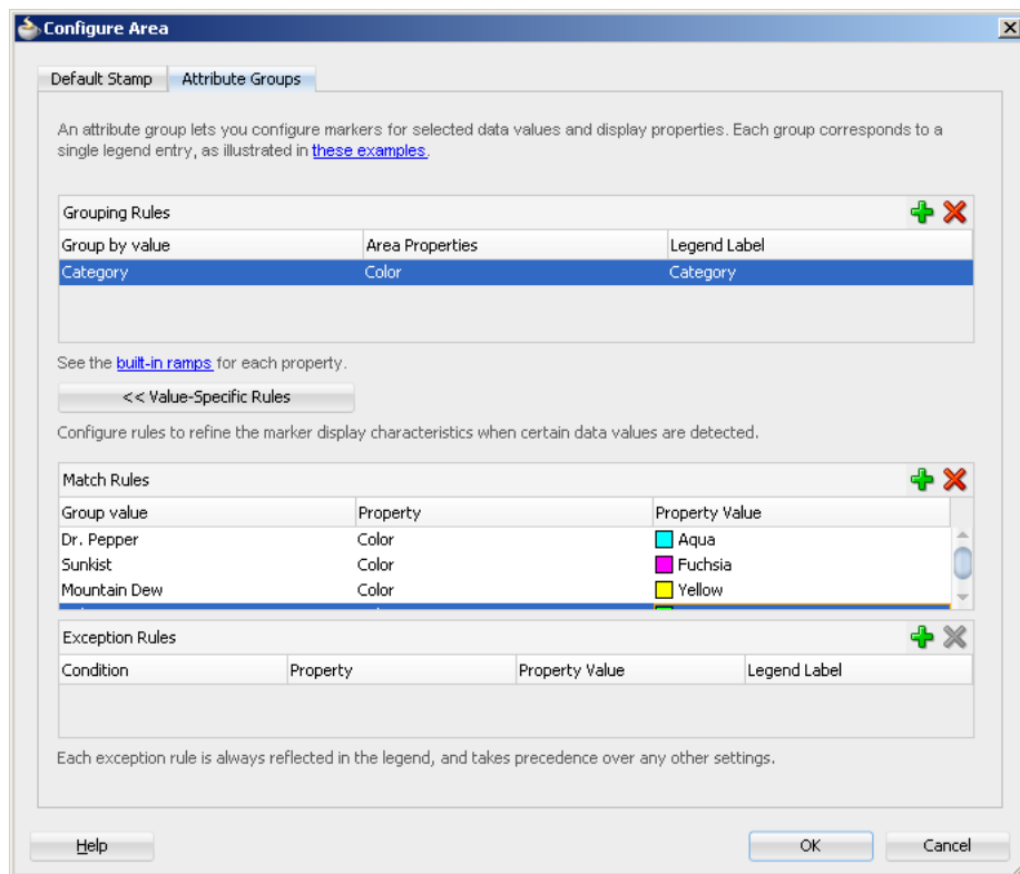
Figure 33–51 Configure Area Dialog Attribute Groups Page
