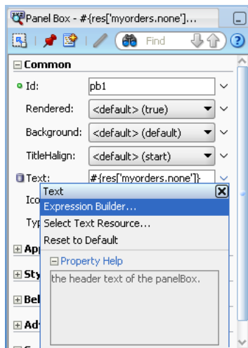
Figure 10–4 Opening the Expression Builder for an Attribute in the Property Inspector
