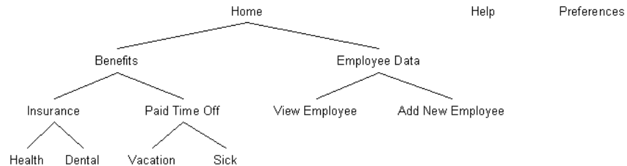
Figure 20–14 Sample Page Hierarchy
