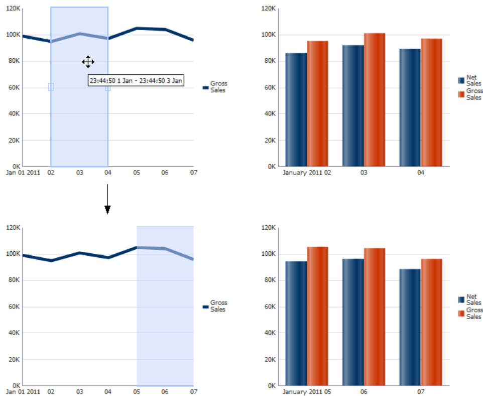
Figure 22–43 Time Selector in Master-Detail Graph
