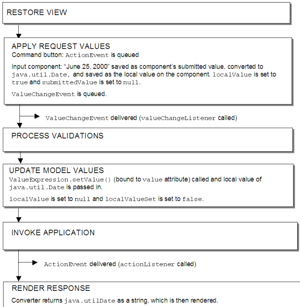
Figure 5–4 Immediate Attribute on an Input Component
