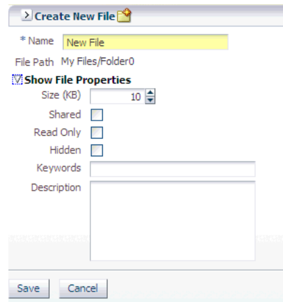
Figure 11–3 Form Uses Input Components
