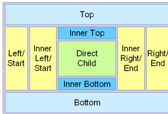
Figure 9–18 Facets in panelBorderLayout
