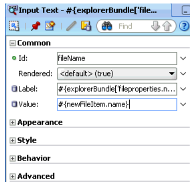
Figure 3–10 JDeveloper Property Inspector
