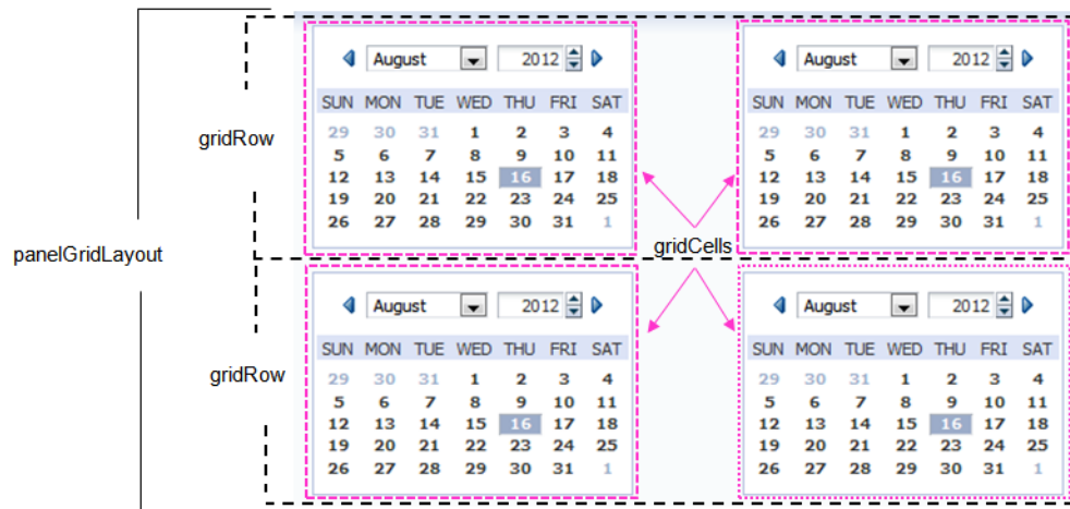
Figure 9–16 Simple Grid Layout with Two Rows Each with Two Cells
