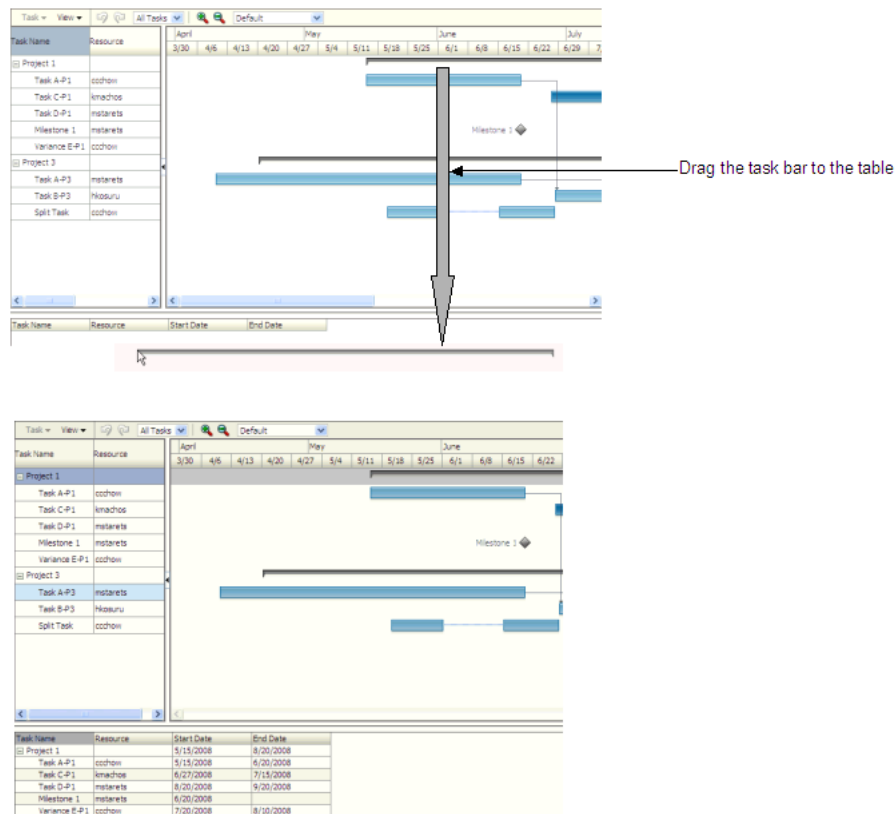
Figure 33–6 Dragging and Dropping an Object
