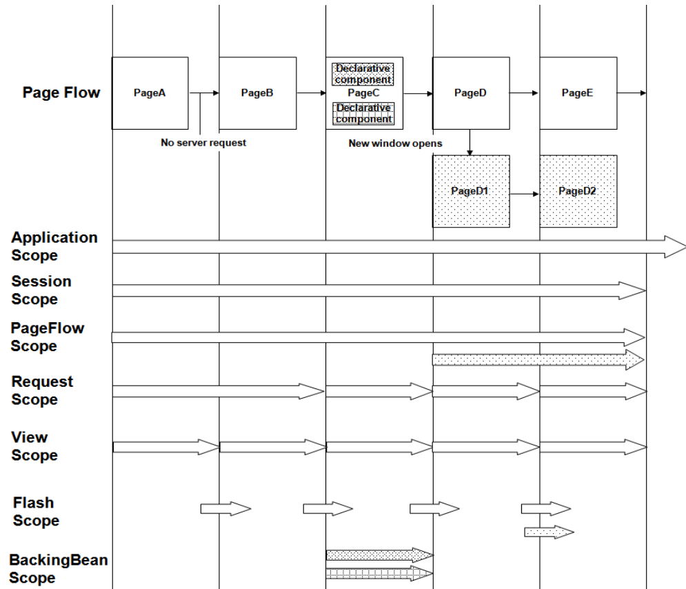
Figure 5–11 Relationship Between Scopes and Page Flow
