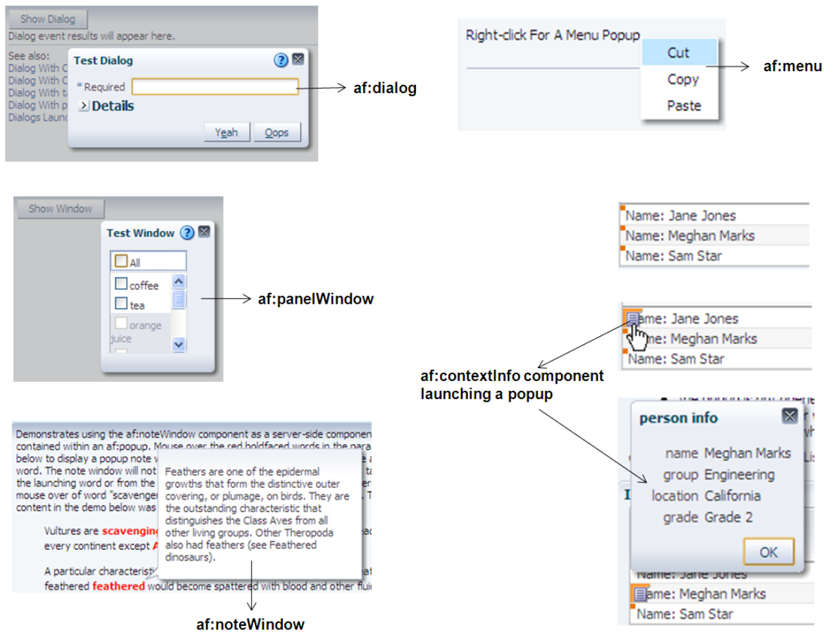
Figure 15–1 ADF Faces Components for Dialogs, Menus, and Windows
