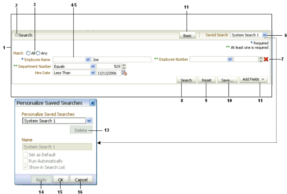
Figure 14–4 Query Component and Associated Popup Dialog
