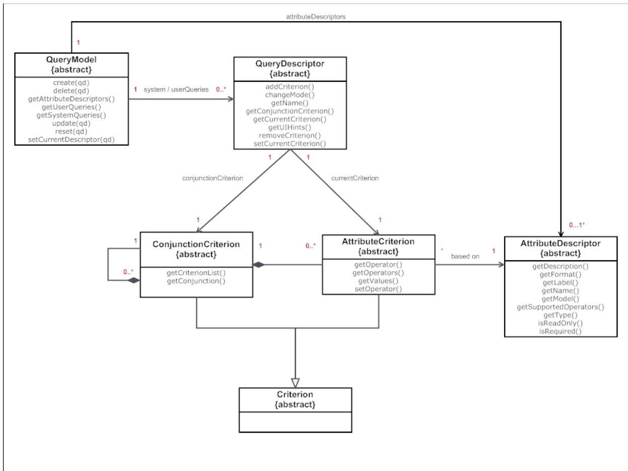
Figure 14–3 Class Diagram for QueryModel
