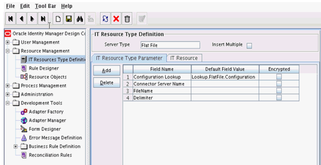
Figure 11–1 IT Resource Type Definition in Design Console
