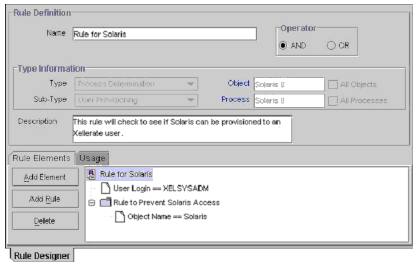
Figure 4–2 Rule Designer Form
