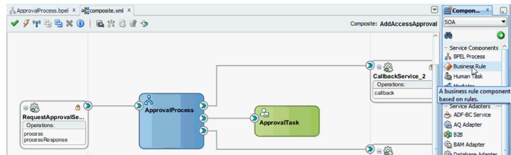
Figure 21-18 Adding Business Rule Component
