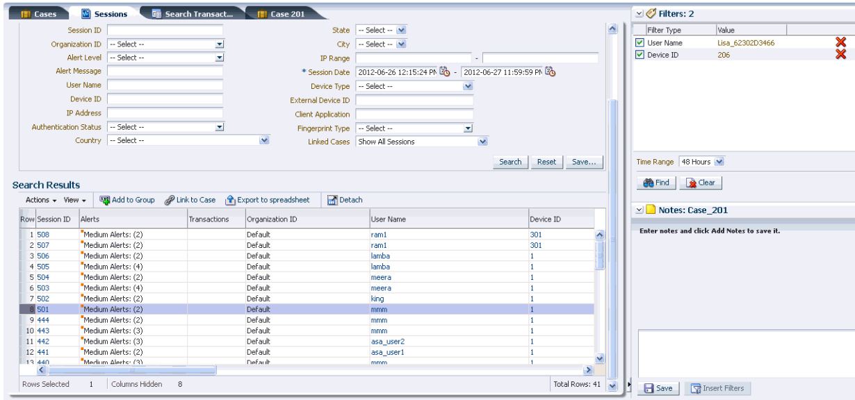
Figure 5–1 Investigation Interface
