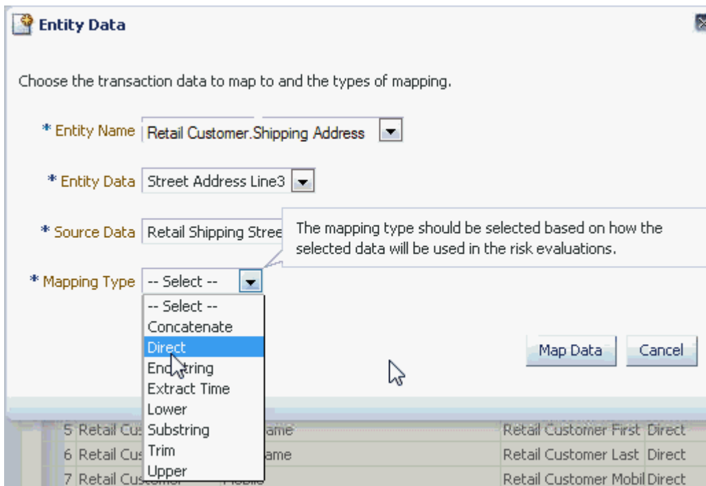
Figure 20–8 Mapping Entity Data
