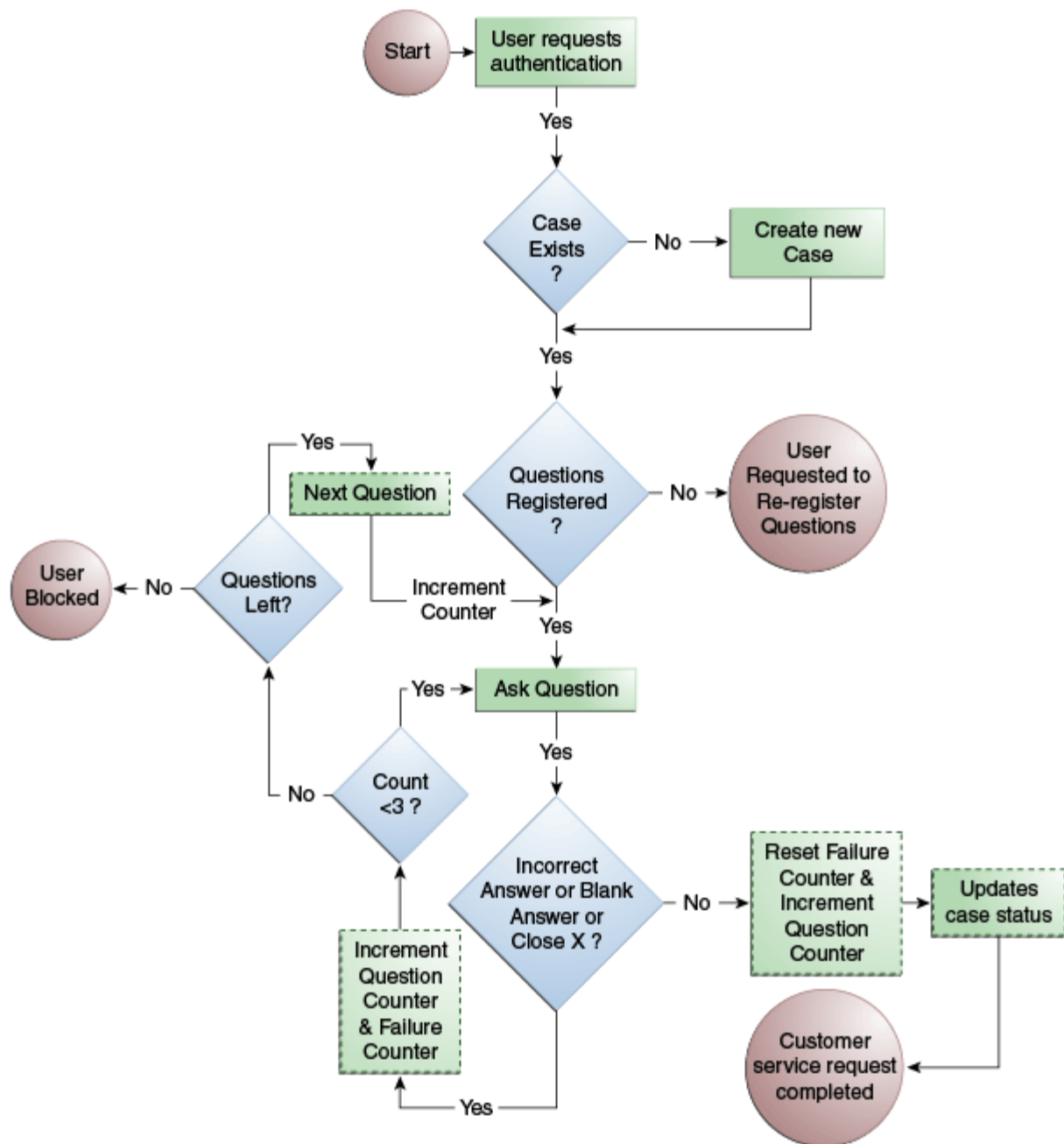
Figure 4-7 Ask Question Flow
