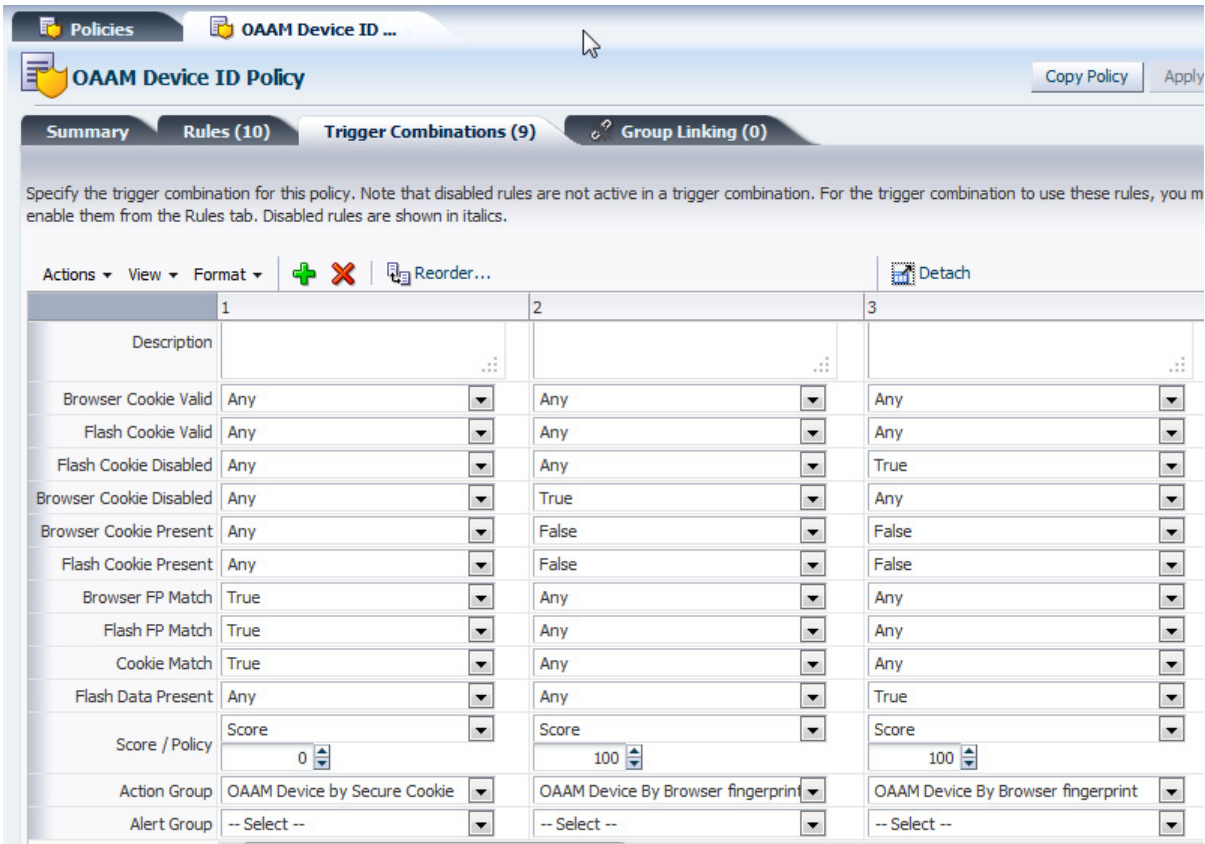
Figure E-15 Device ID Policy Trigger Combinations 1-3
