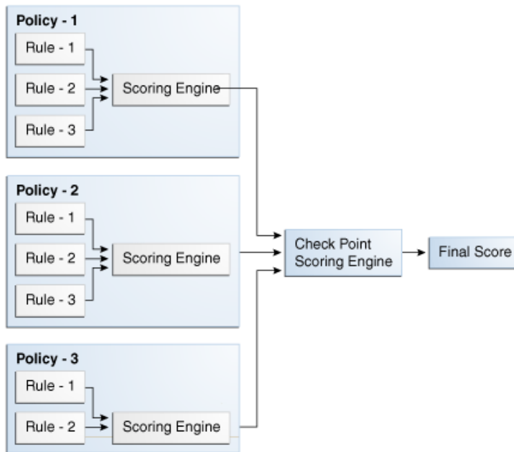
Figure 10-4 Scoring
