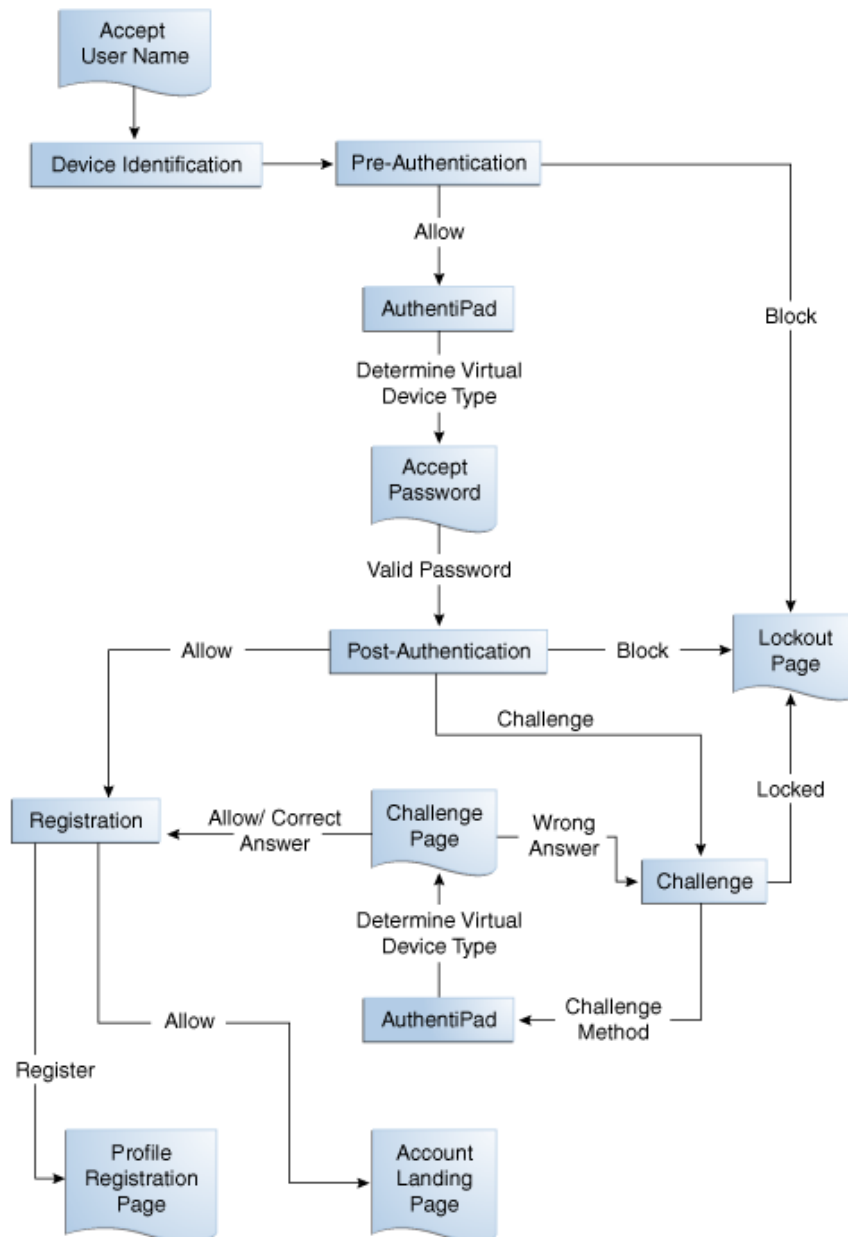
Figure 10–8 Authentication Flow
