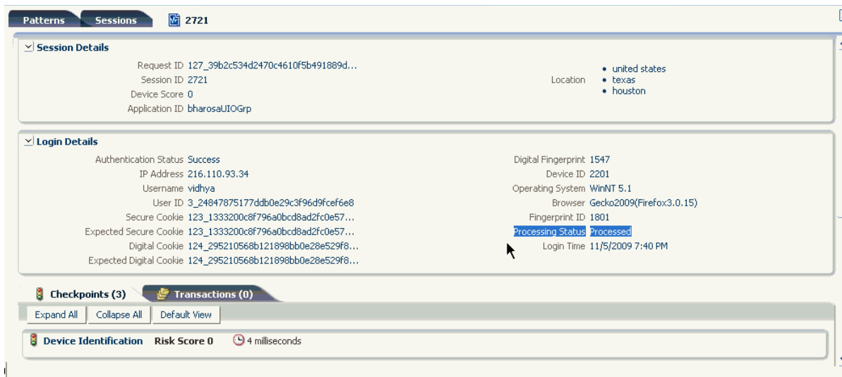
Figure 29–1 Autolearning processing
