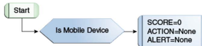
Figure 10–12 OAAM Base Device ID Flow Diagram
