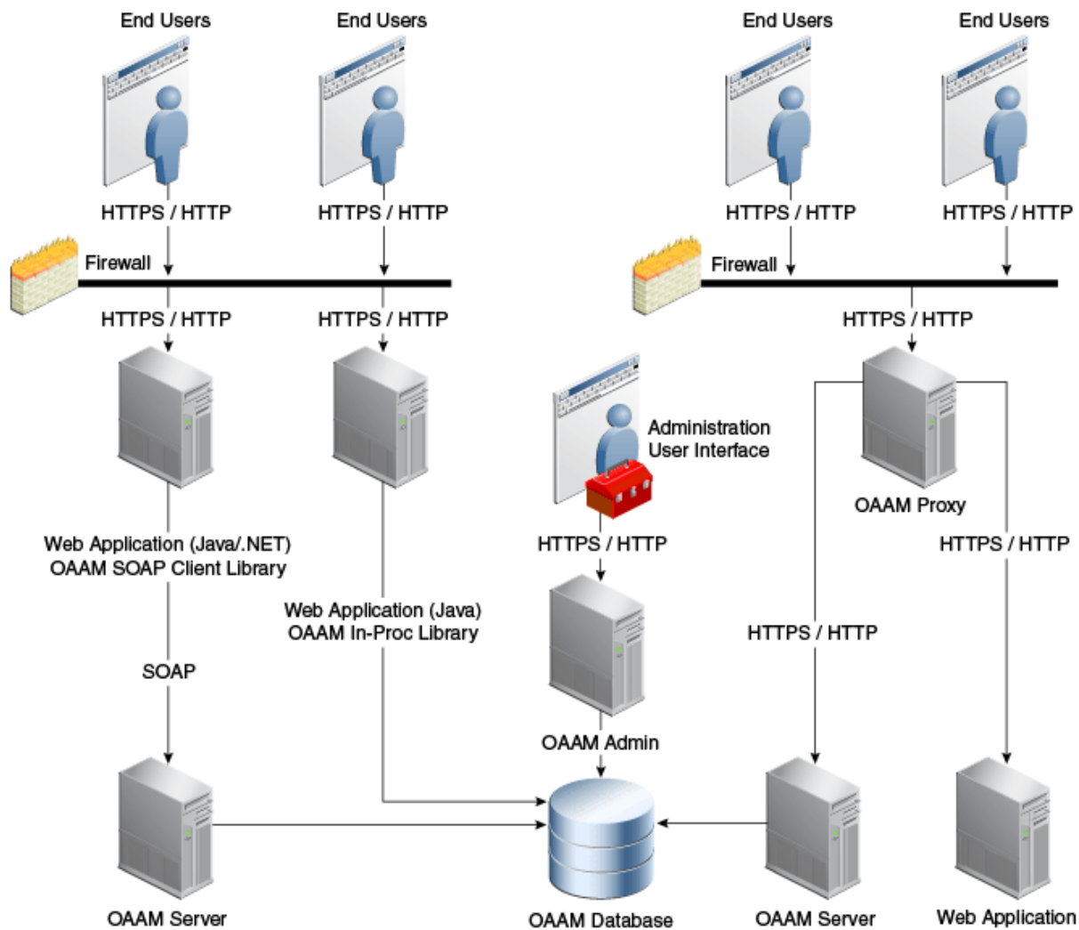
Figure 1–2 OAAM Deployment Options
