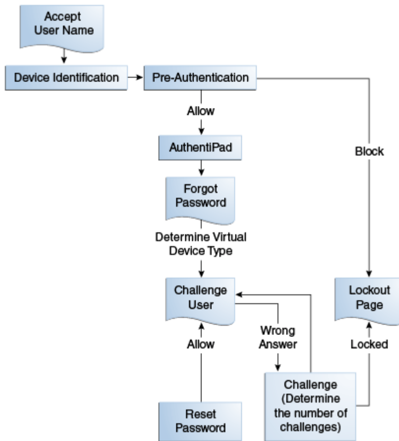
Figure 10–9 Forgot Password Flow
