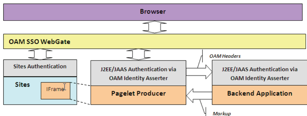
Figure 62–56 Pagelet Producer Calling the Backend Application Directly
