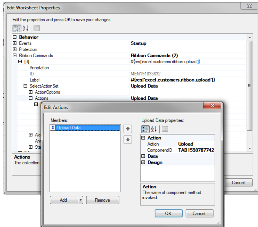
Figure 7–8 Action Set Uploading Data from an ADF Table Component
