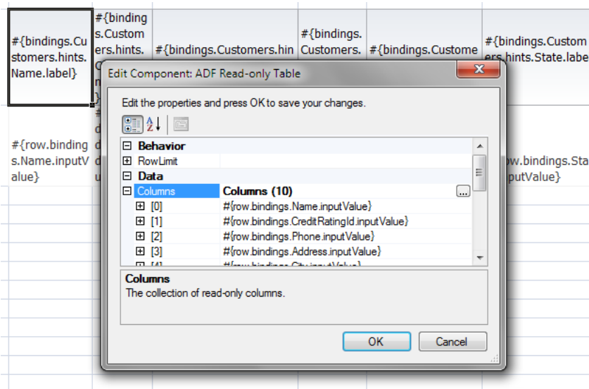
Figure 7-15 ADF Read-only Table Component at Design Time
