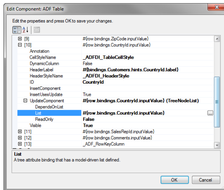
Figure 7–13 ADF Table Component Column Configured to Display a List of Values
