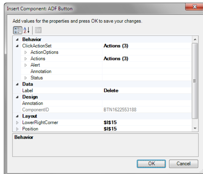
Figure 5-7 Property Inspector Window for ADF Button Component
