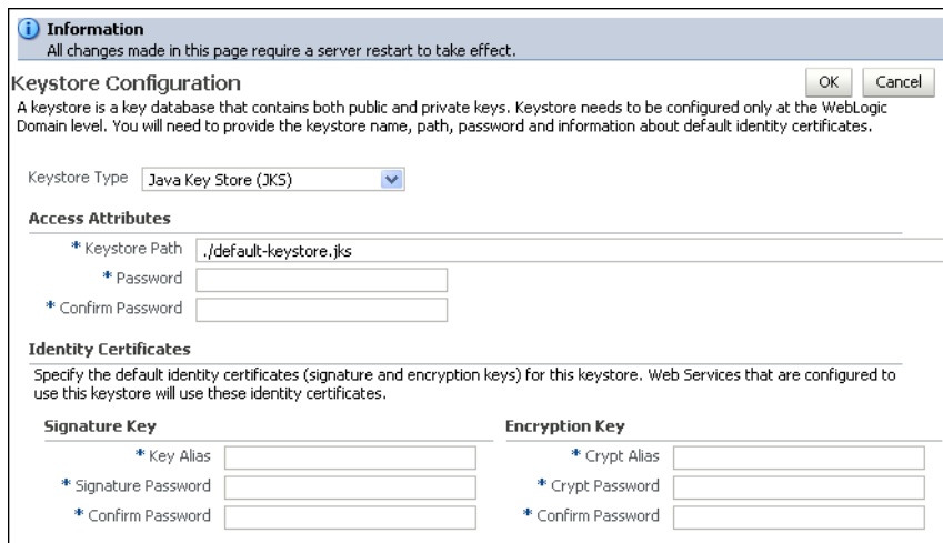
Figure 10–3 Keystore Configuration
