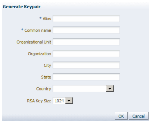
Figure 10–12 Generate Keypair
