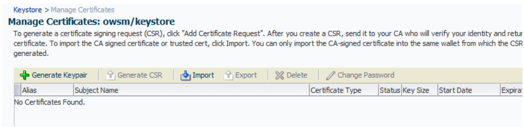
Figure 10–11 Manage Certificates
