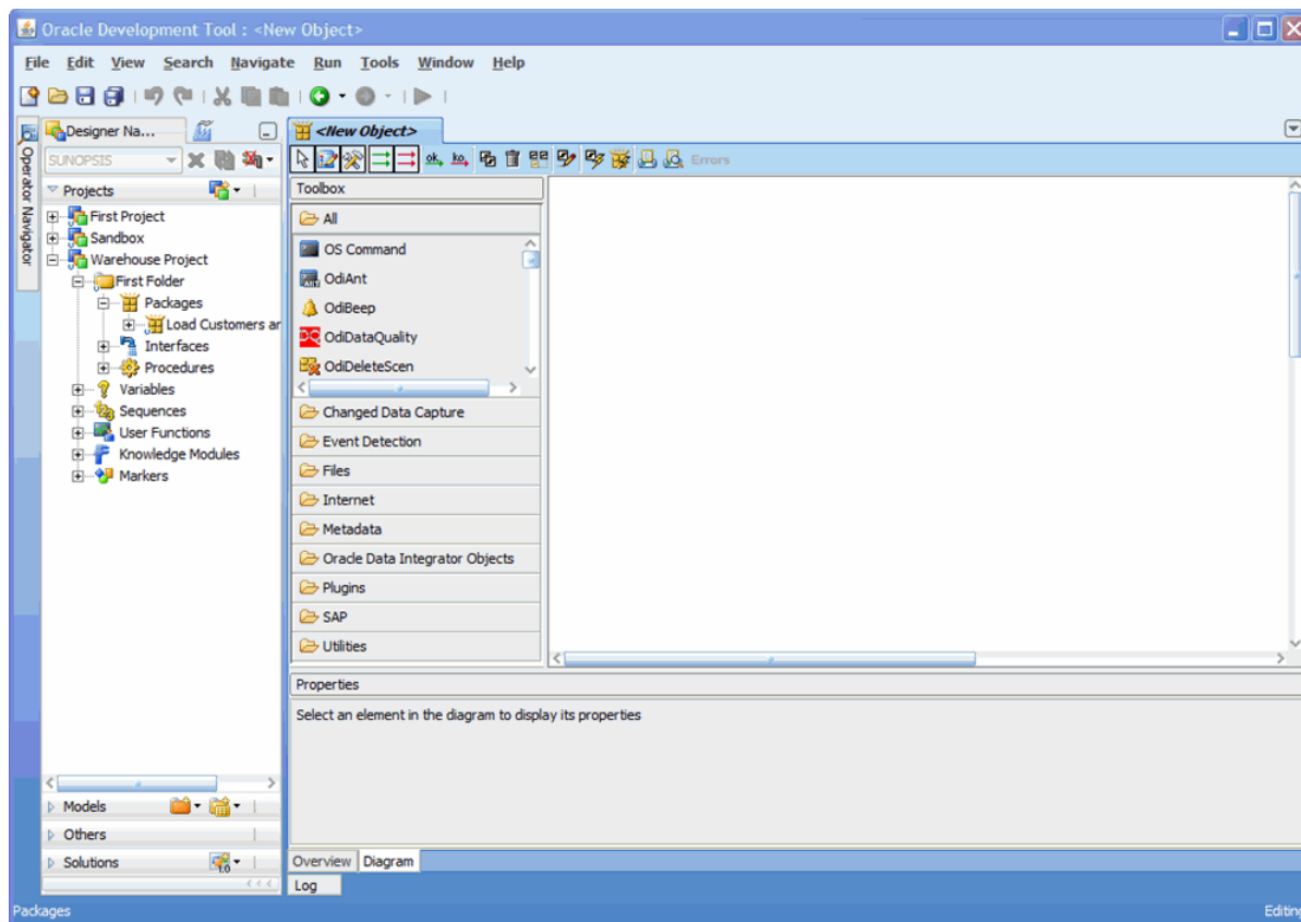
Figure 10–2 Package editor
