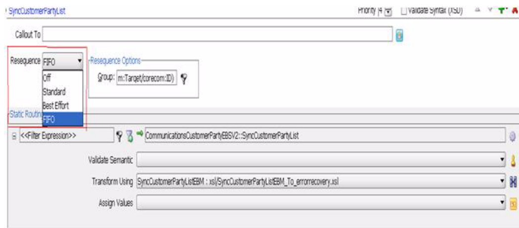
Figure 17–15 Resequence Types
