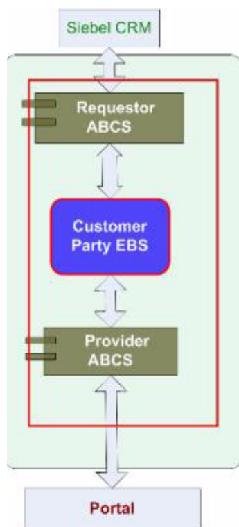
Figure 17-11 Transaction Boundary
