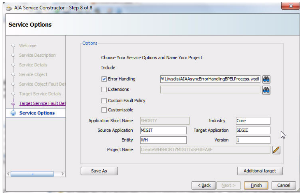
Figure 4–15 Service Options
