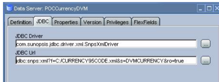
Figure 25–12 XML Used in the JDBC Description for the Data Server
