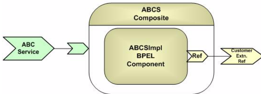
Figure 17-6 Example of Composite with One External Reference
