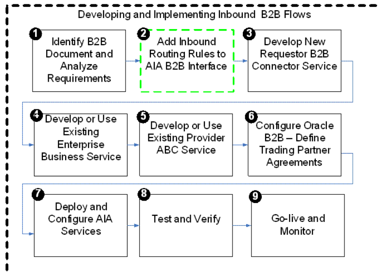
Figure 22–3 Step 2: Adding Inbound Routing Rules to an AIA B2B Interface
