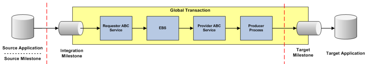
Figure 27–3 Integration Flow in Which the Receiver Target Milestone is Within the Global Transaction Space
