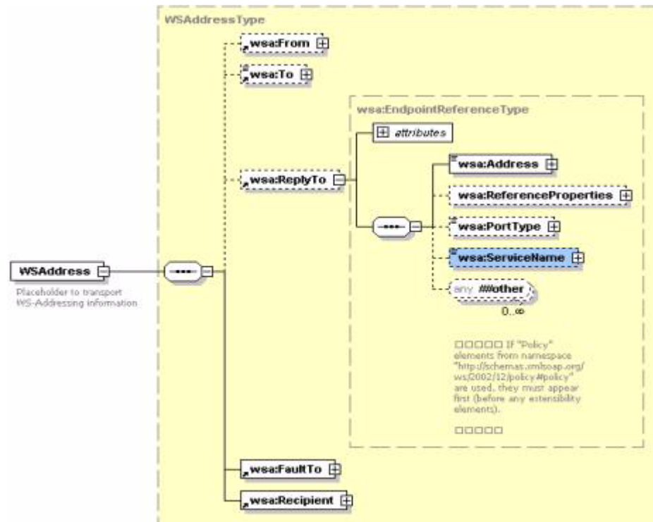
Figure 16-6 Structure of the WSAddressType
