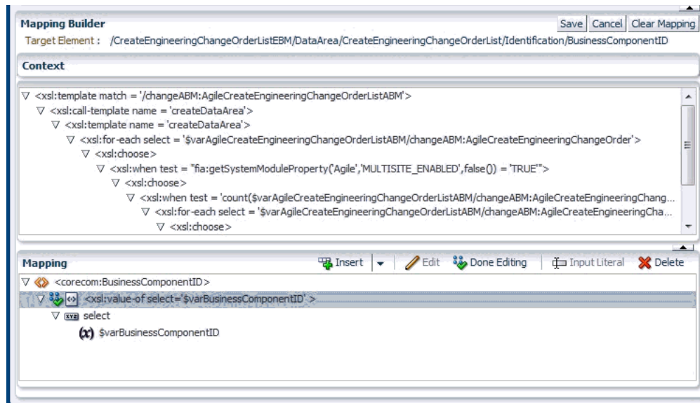
Figure 33–4 Mapping Expression Builder Screen
