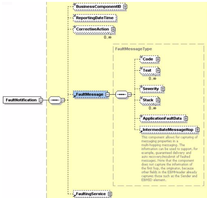
Figure 27-9 FaultNotification Element and Its Child Elements
