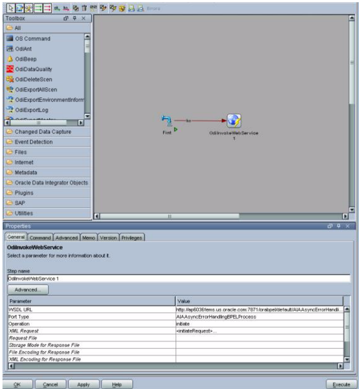
Figure 25–21 Sample Interface that Invokes AIAAsyncErrorHandlerBPELProcess When it Ends in Error
