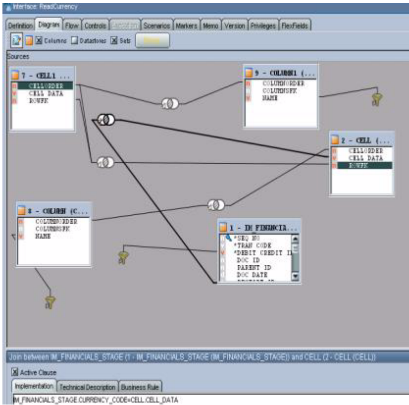
Figure 25–14 Join of IM_FINANCIALS_STAGE with the CELL Table
