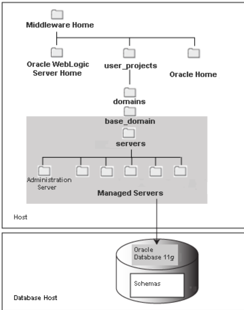
Figure 1-1 Installation Topology
