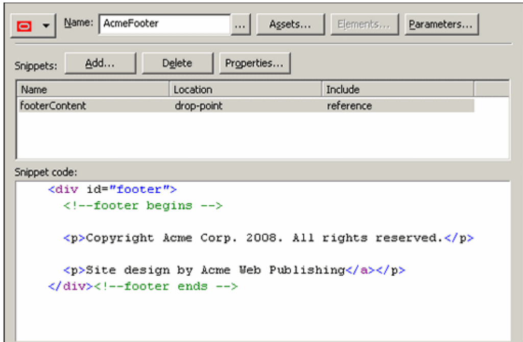
Figure A-73 Fragment Editor dialog
