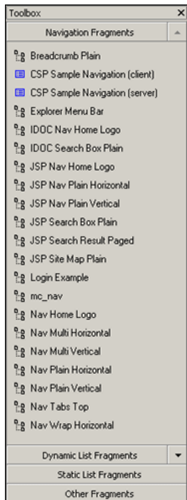
Figure 5–18 Toolbox
