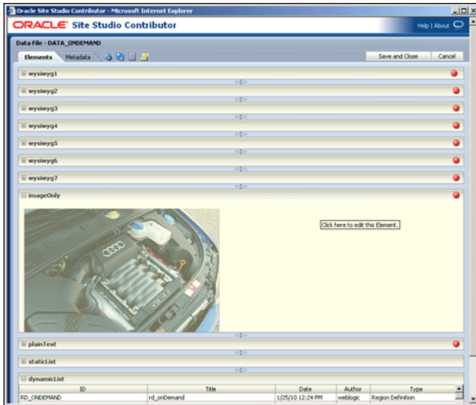
Figure 5–44 Contributor Editor
