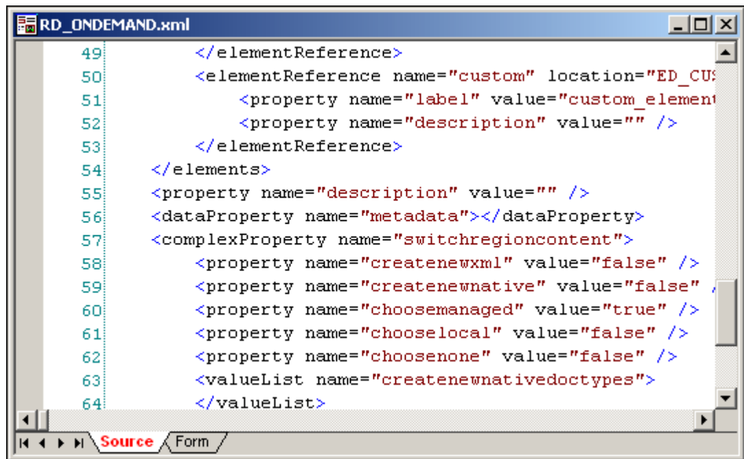
Figure 9–10 Source View
