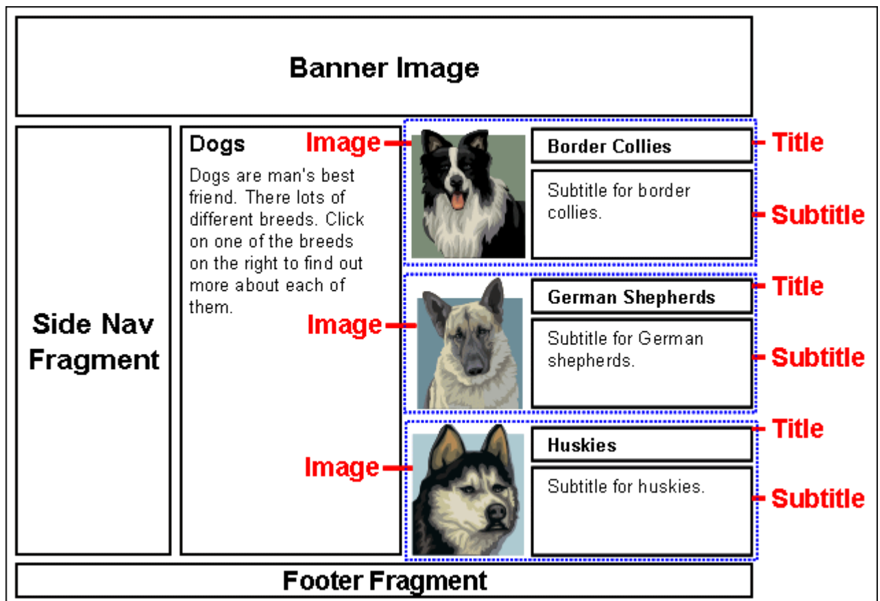
Figure 3-6 Web Page With "Teaser" Content
