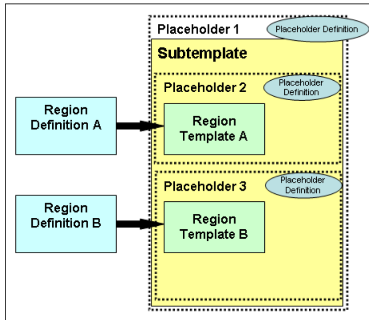
Figure 3–16 Subtemplate in a Placeholder
