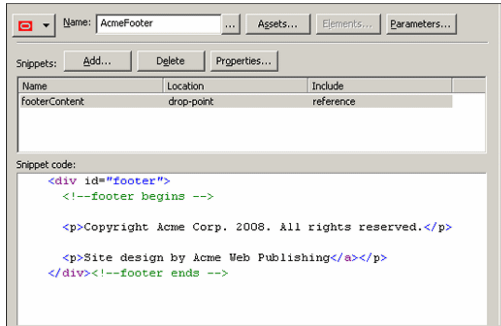
Figure 5–34 Fragment Editor
