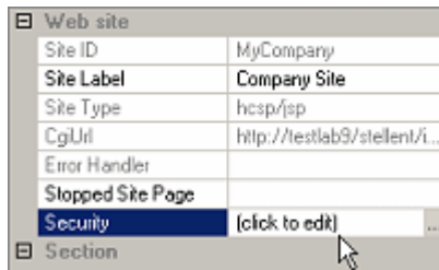
Figure 12–9 Security property
