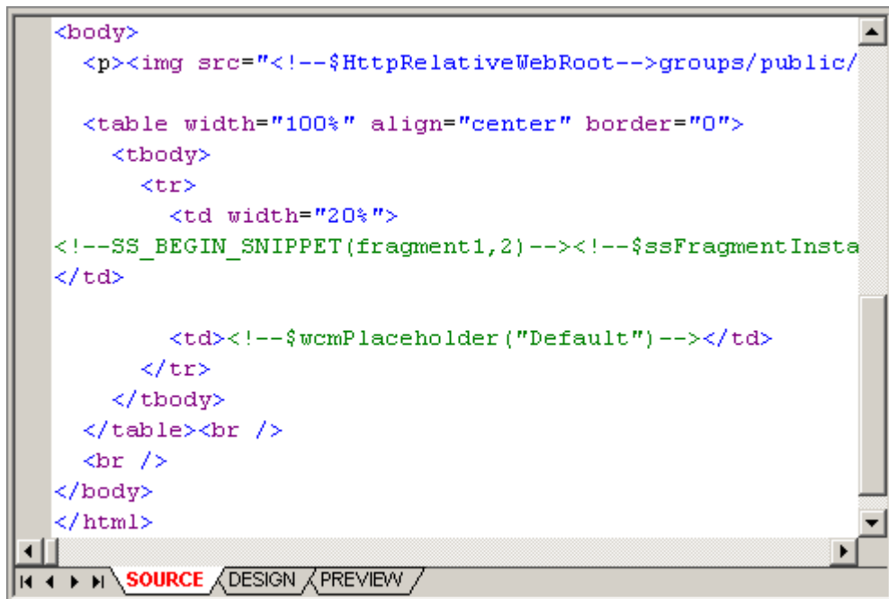
Figure 8–11 Source View
