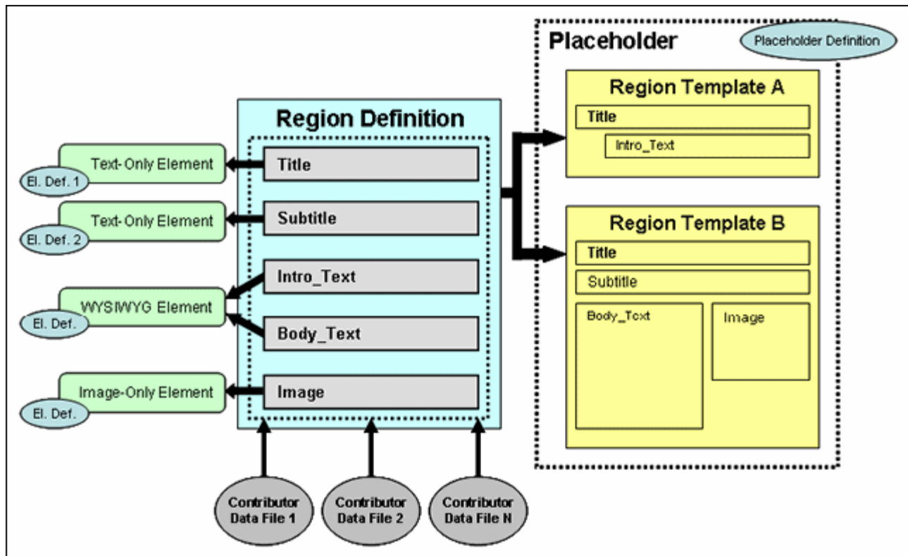
Figure 3–5 Example of Site Object Hierarchy
