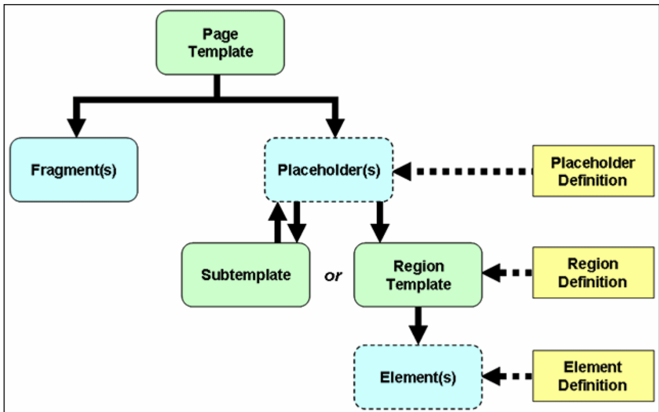
Figure 3–4 Object Hierarchy of Web Sites
