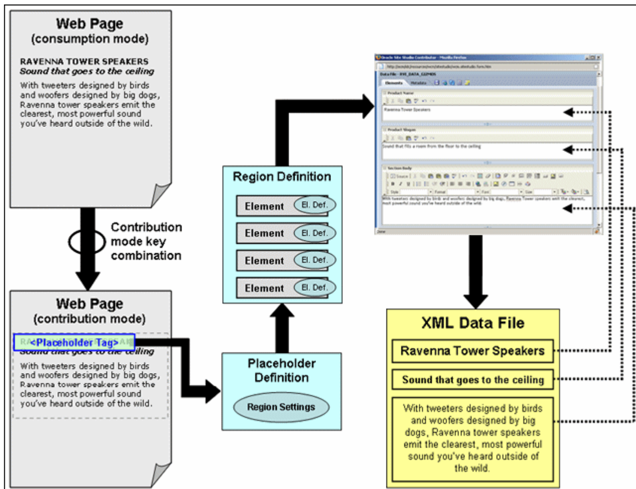
Figure 3–3 Contribution Model for Site Studio Web Sites
