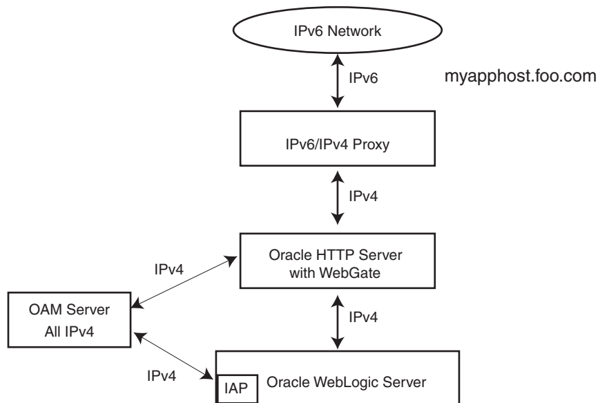
Figure 15–2 Simple Authentication with the IPv6/IPv4 Proxy
