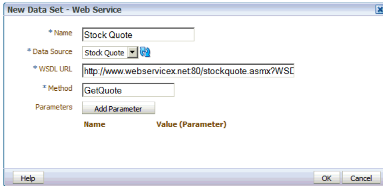
Figure 2–22 Creating a Data Set Using a Simple Web Service Connection
