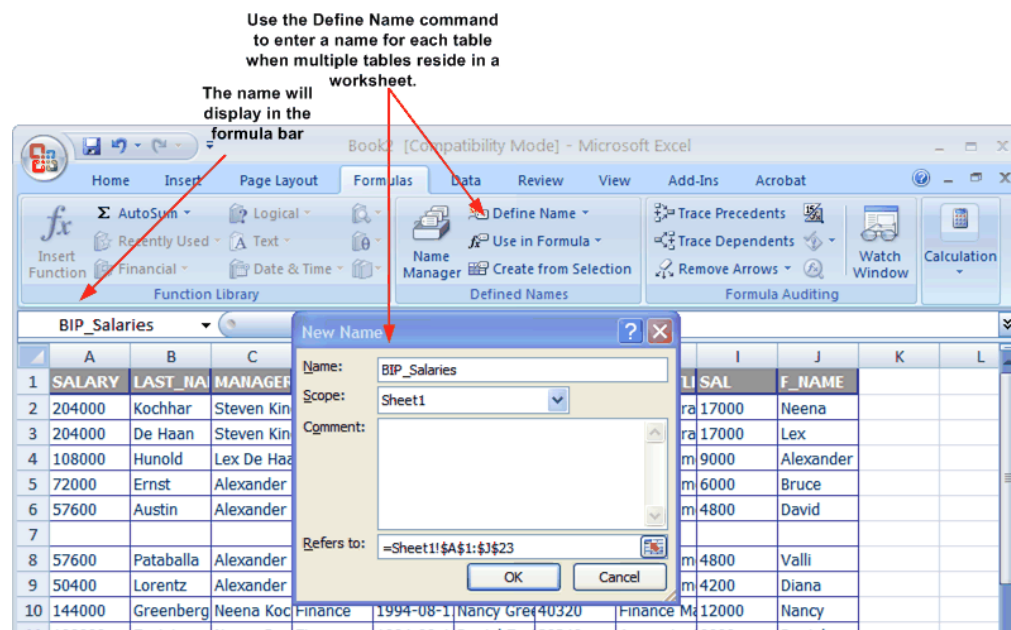
Figure 2–35 Using the Define Name Command in Microsoft Excel
