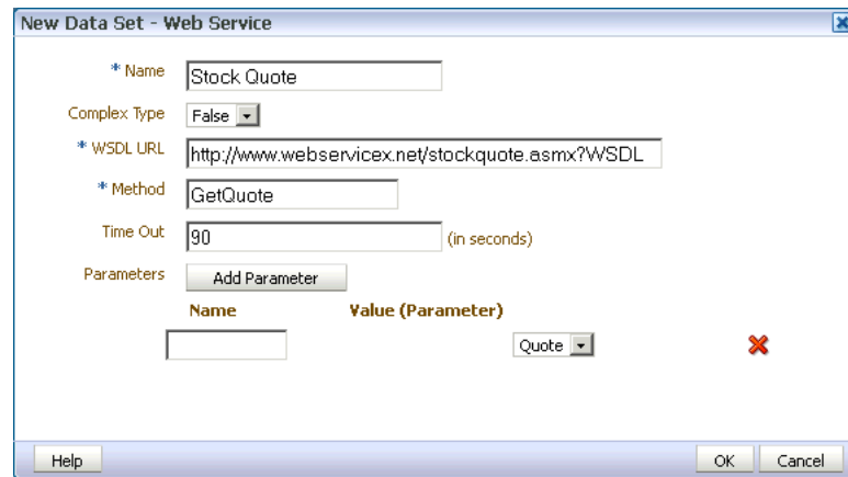
Figure 2–28 Adding the Parameter to Web Service Data Set
