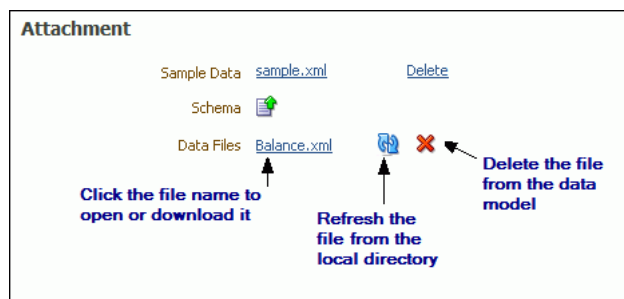
Figure 2–34 Attachments Region of the Properties Pane
