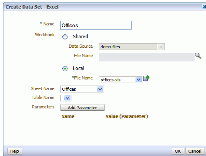
Figure 2–37 Creating a Data Set from an Excel Spreadsheet
