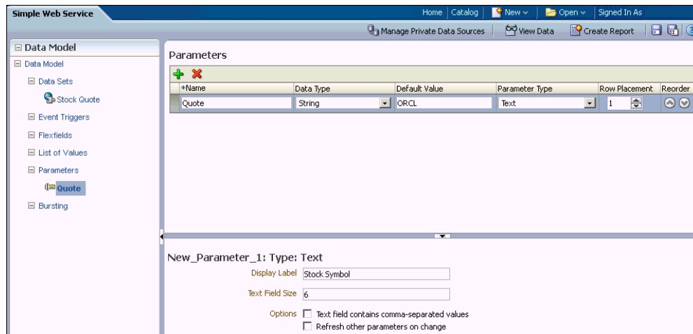
Figure 2–27 Creating the Parameter
