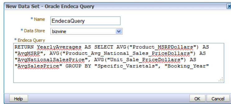
Figure 2–44 Sample Oracle Endeca Query
