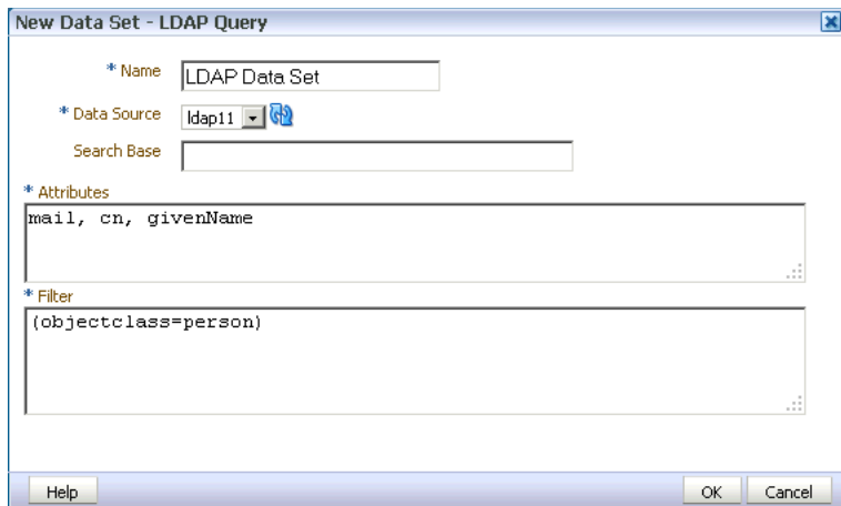
Figure 2–31 Sample LDAP Query
