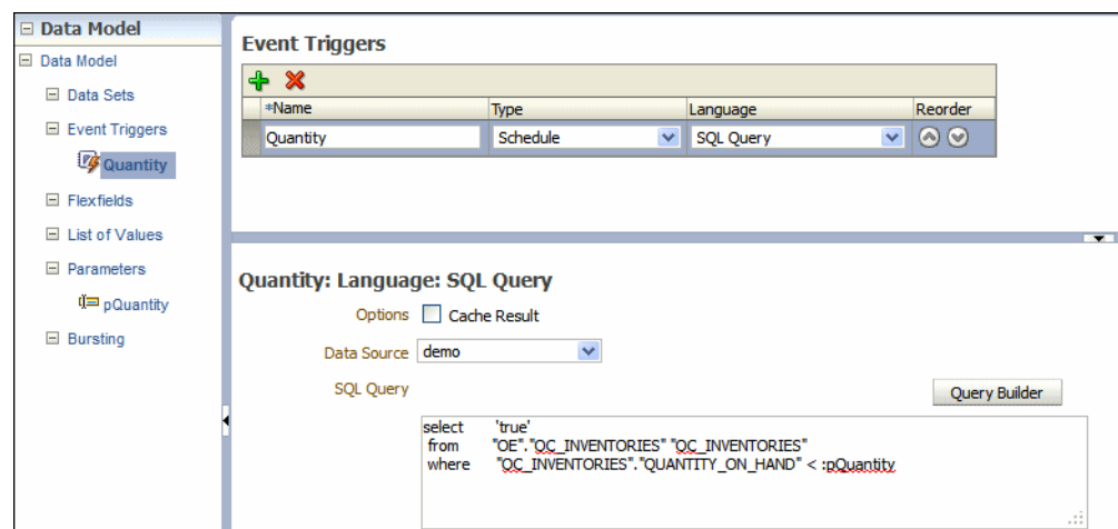
Figure 5–2 Schedule Trigger
