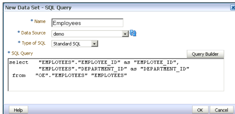
Figure 2–45 Sample Query
