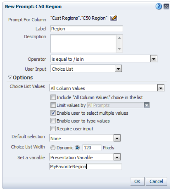
Figure 2–15 Region Prompt
