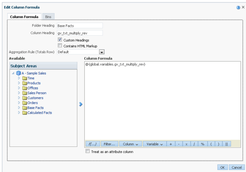
Figure 2–14 Example of a New Global Variable in the Edit Column Formula Dialog
