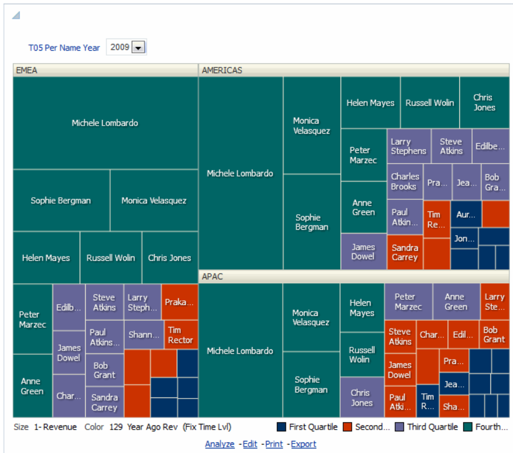
Figure 3–22 Example of a Treemap View on a Dashboard
