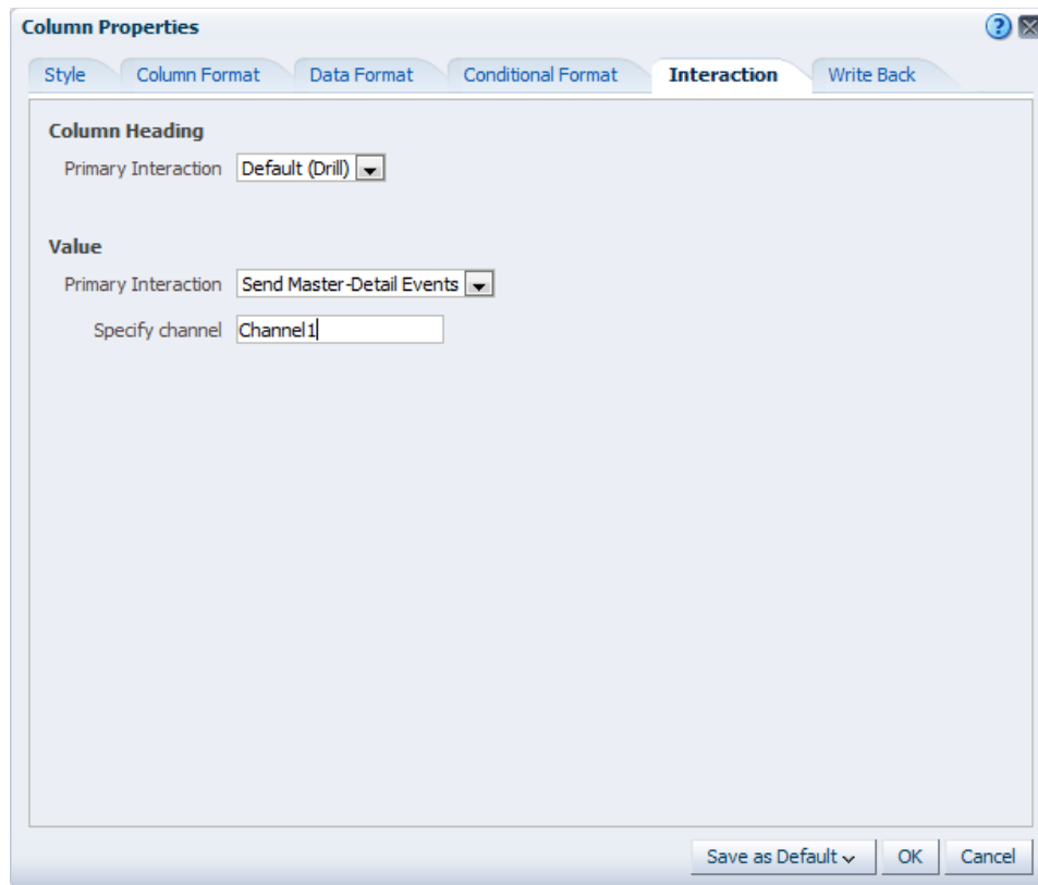
Figure 3–33 Example of Defining a Master View
