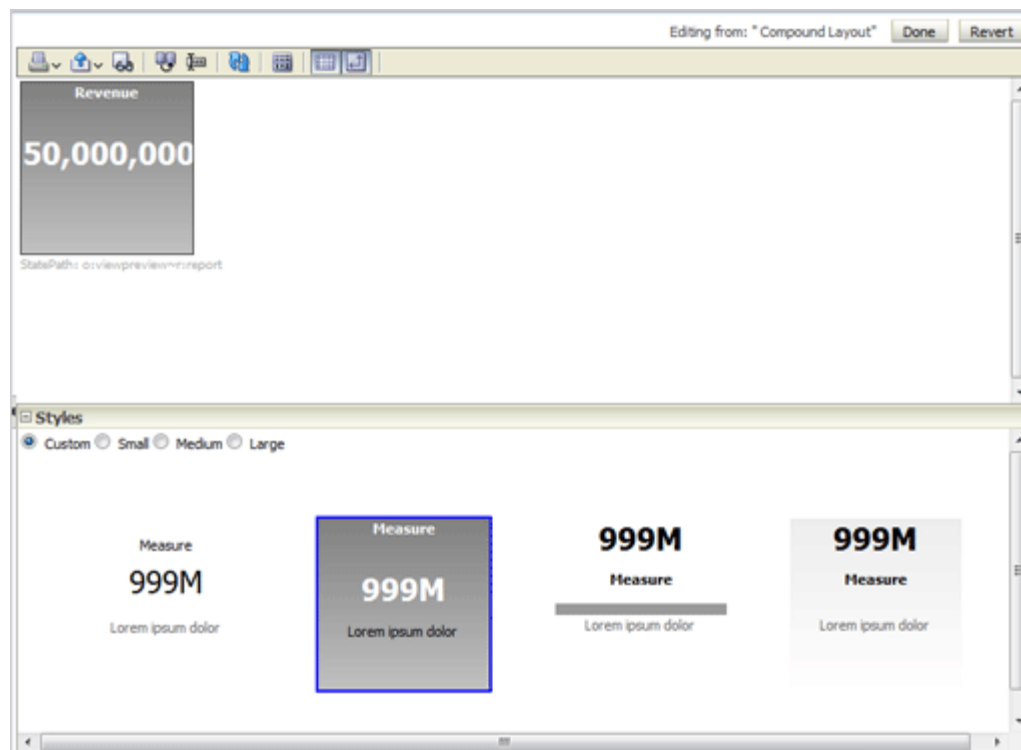
Figure 3–21 Styles Pane
