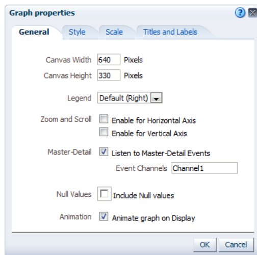
Figure 3–34 Setting up to Listen to Master -Detail Events
