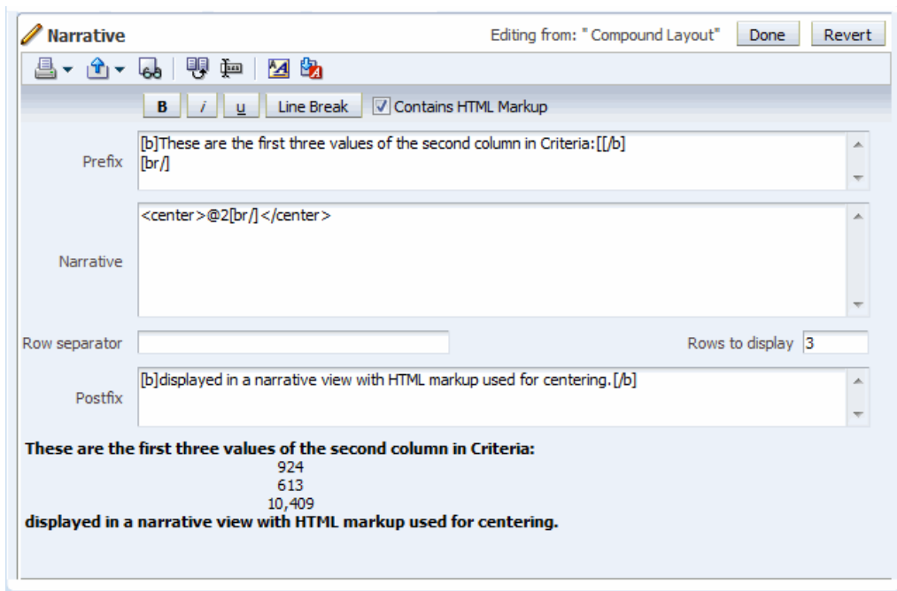
Figure 3–16 Sample of the Narrative Editor
