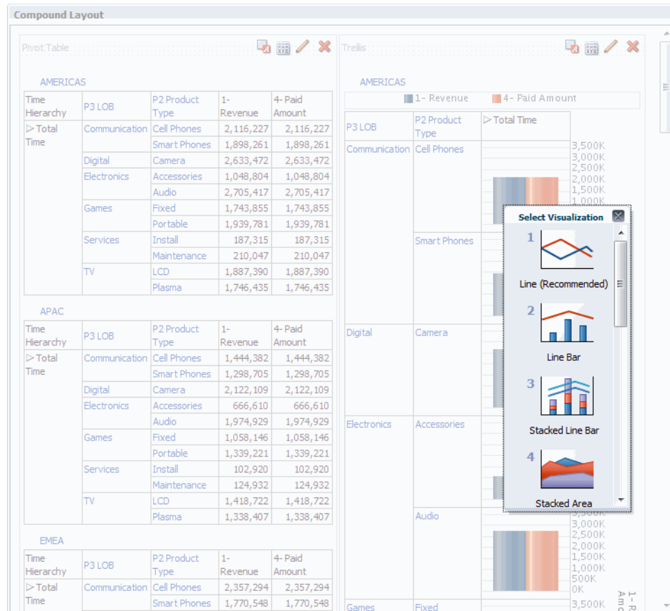
Figure 3–2 Recommended Visualizations in Select Visualization List
