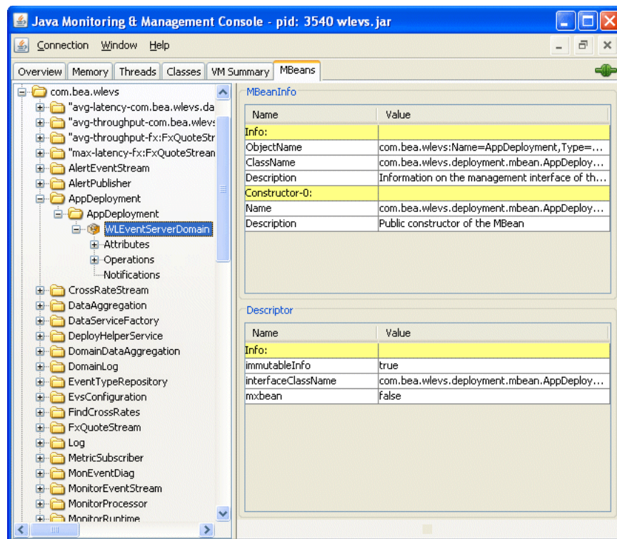
Figure 12-6 JConsole Browser
