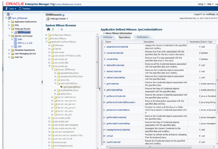
Figure O–1 getPortableCredential Operation
