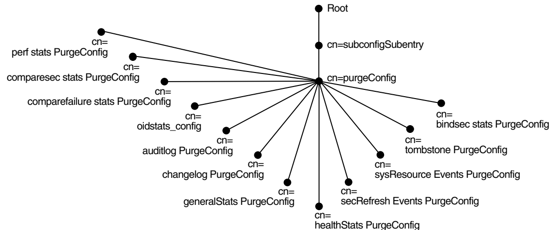
Figure 36–2 Garbage Collection Entries in the DIT
