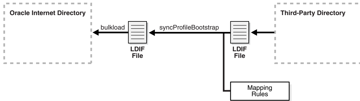
Figure 37-4 Using syncProfileBootstrap, bulkload, and LDIF Files
