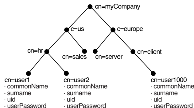
Figure 40-1 A Sample Naming Context
