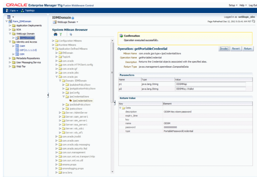
Figure O–2 getPortableCredential Operation
