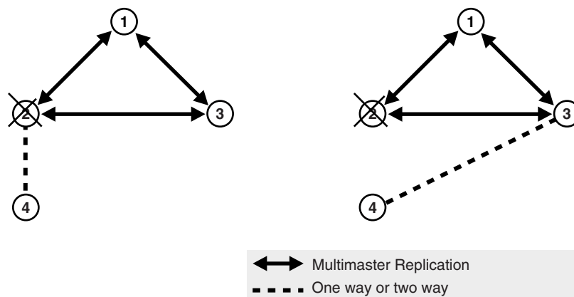
Figure 41-3 Old and New Suppliers in the Same Advanced Replication Group
