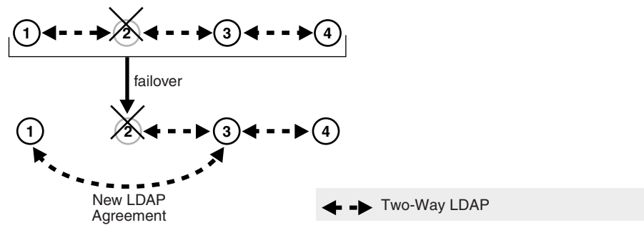
Figure 41-5 Compare and Reconcile All Connected Replicas
