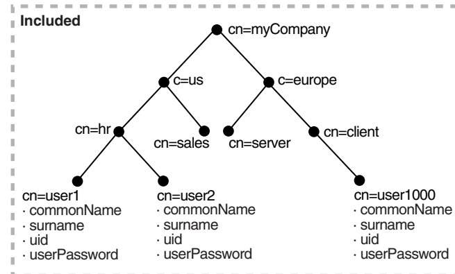
Figure 40-2 Naming Context Object #1
