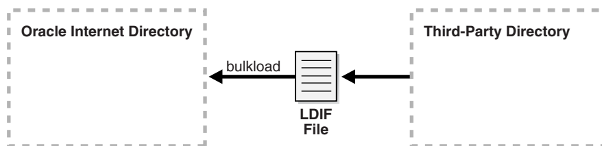
Figure 37-1 Using an LDIF File and bulkload
