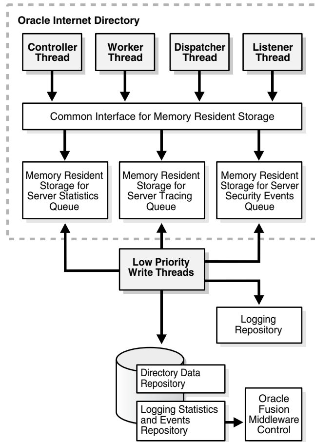
Figure 25–1 Architecture of Oracle Internet Directory Server Manageability
