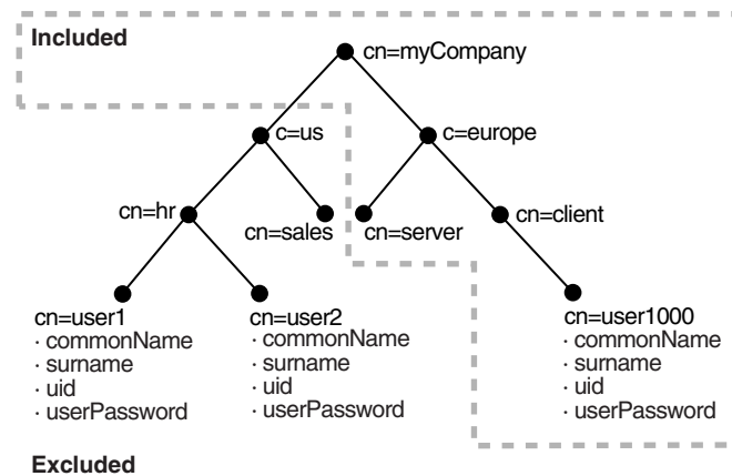
Figure 40–7 Result of Combining Naming Context Objects #3 and #4
