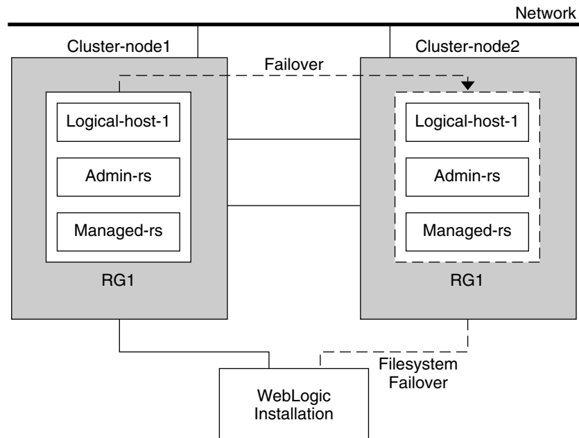
FIGURE 1–2 Oracle Solaris Cluster HA for WebLogic Server File System Failover Configuration
