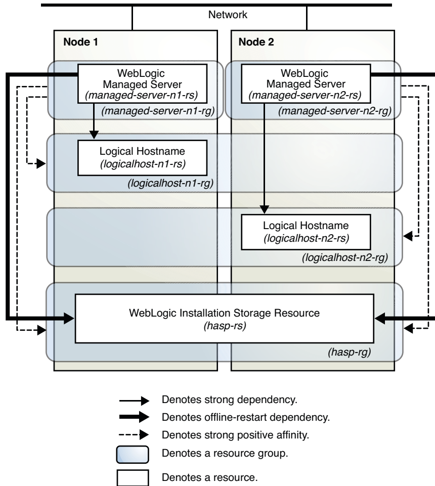
FIGURE 1-4 Oracle WebLogic Server Configured as a Multi-Instance Application With Single-Node Resource Groups
