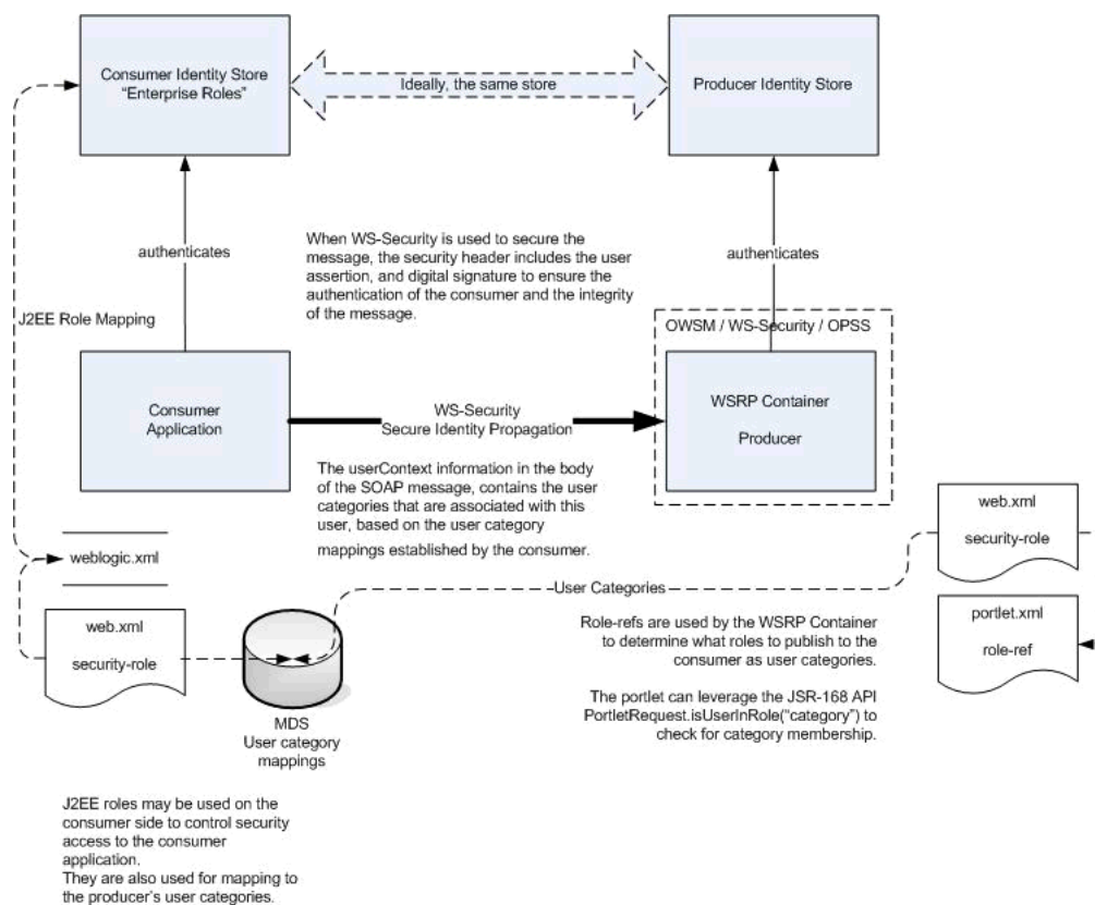
Figure 68–18 WSRP Portlet Security Architecture
