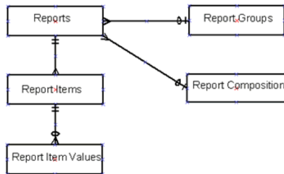
Figure G-4 Report Metadata Entities
