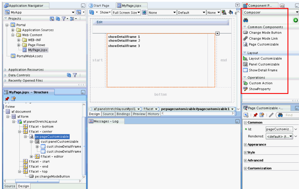
Figure 17–59 Composer Tag Library in the Component Palette
