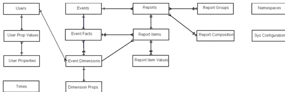
Figure G-1 Analytics Database Model
