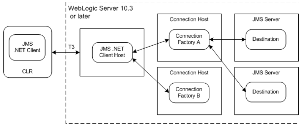
Figure 1–1 JMS .NET Client Architecture
