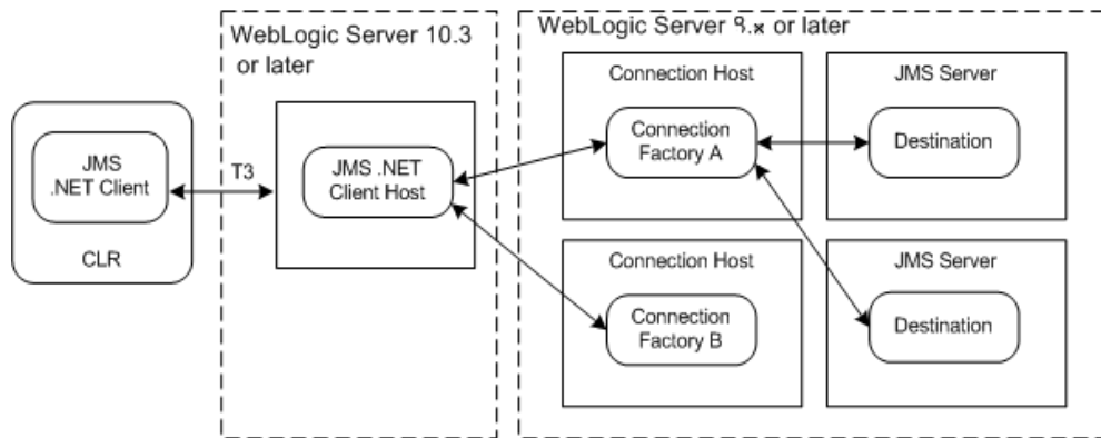
Figure 1–2 JMS .NET Client Interoperability
