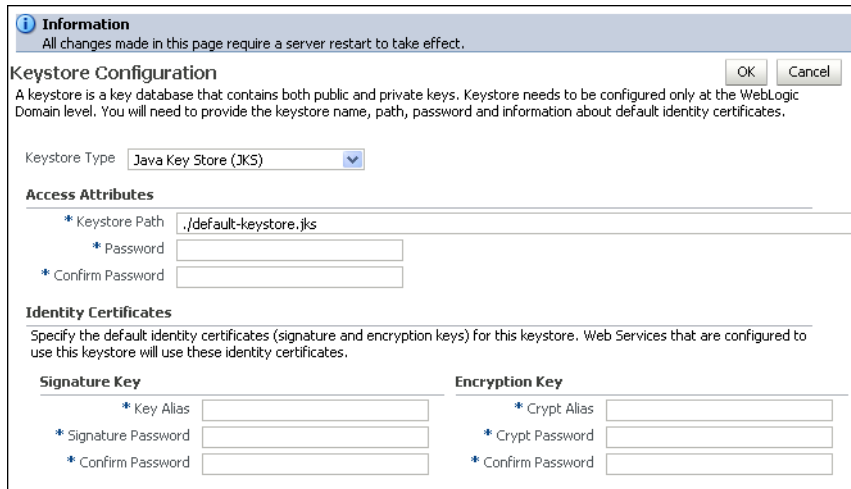
Figure 10–3 Keystore Configuration
