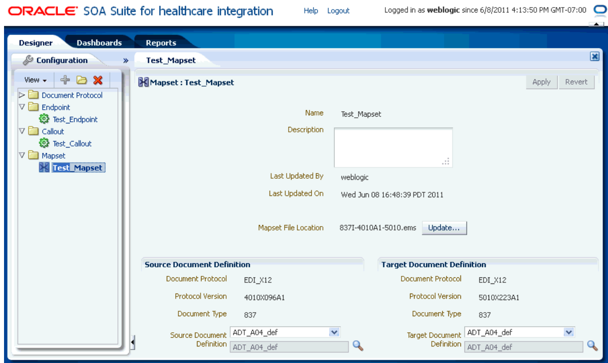
Figure 1–7 Sample Mapset
