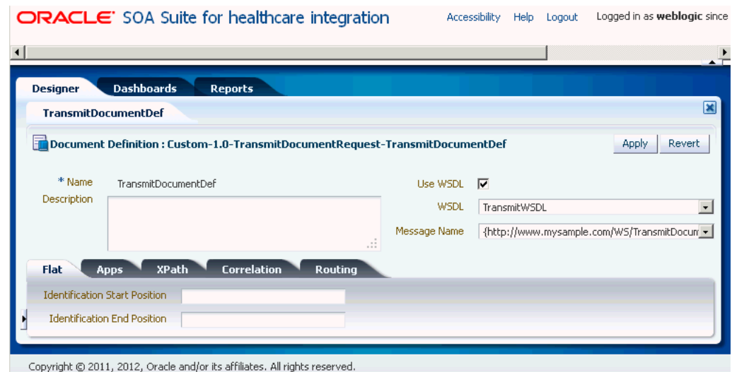
Figure 15–2 Creating Documents
