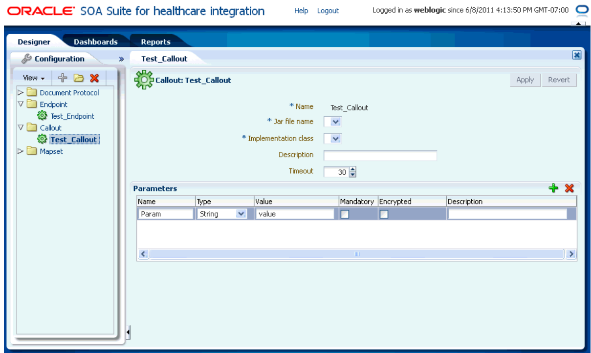
Figure 1–6 Sample Callout
