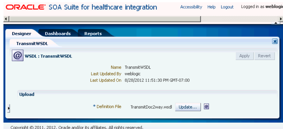
Figure 15–1 Uploaded WSDL
