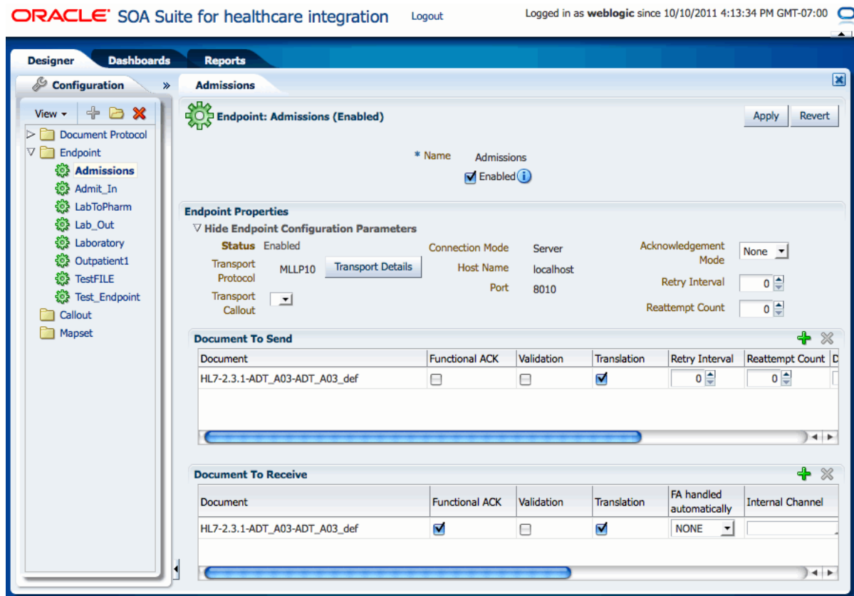
Figure 1–5 Sample Endpoint
