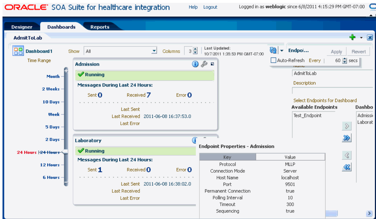
Figure 1–14 Sample Dashboard
