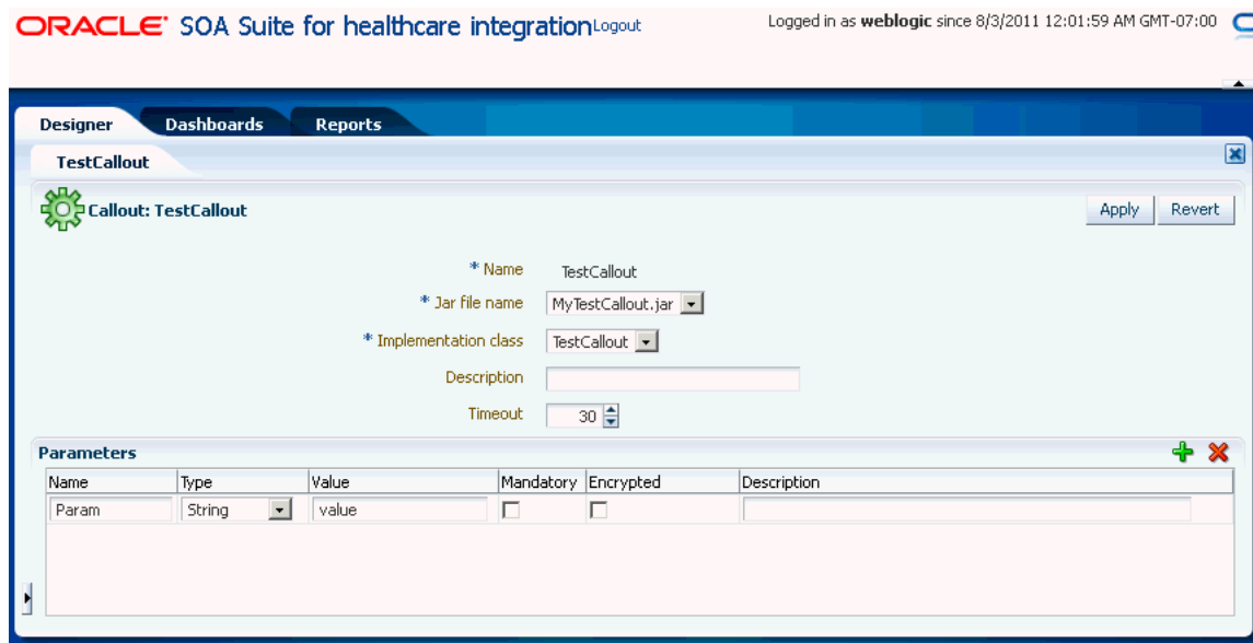
Figure 5–4 Configuring Callouts
