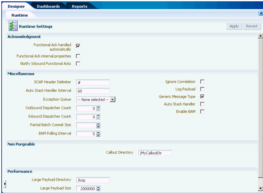
Figure 13–1 Runtime Settings
