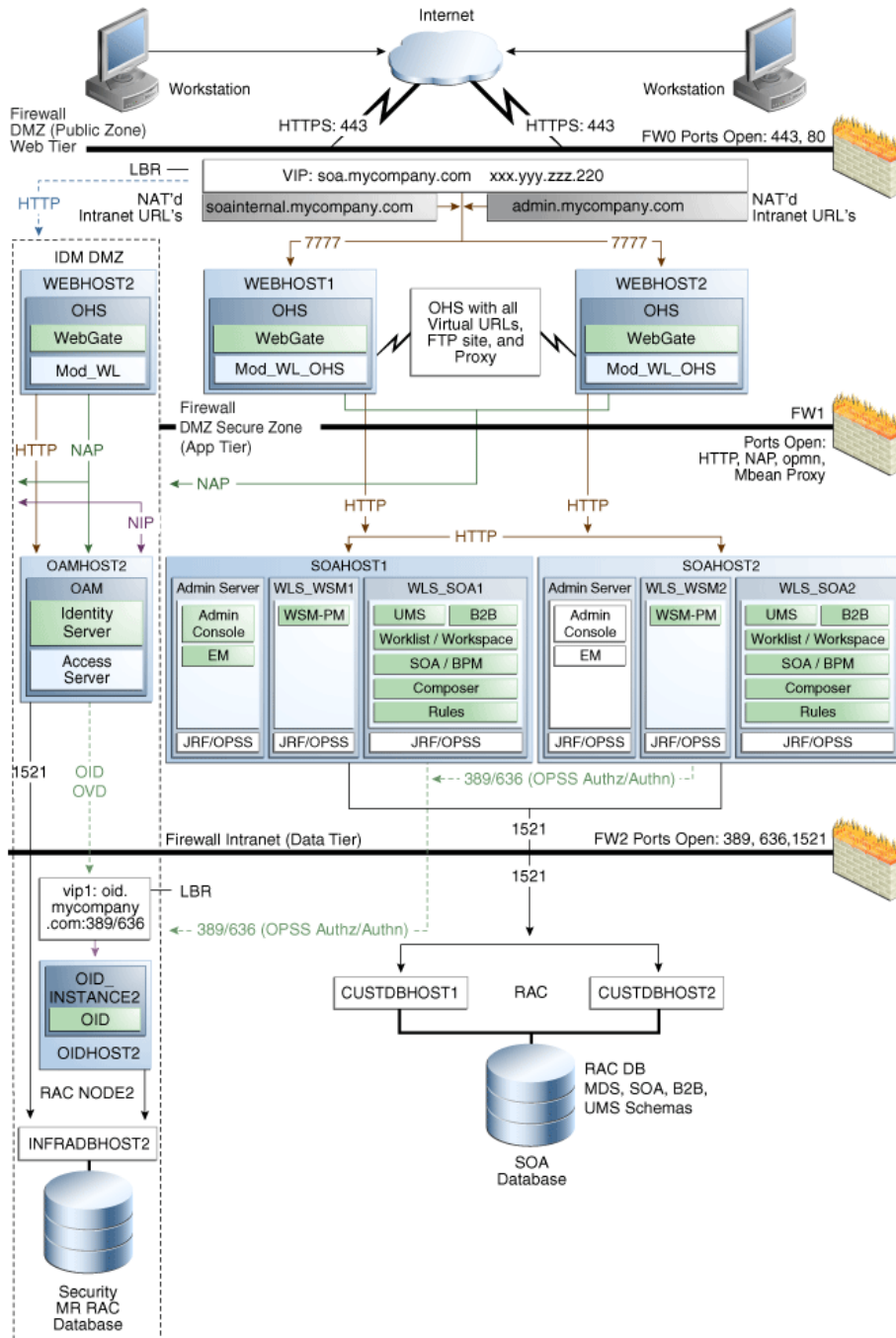
Figure 4-3 SOA Topology with Oracle Access Manager and BPM
