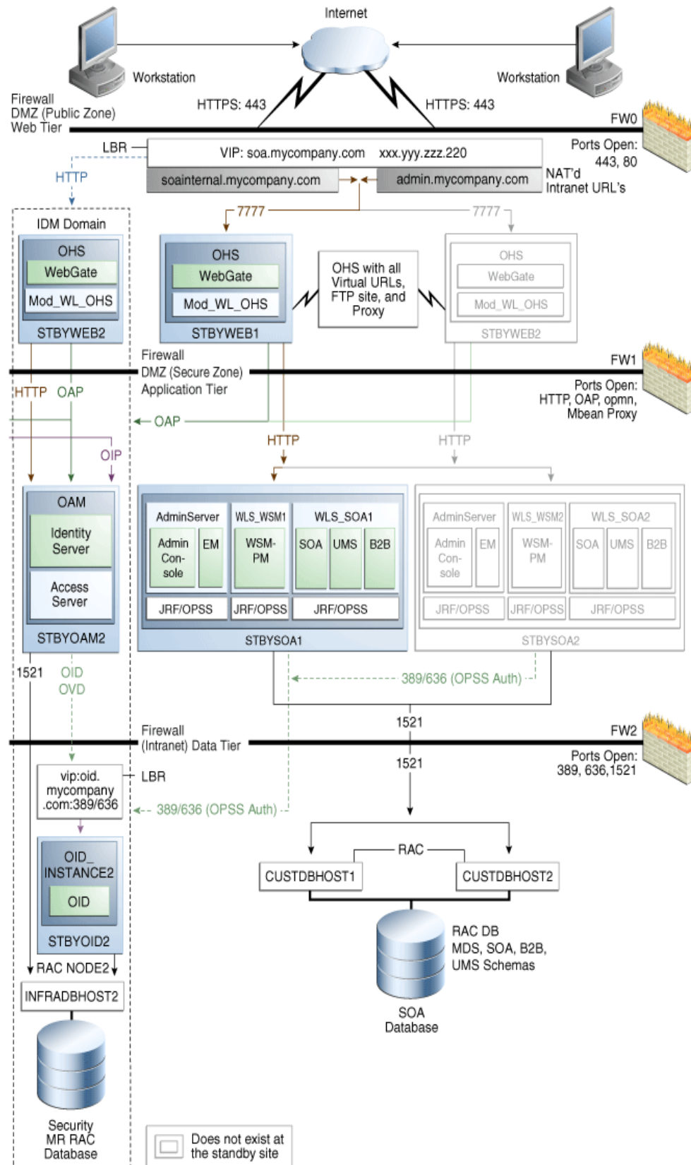
Figure 4-15 An Asymmetric Standby Site with Fewer Hosts and Instances
