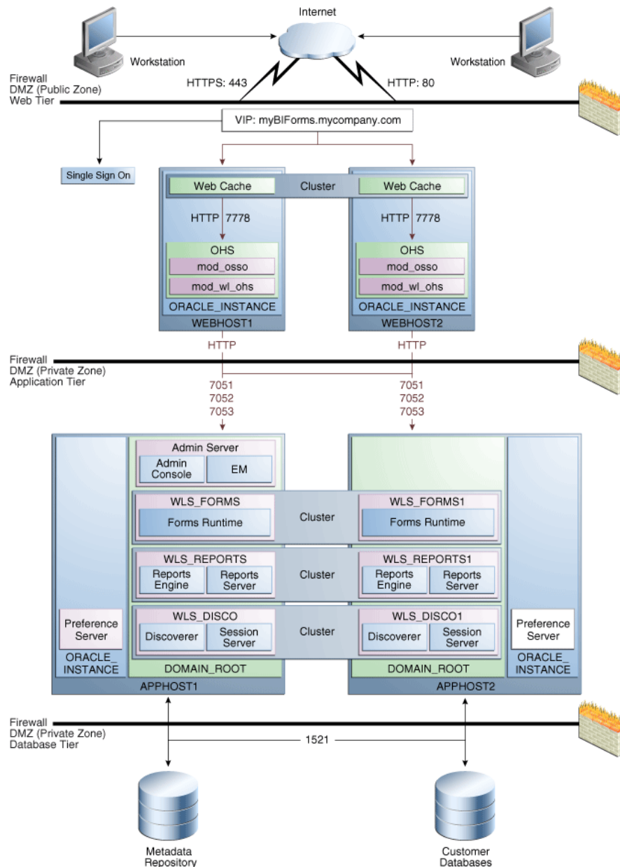
Figure 4–10 Oracle Forms, Reports, and Discoverer Topology
