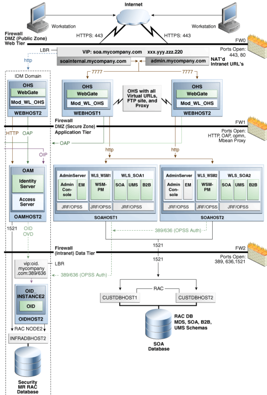
Figure 4-2 Oracle SOA Topology with Oracle Access Manager
