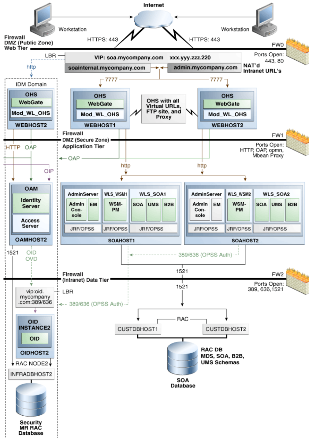
Figure 3–1 Deployment Used at Production and Standby Sites for Oracle Fusion Middleware Disaster Recovery
