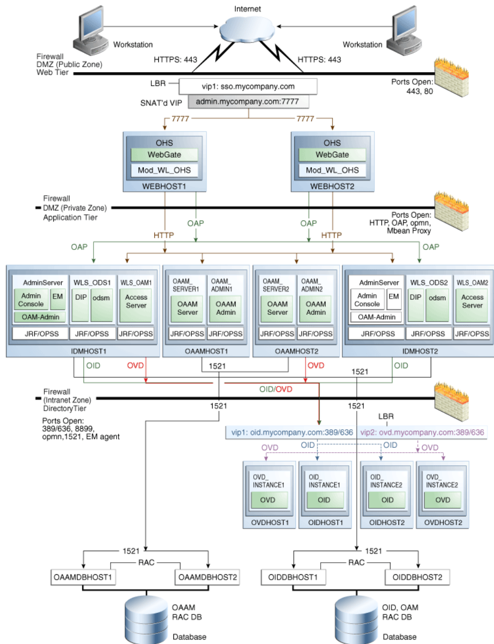
Figure 4–8 Oracle Identity Management Topology with Oracle Adaptive Access Manager
