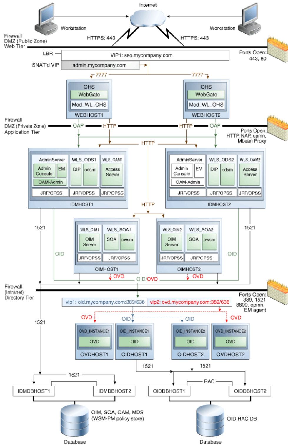
Figure 4-7 Oracle Identity Management Topology with Oracle Access Manager and Oracle Identity Manager
