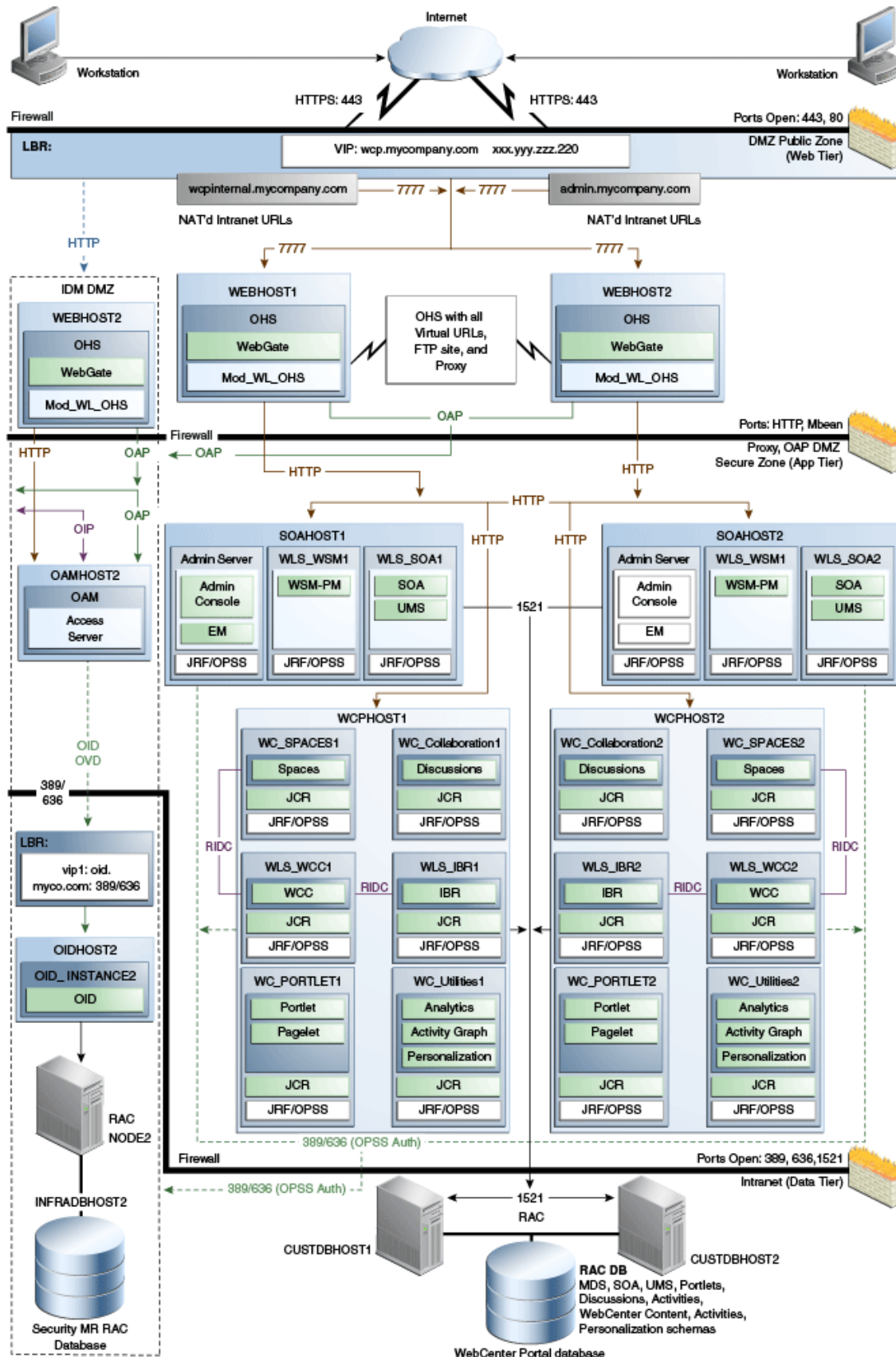
Figure 4-4 Oracle WebCenter Portal Topology with Oracle Access Manager
