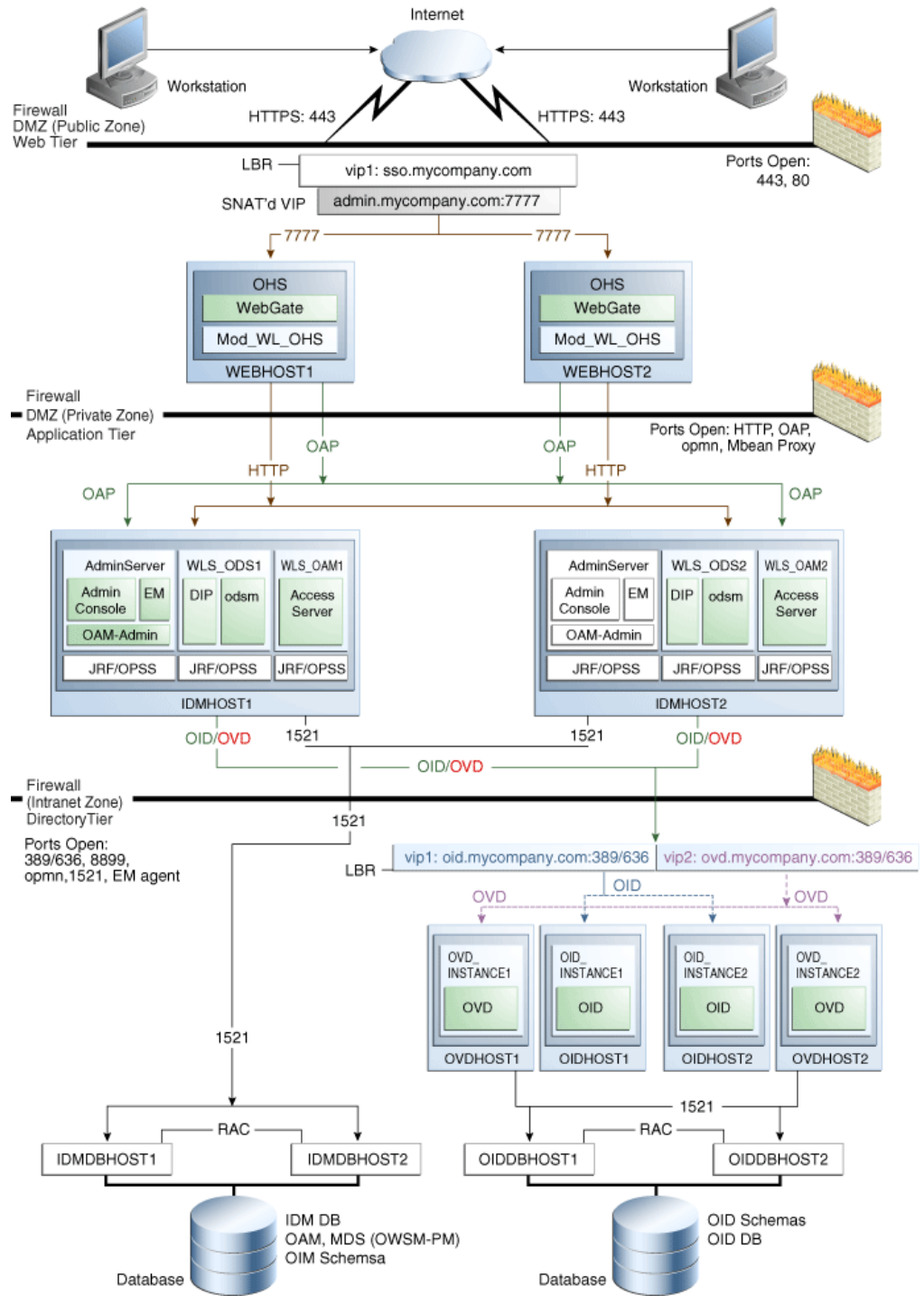
Figure 4-6 Oracle Identity Management Topology with Oracle Access Manager
