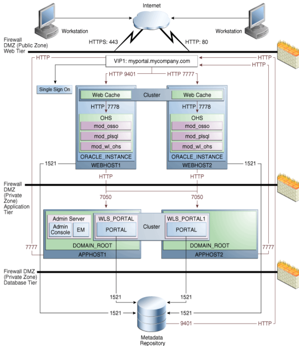
Figure 4–9 Oracle Portal Topology
