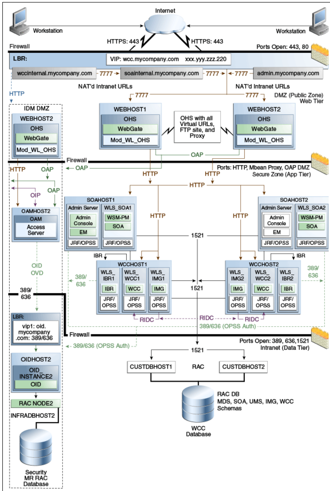
Figure 4-12 Reference Topology for Oracle WebCenter Content Enterprise Deployment
