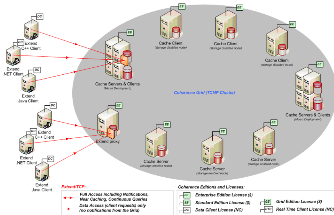
Figure 1–1 Oracle Coherence Standard or Enterprise Edition Deployment
