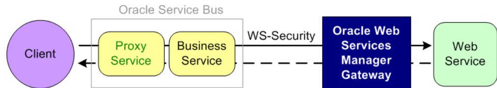
Figure 50–4 Message Protection With an Oracle Web Services Manager Gateway
