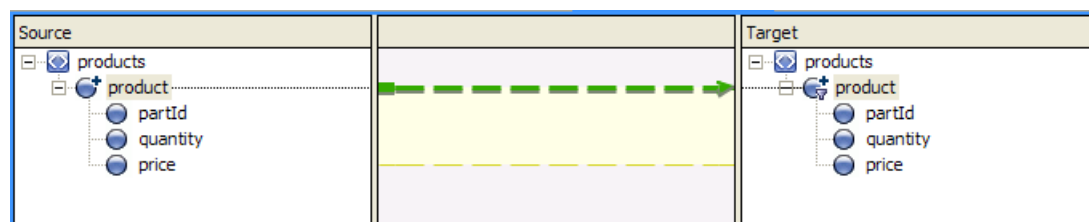
Figure 6–5 Repeating-Group-to-Repeating-Group Link
