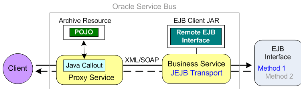
Figure 29–2 A Non-EJB Client Invokes an EJB
