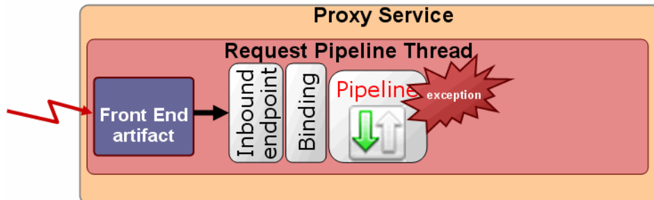
Figure 39–2 Error Case 1
