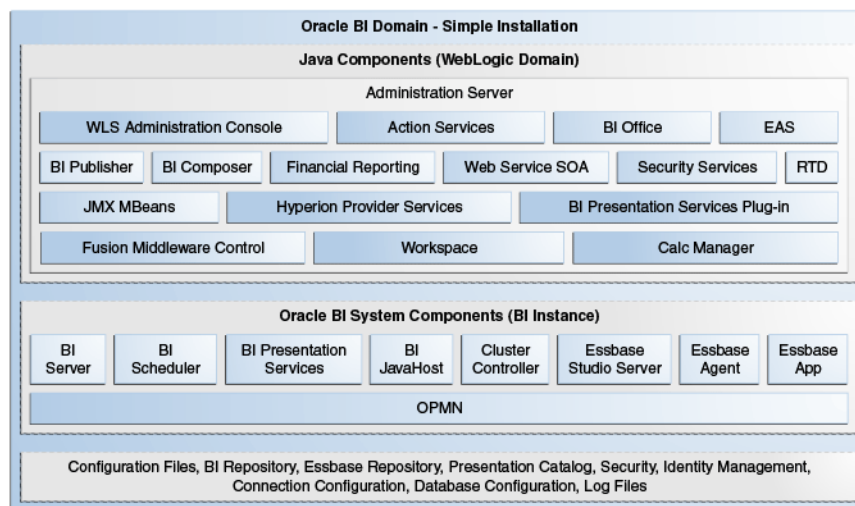
Figure 1–2 System Logical Architecture for Simple Install (Single Host)
