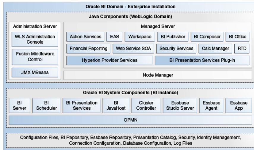
Figure 1–1 System Logical Architecture for Enterprise Install (Single Host)
