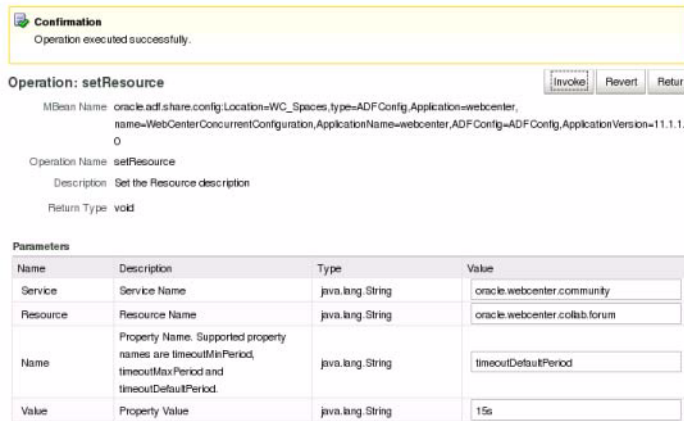
Figure 30–3 System MBean Browser - setResource
