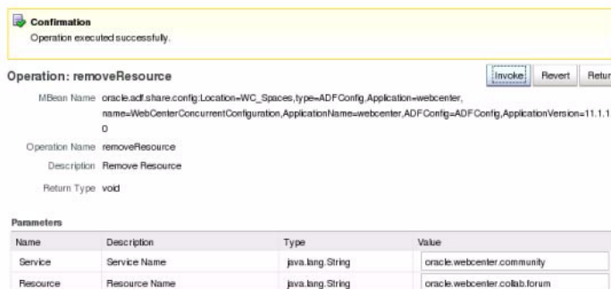
Figure 30–4 System MBean Browser - removeResource
