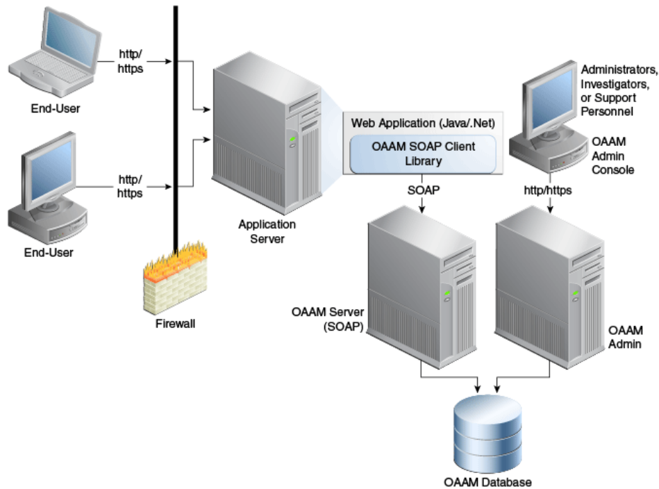
Figure 2-1 SOAP Service Wrapper API Integration
