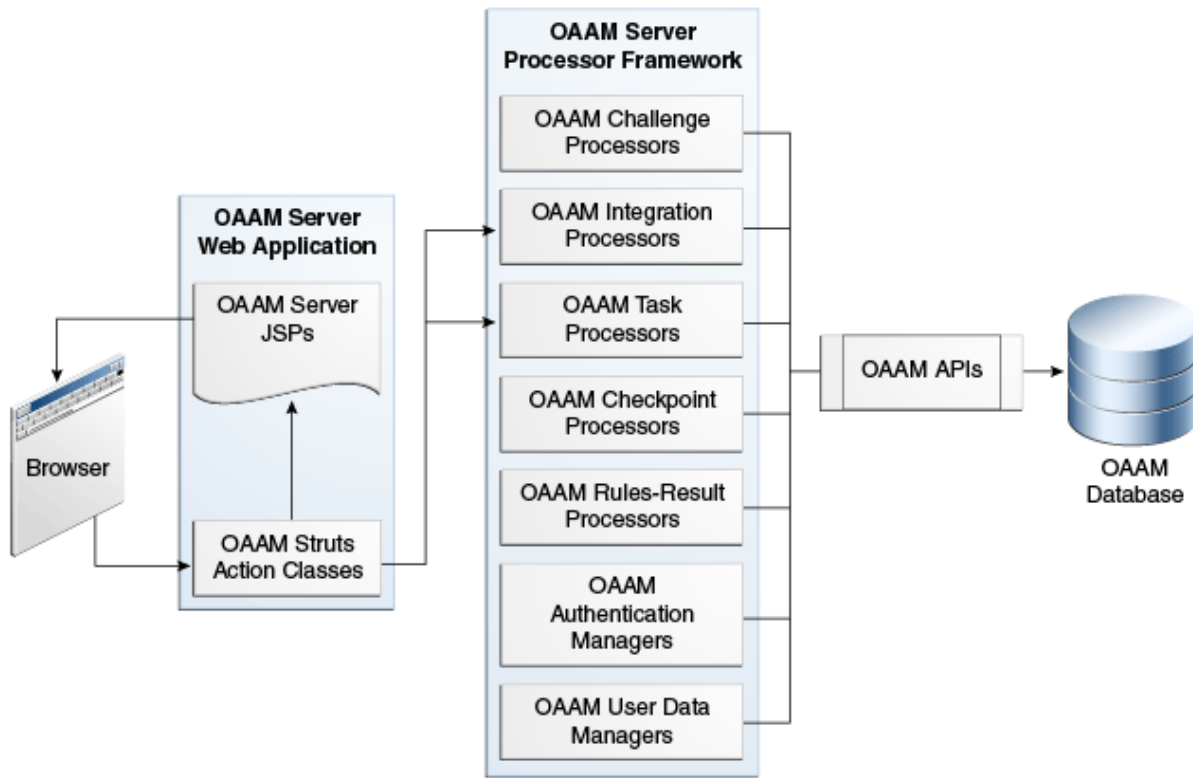
Figure 22–1 OAAM Processor Framework
