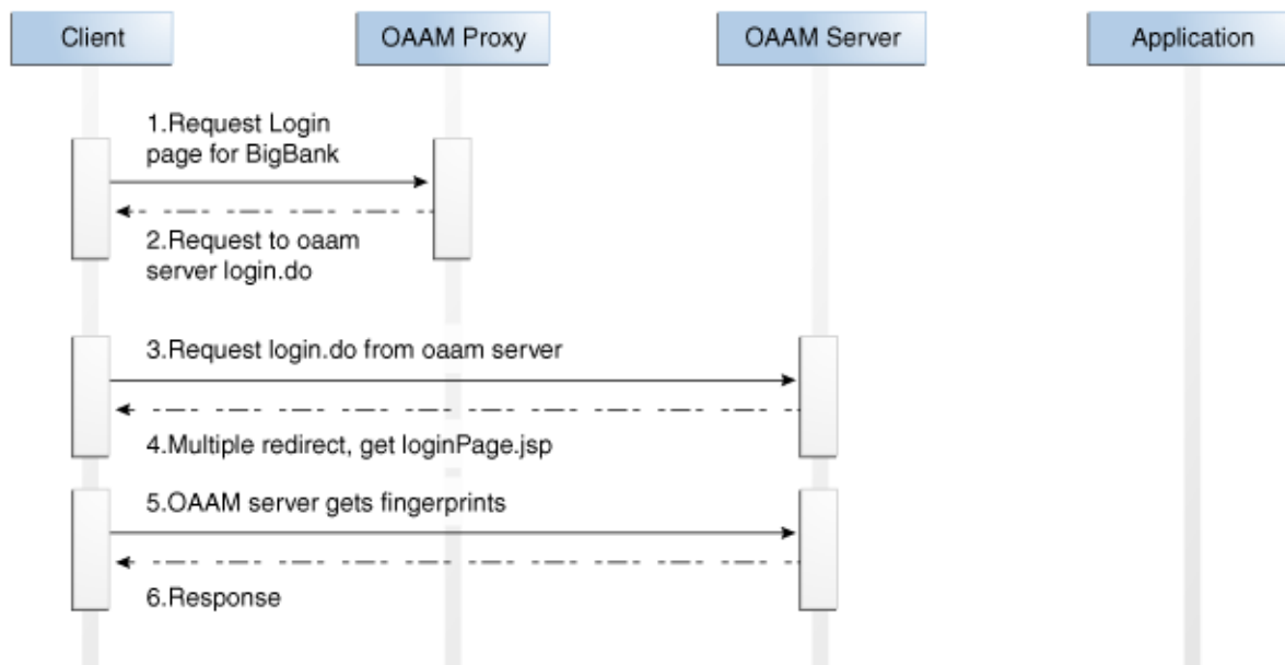
Figure 6–5 Flow for Getting Login Page
