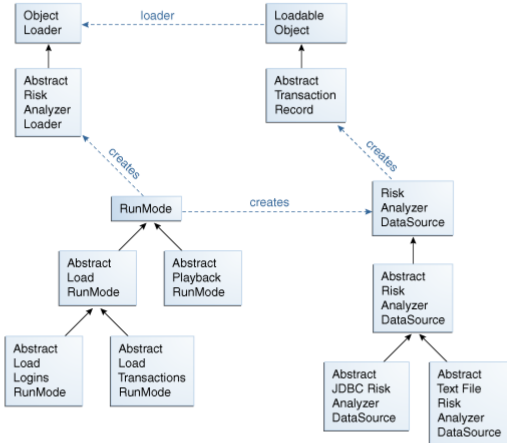
Figure 23–1 Basic Framework of a Custom Loader
