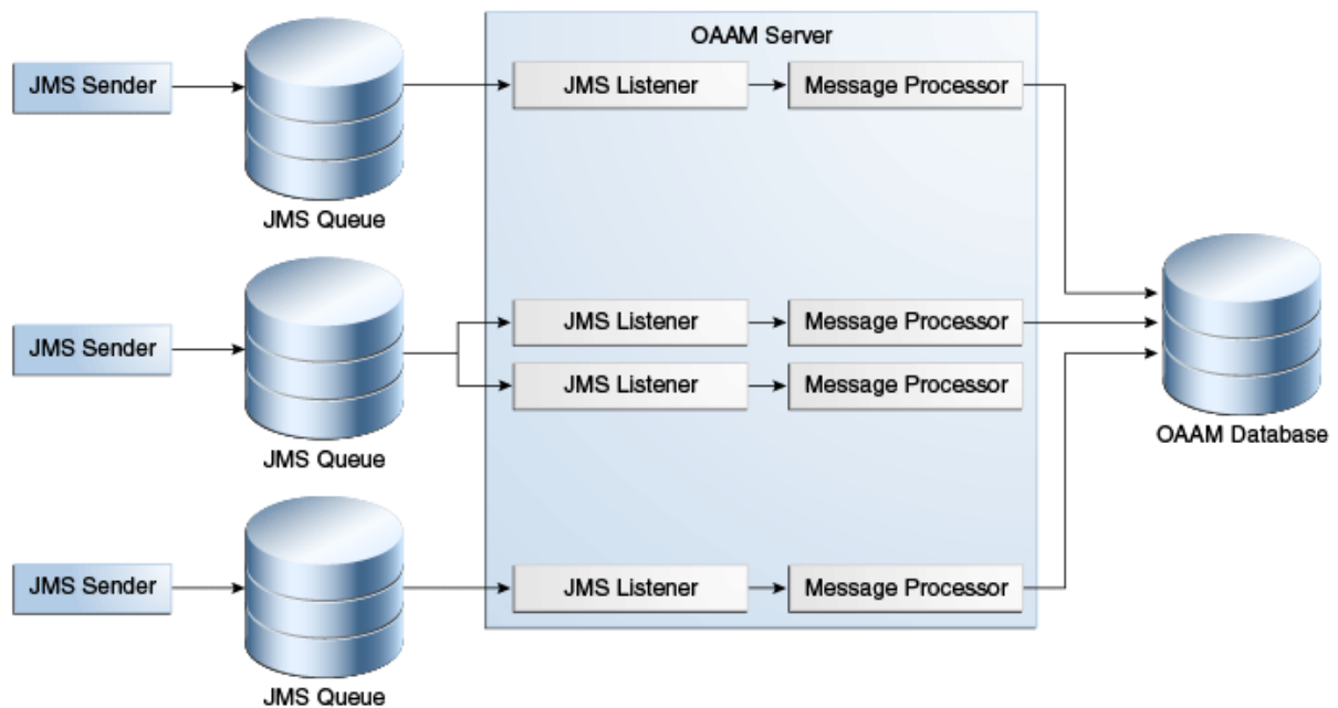
Figure 20–1 JMS integration with OAAM
