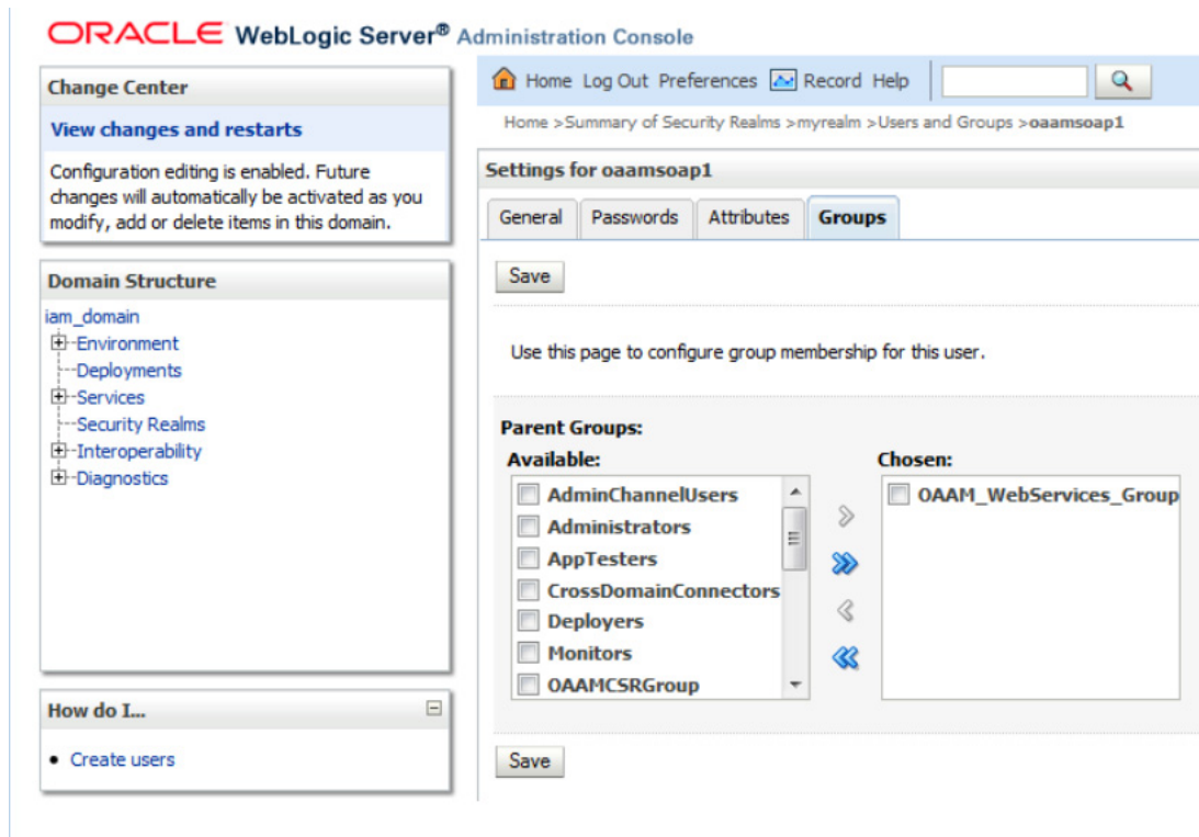
Figure 4–3 Configuring Group Membership for the User
