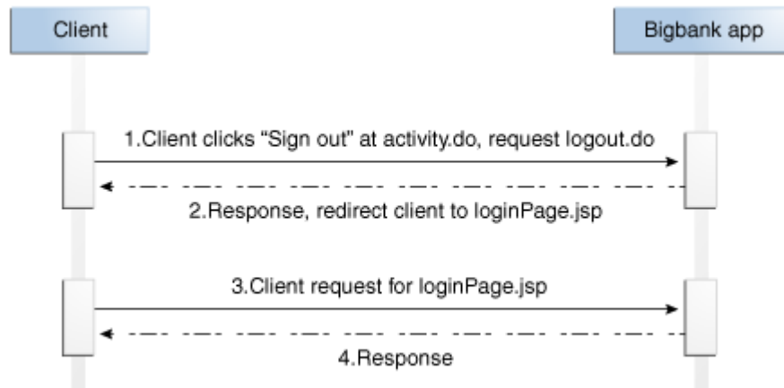
Figure 6-4 Logout - Without UIO Proxy
