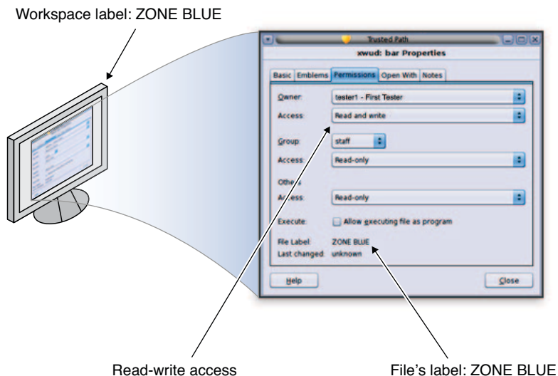
FIGURE 1-1 Comparing the Label of a Text Editor With the Label Property in the File Browser
