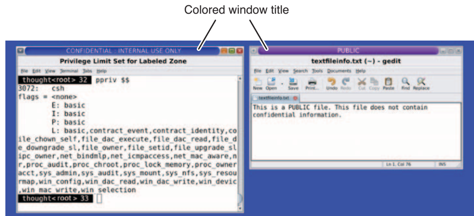
FIGURE 5-1 Window Labels With Colors From COLOR NAMES
