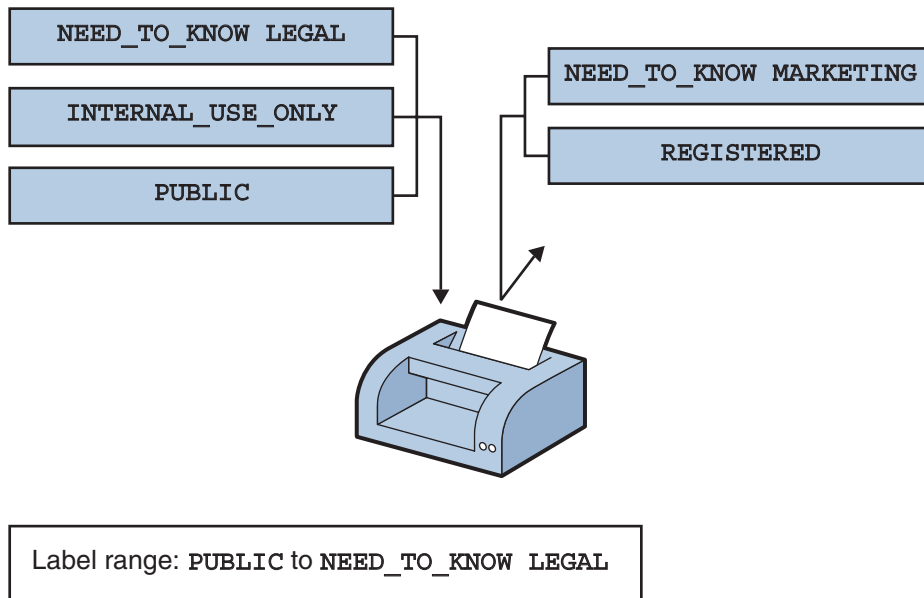
FIGURE 6–2 How a Printer With a Restricted Label Range Handles Print Jobs
