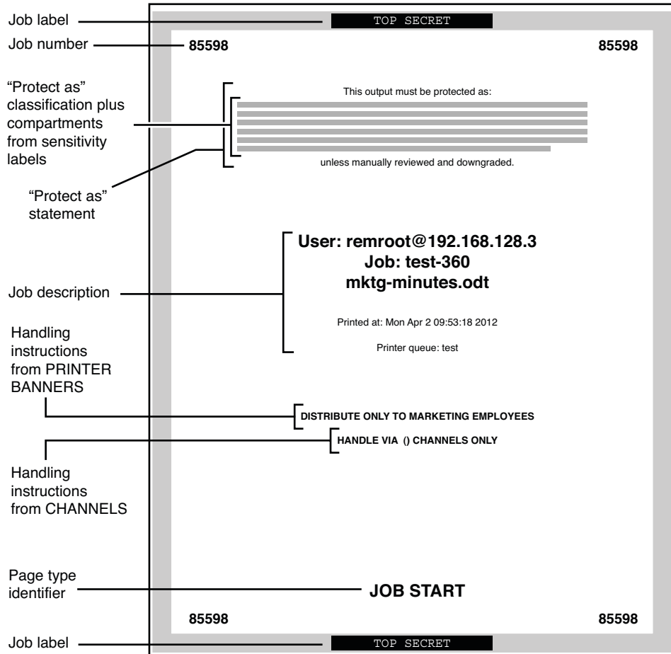
FIGURE 4-2 Typical Banner Page of a Labeled Print Job
