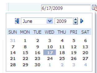
Figure 11–17 inputDate Component
