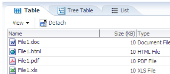
Figure 9-44 panelTabbed Panes
