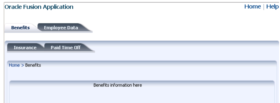
Figure 20–13 First-Level Page
