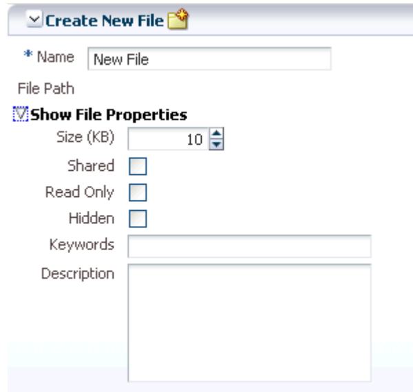
Figure 9–31 Expanded showDetail
