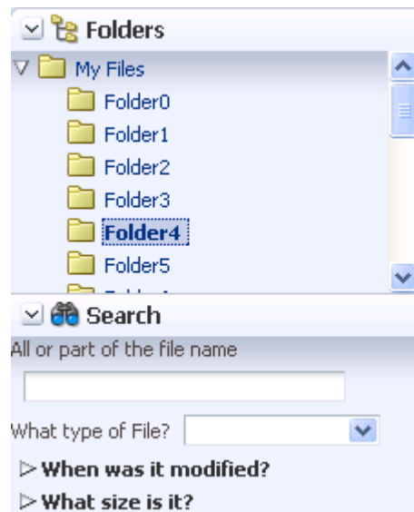
Figure 9–40 panelAccordion Panes
