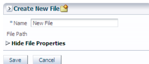
Figure 9–30 Collapsed showDetail
