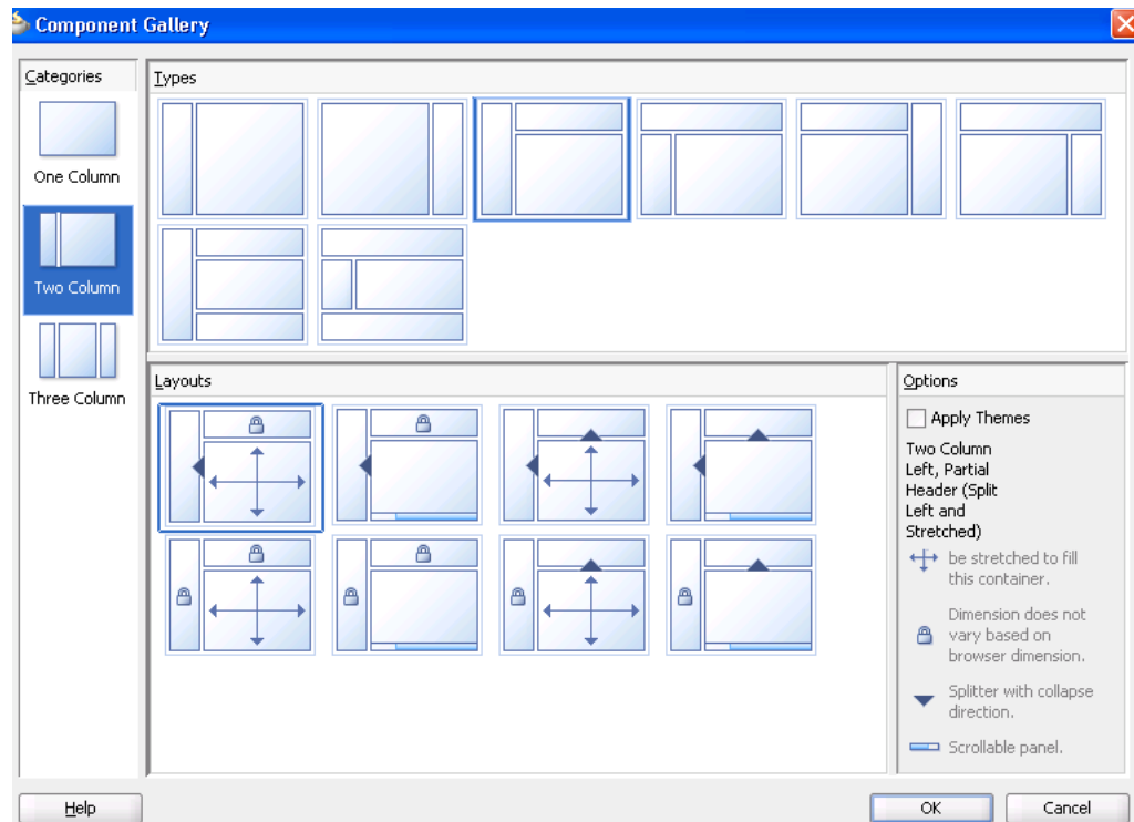
Figure 3-4 Quick Layouts
