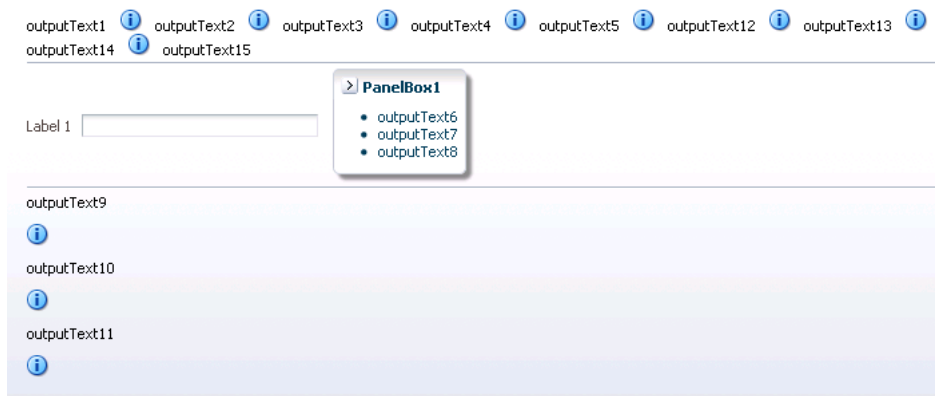
Figure 9–55 panelGroupLayout Arrangements
