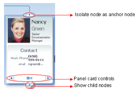
Figure 27–11 Node Controls
