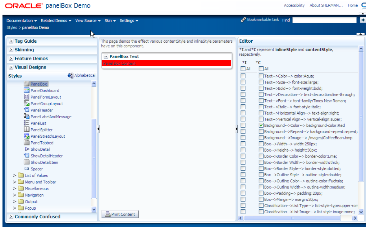
Figure 2-6 Styles Demonstration
