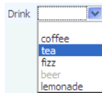
Figure 11–26 selectOneChoice Component
