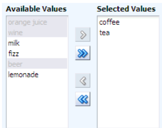
Figure 11–30 selectManyShuttle component
