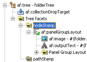
Figure 12–22 nodeStamp Facet in the Structure Window
