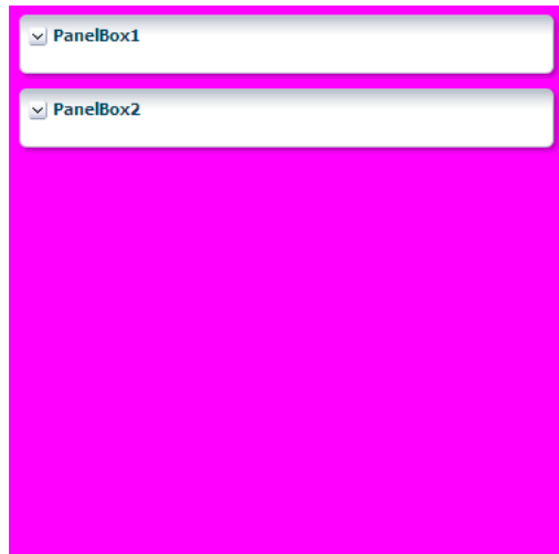
Figure 9–24 panelDashboard Stretches to Fill Space
