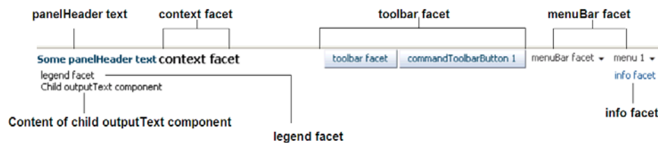
Figure 9-45 panelHeader and Its Facets
