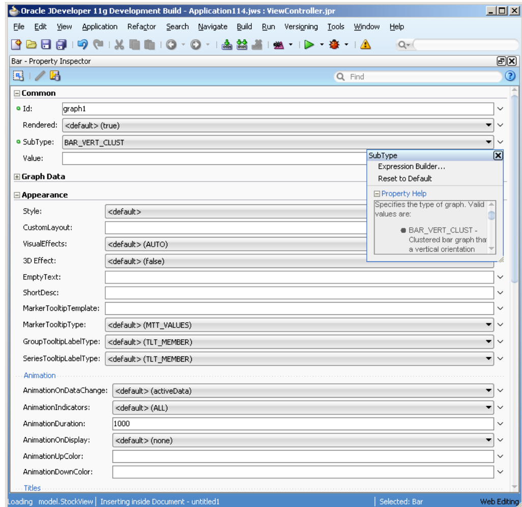
Figure 22–35 Bar Graph Component Value Attribute Dropdown Menu
