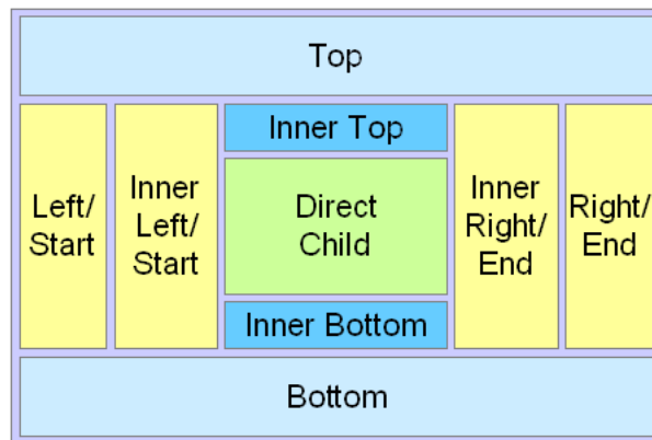
Figure 9–16 Facets in panelBorderLayout
