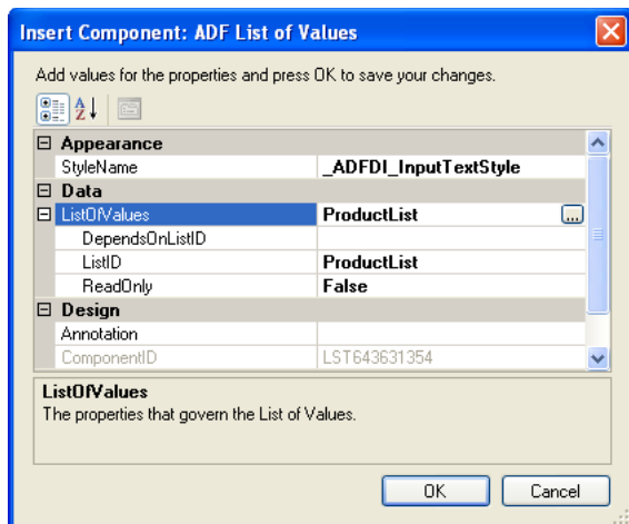
Figure 6–11 ADF List of Values Component
