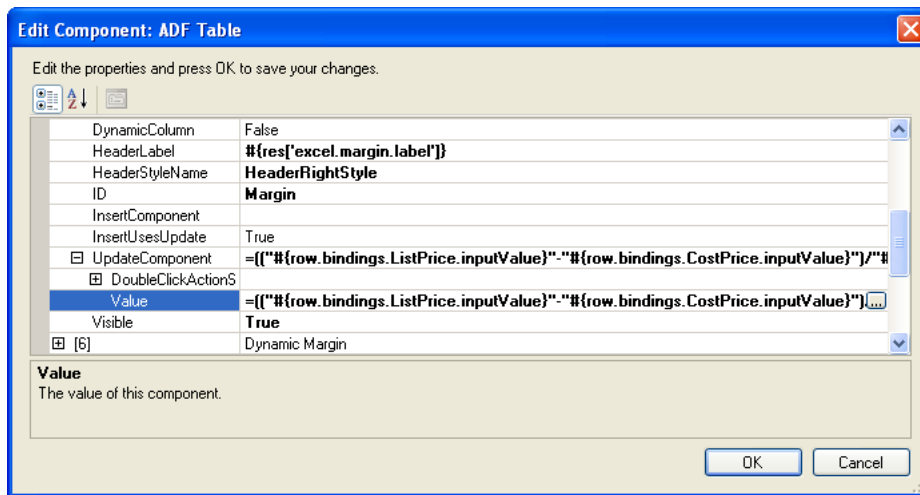
Figure 6–14 ADF Output Text Component That Displays Calculated Data
