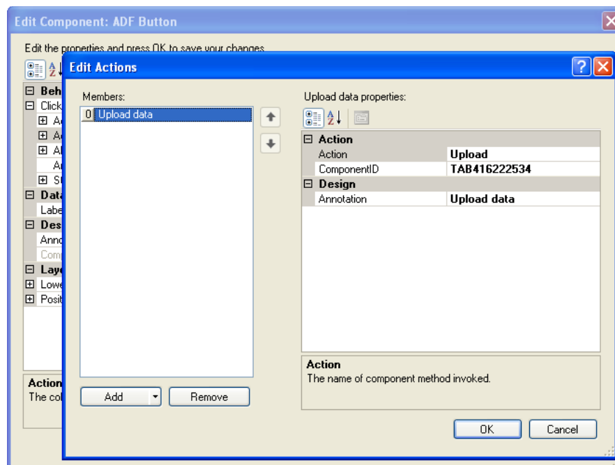
Figure 5–14 Collection Editor
