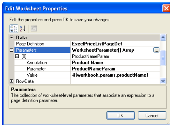
Figure 14–4 Worksheet Parameters
