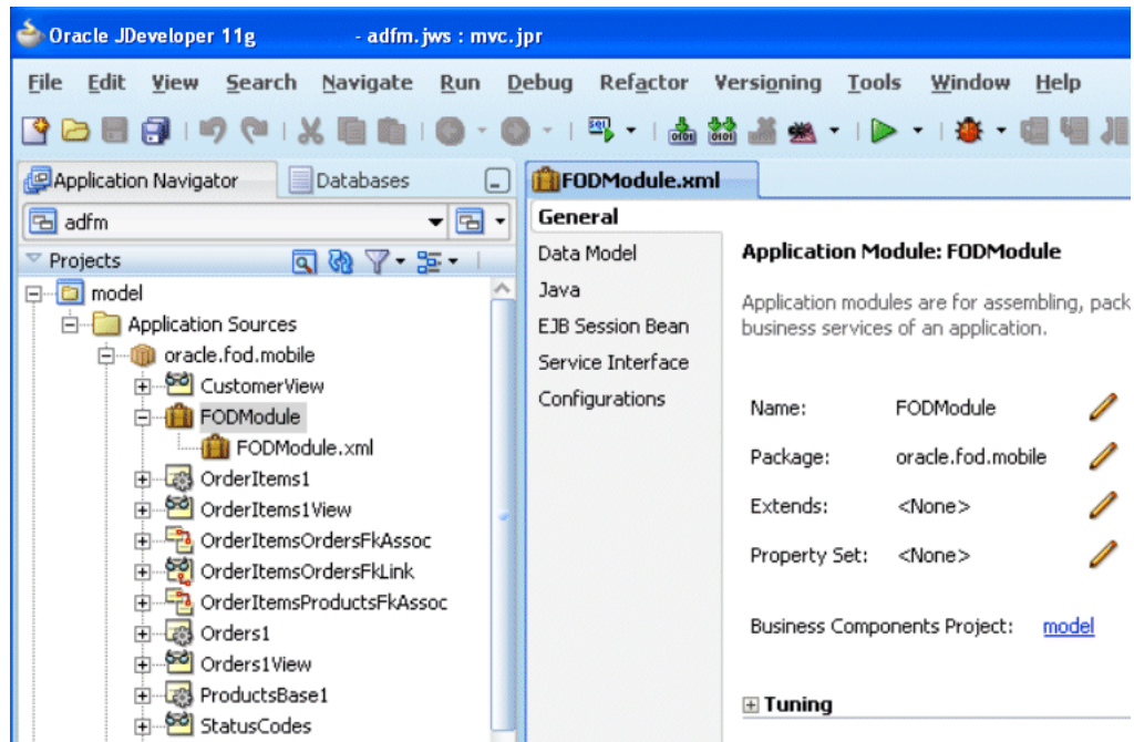
Figure 2–8 Creating a Business Components Project within an ADF Mobile Browser Application
