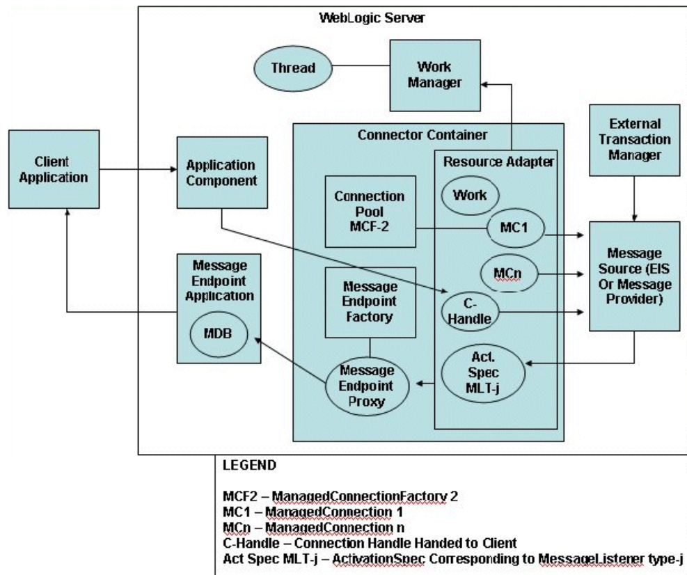
Figure 8–1 Messaging and Transactional Inflow Architecture
