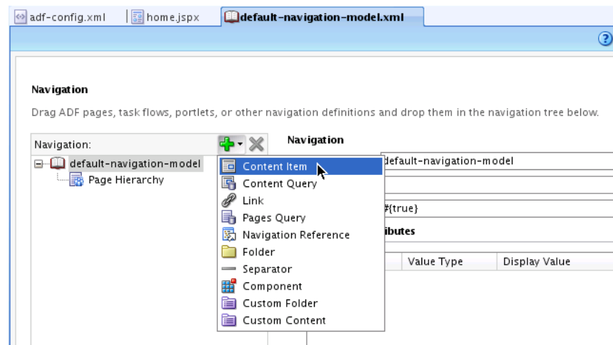
Figure 6–22 Adding a Content Item to the Default Navigation Model
