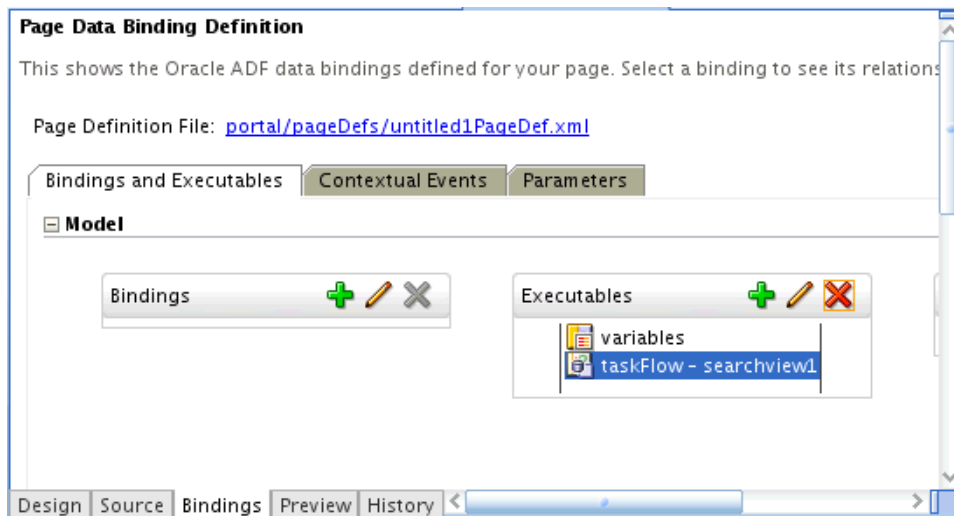
Figure 45-4 Page Data Binding Definition
