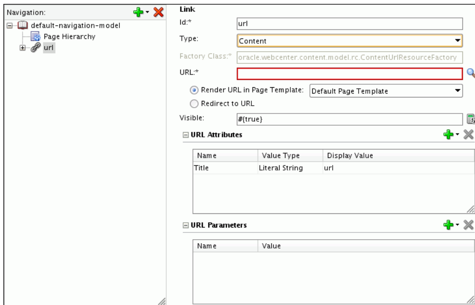
Figure 11–4 Adding a Content Item to a Navigation Model
