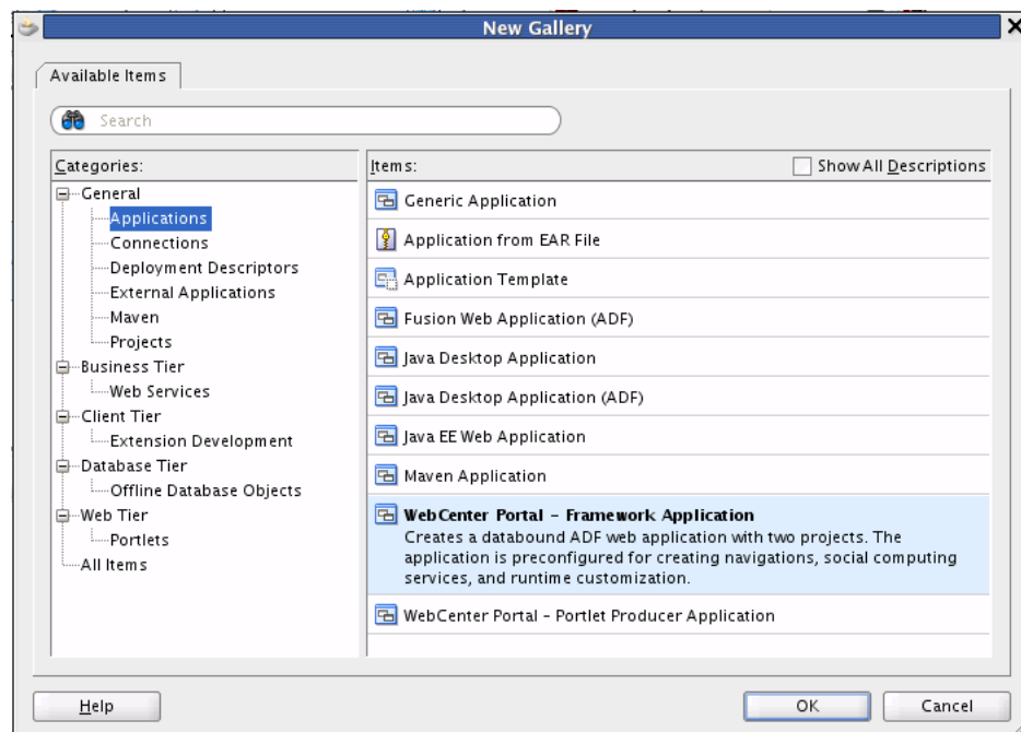
Figure 5–1 New Gallery Dialog
