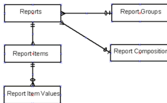
Figure I-4 Report Metadata Entities
