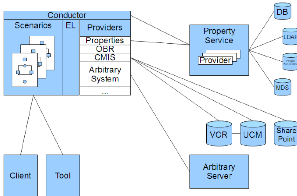
Figure 67–1 Personalization Services Architecture
