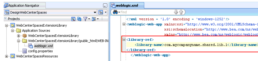
Figure 56–6 weblogic.xml - Single Shared Library Reference
