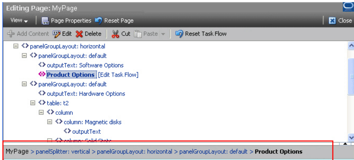
Figure 18–48 Bread Crumbs for a Component Selected in Page Source View
