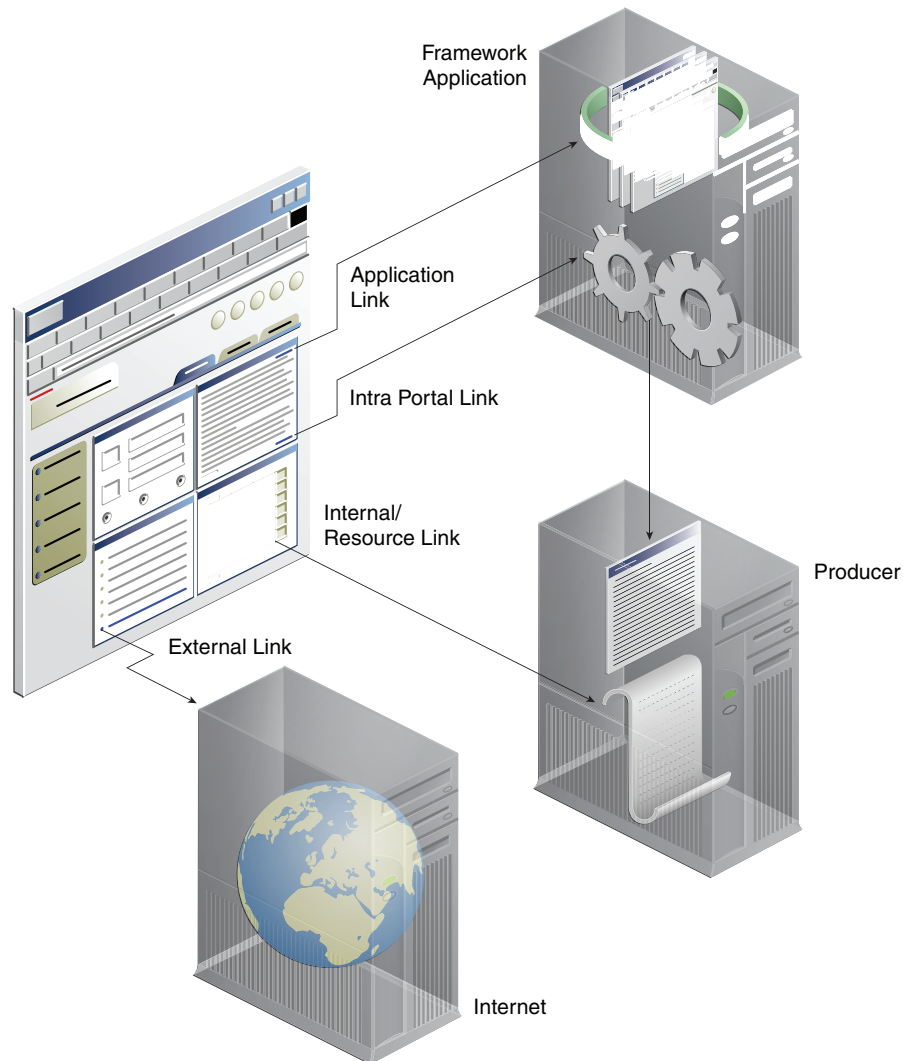
Figure 61–1 WebCenter Portal: Framework Application Link Types
