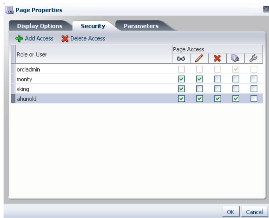
Figure 18-37 Security Tab on the Page Properties Dialog
