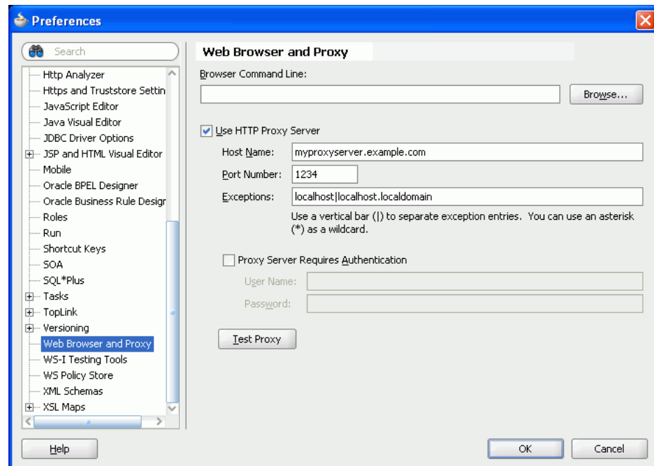
Figure 53–3 Setting Up a Proxy Server
