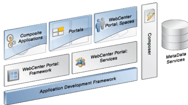
Figure 2–1 Overview of Oracle WebCenter Portal Architecture
