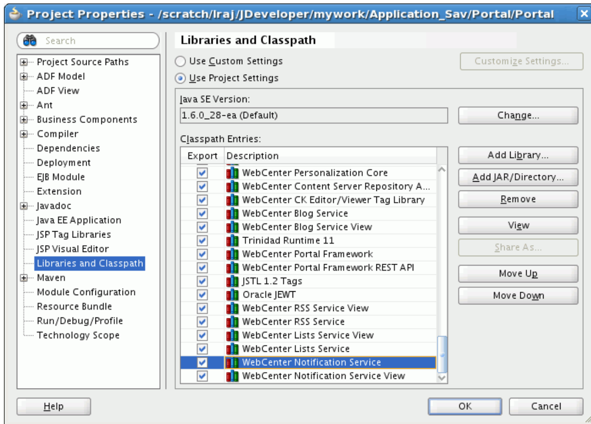
Figure 49–7 Libraries and Classpath in Project Properties
