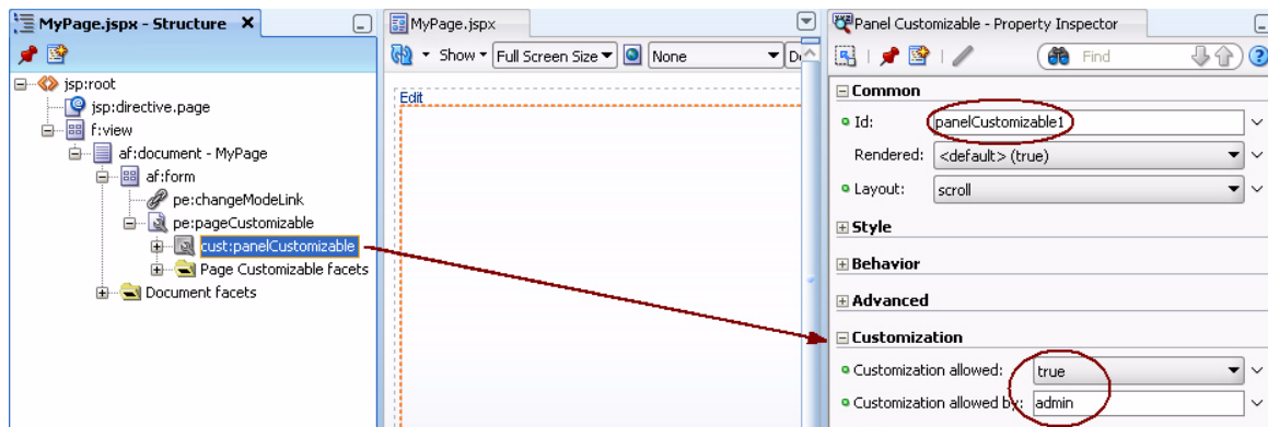
Figure 24-7 Design View: Customization Allowed
