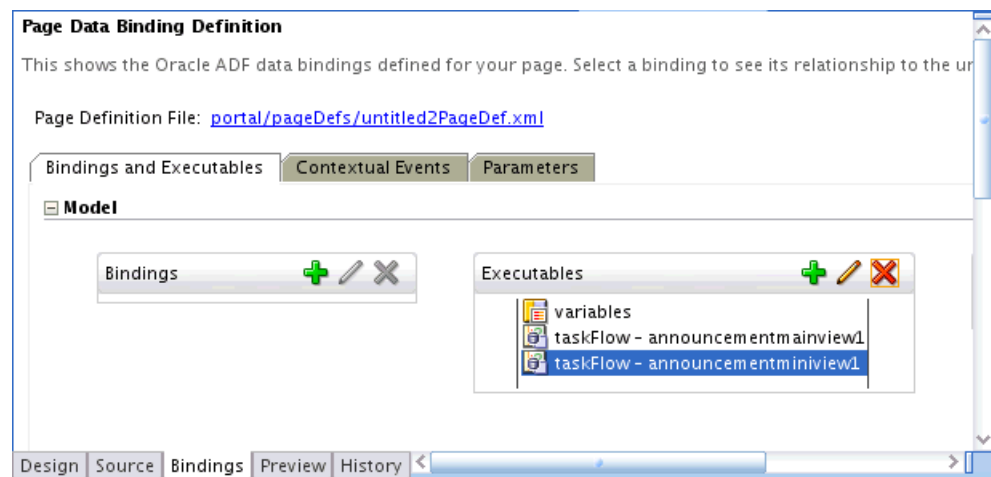
Figure 33–6 Page Data Binding Definition
