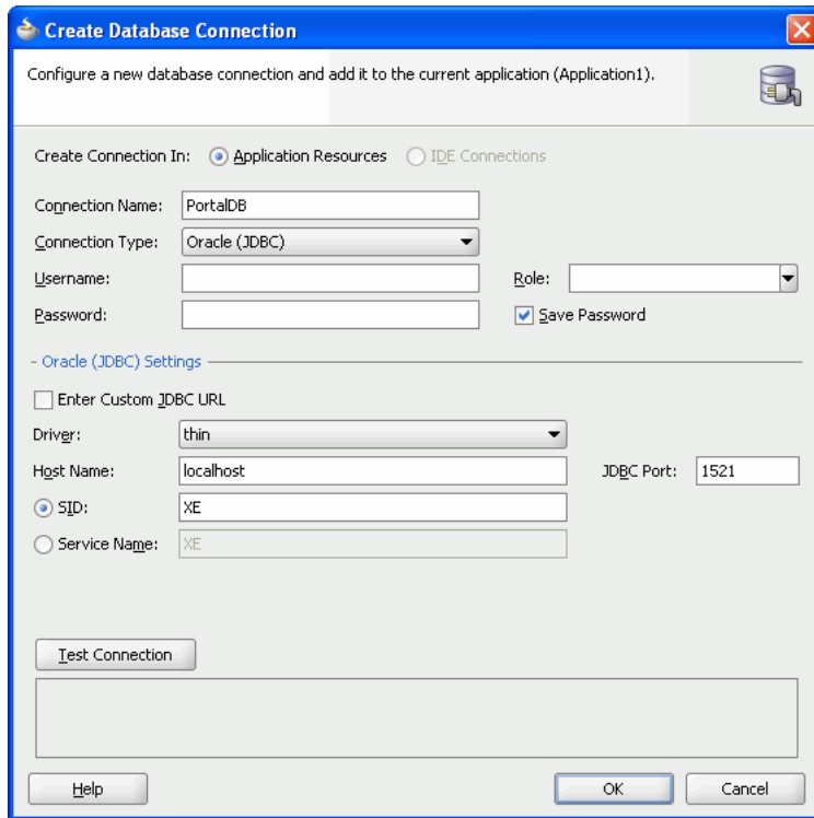
Figure 27–3 Create Database Connection
