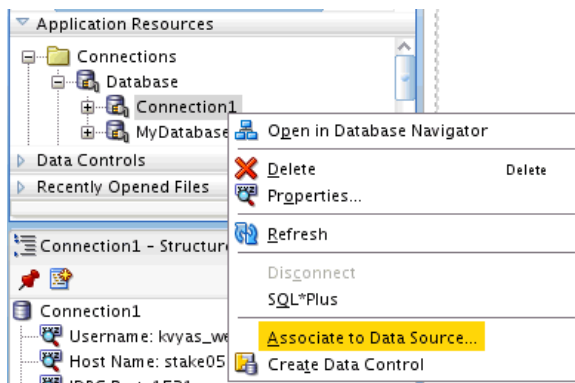
Figure 7-7 Associating to Data Source for Existing Connections
