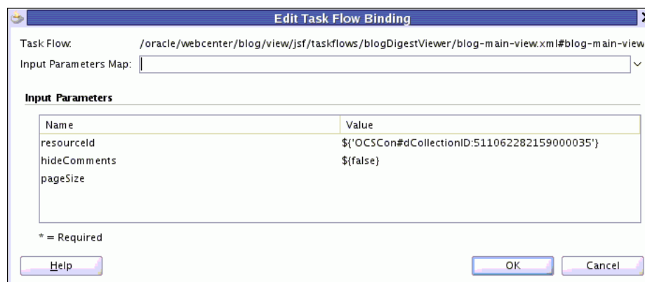
Figure 32–6 Specifying Parameters for Blogs Task Flow
