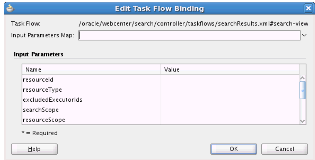
Figure 45–5 Edit Task Flow Binding Dialog for Search Task Flow
