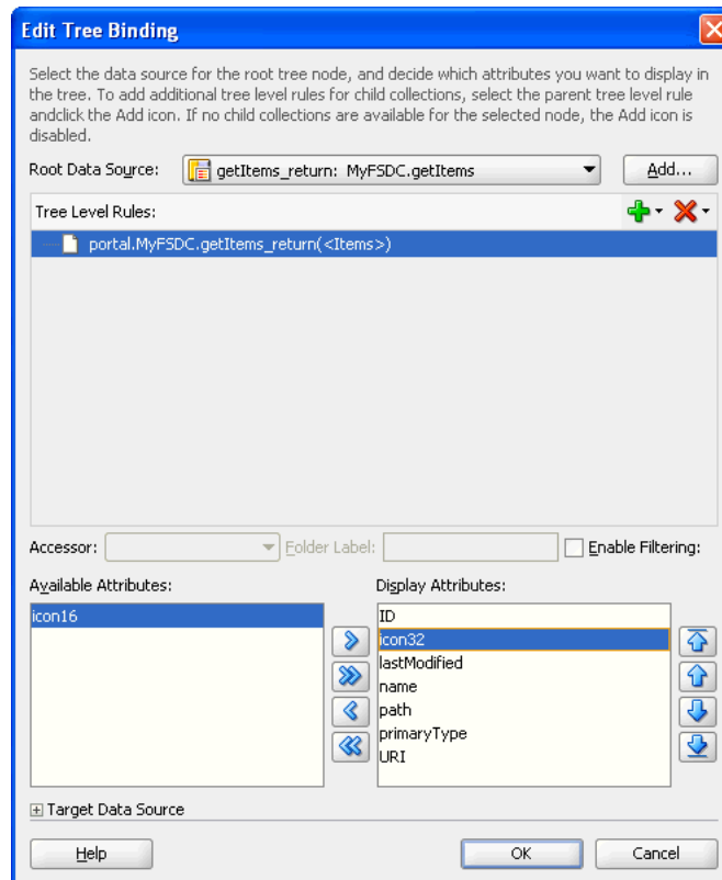
Figure 28–31 Edit Tree Binding
