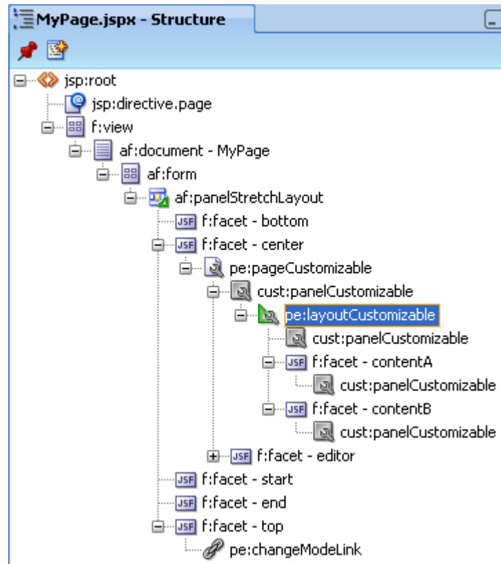
Figure 20–5 Layout Customizable Component
