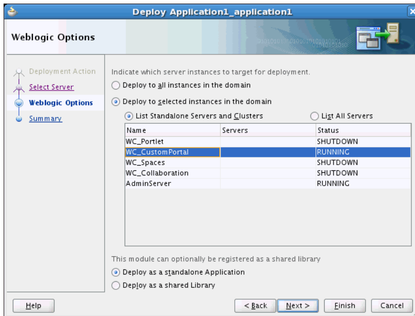
Figure 70–15 Deployment WebLogic Options dialog
