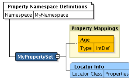
Figure 67–9 Design Pane - Property Definition
