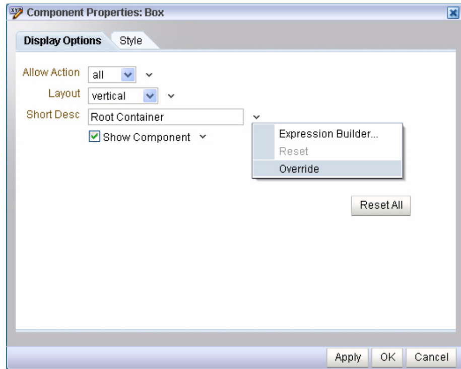
Figure 18–27 Reset and Override Options in the Component Properties Dialog
