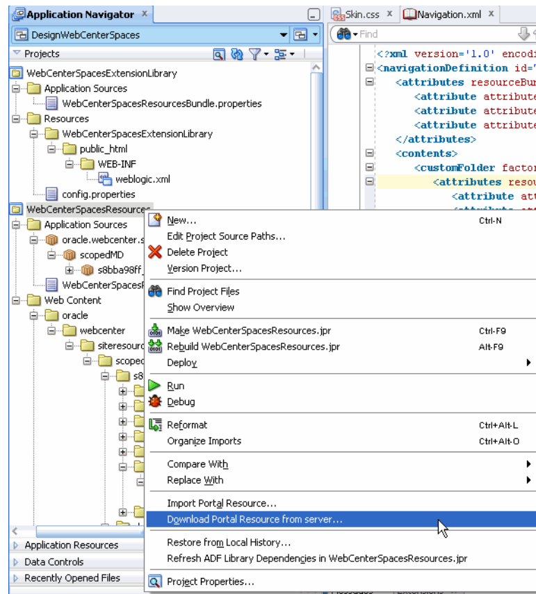
Figure 56–12 Download Portal Resource from Server Menu
