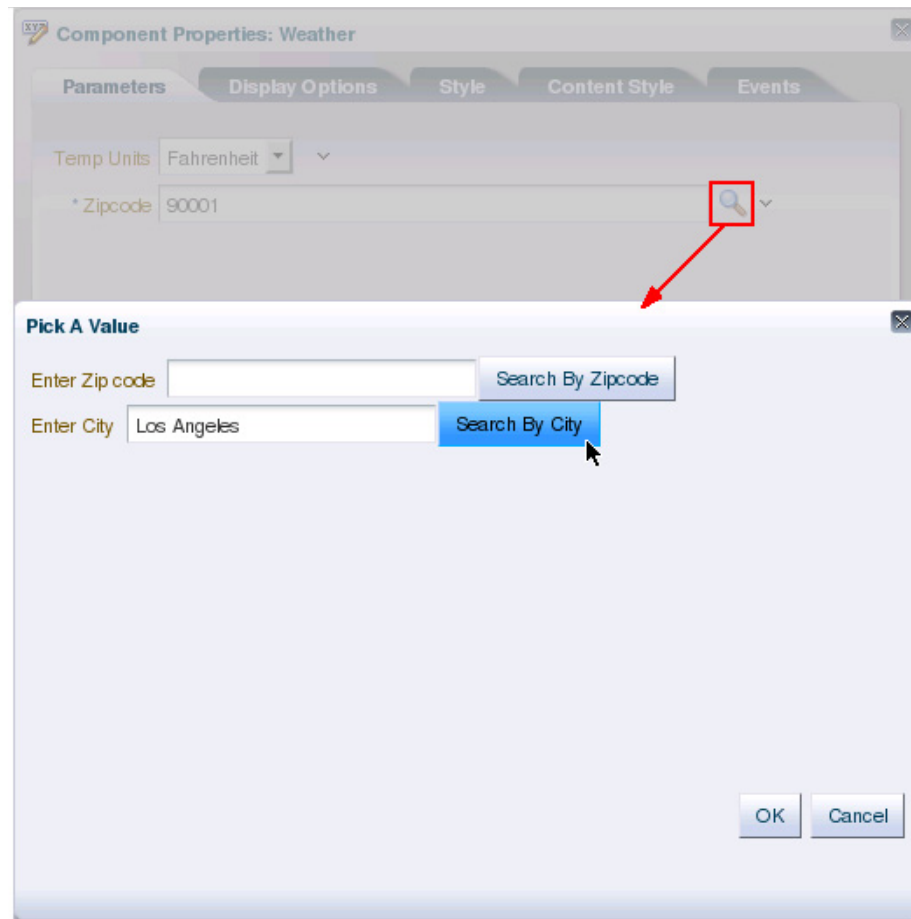
Figure 21–16 Picker Task Flow Configured for the Zipcode Field
