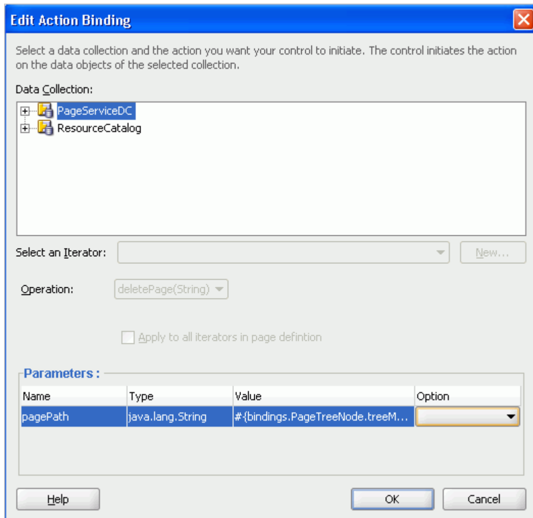
Figure 19–22 Edit Action Binding Dialog
