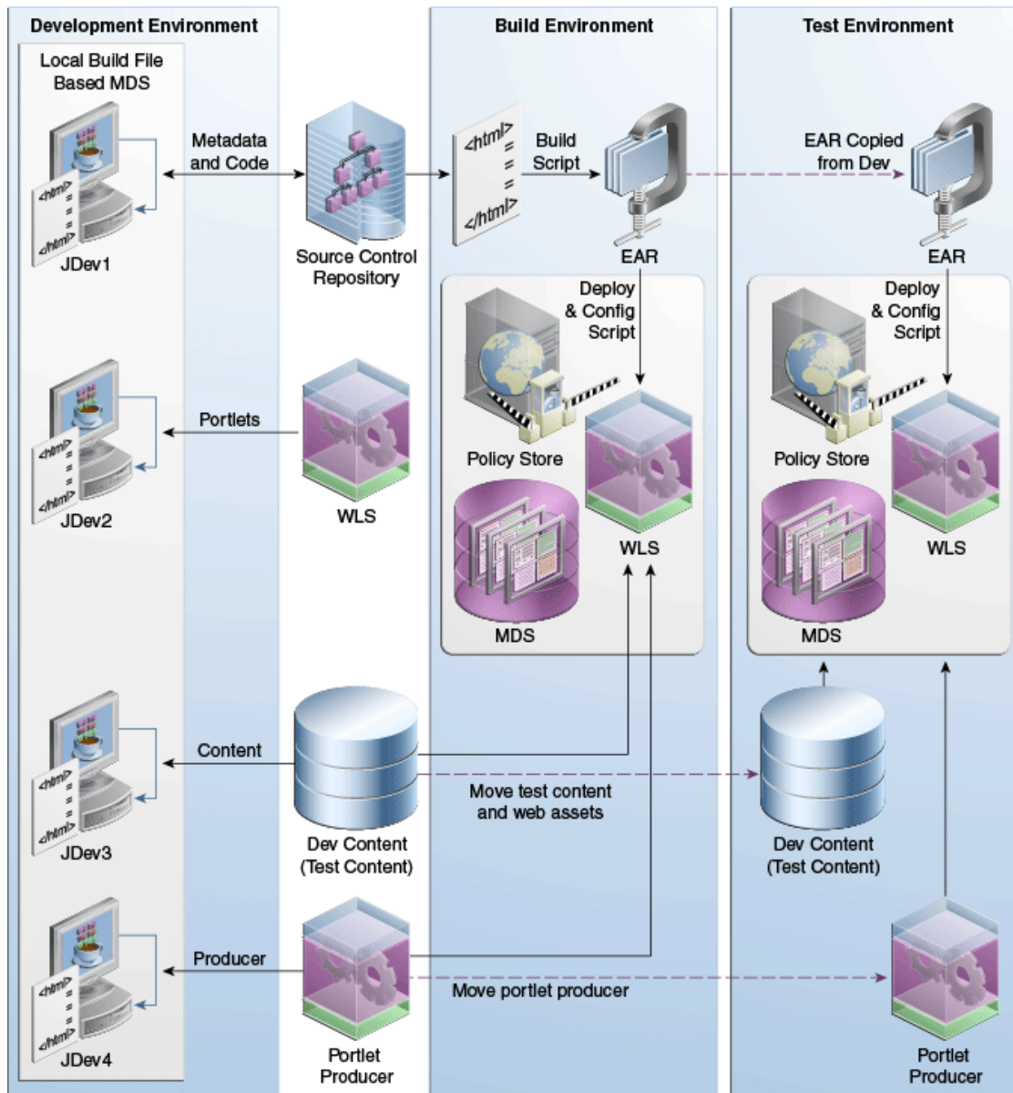
Figure 10–1 Flow from Development to Build to Test Environments
