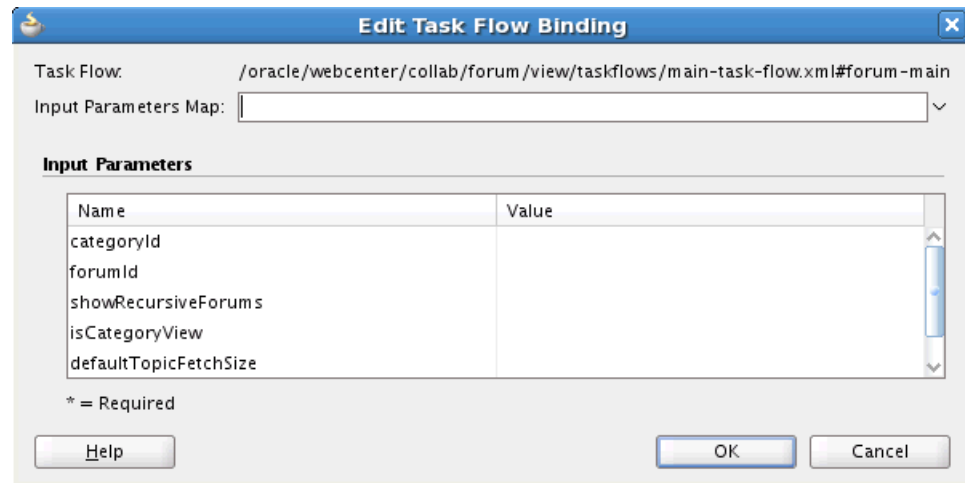
Figure 34–5 Edit Task Flow Binding Dialog for Discussion Forums Task Flow
