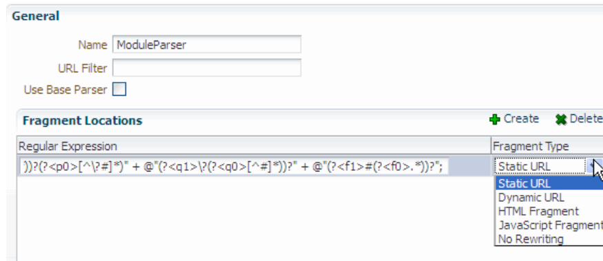
Figure 63–12 Pagelet Producer Console: Parsers - General Page
