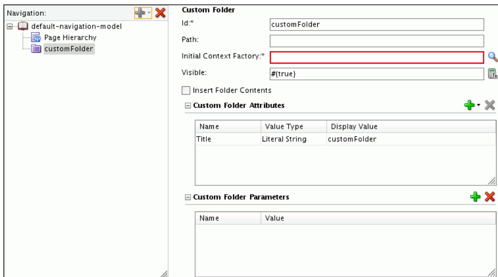
Figure 11–11 Adding a Custom Folder to a Navigation Model
