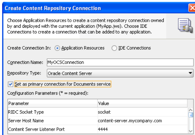
Figure 27–1 Content Repository Connection - Content Server
