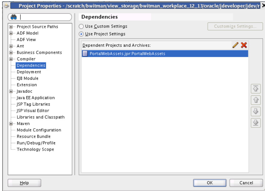
Figure 5-9 Project Dependencies Dialog
