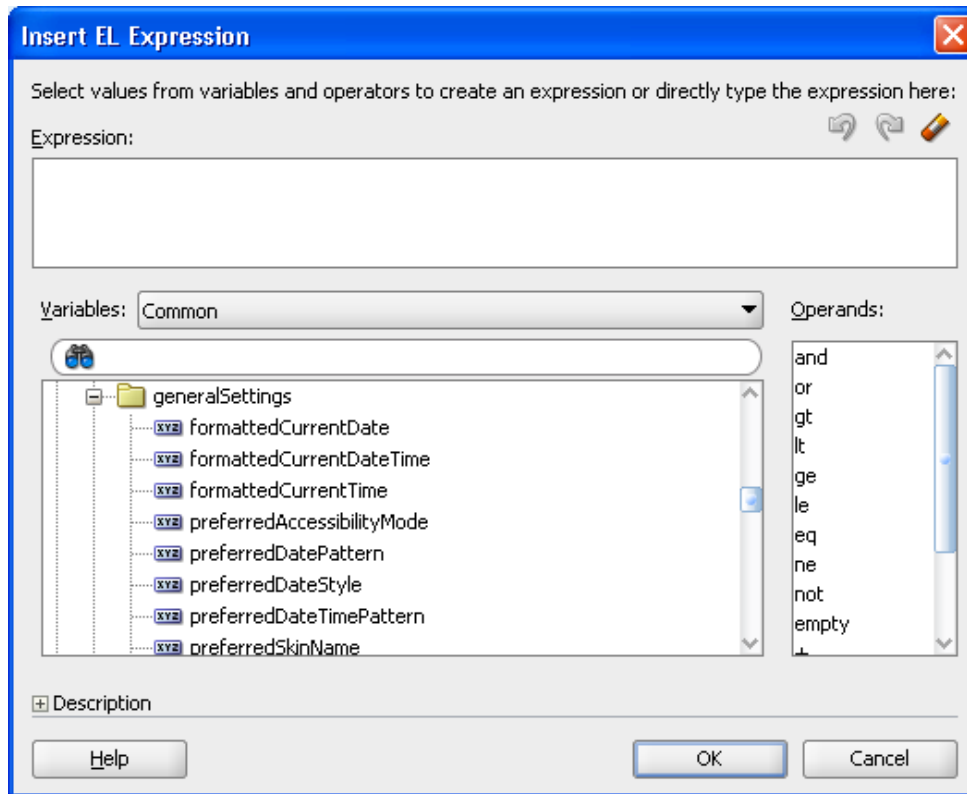
Figure 7–9 Expression Builder for the generalSettings JSF Managed Bean
