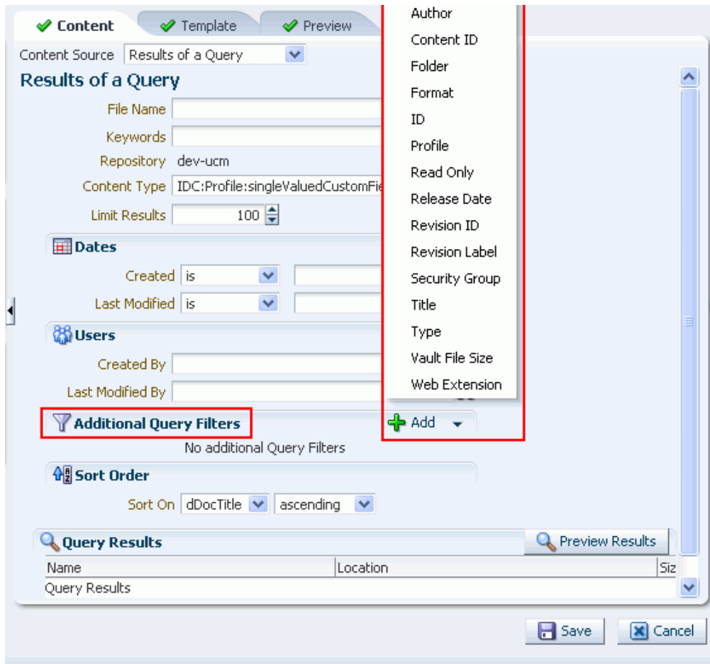
Figure 29–4 Identifying Content Type Properties
