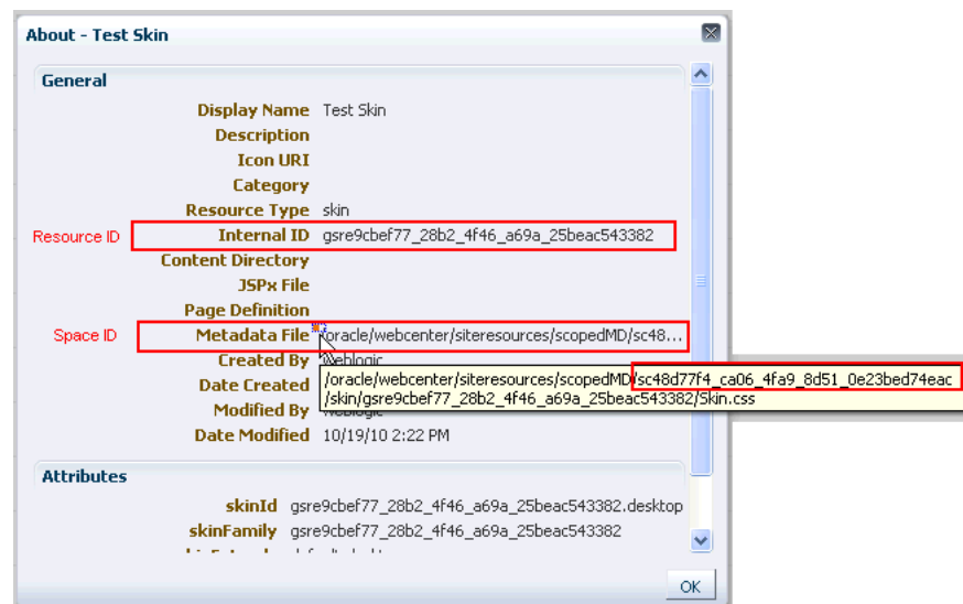
Figure 56–15 Checking Resource IDs in Spaces
