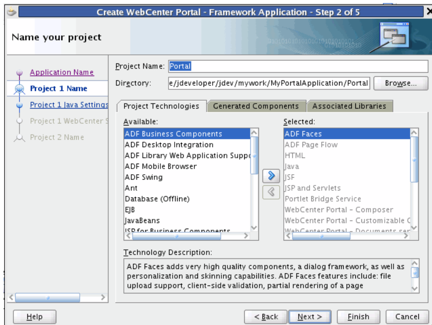
Figure 6–1 Create WebCenter Portal: Framework Application Wizard Step 2 of 5
