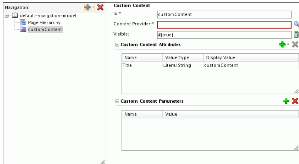
Figure 11–12 Adding a Custom Content Provider to a Navigation Model
