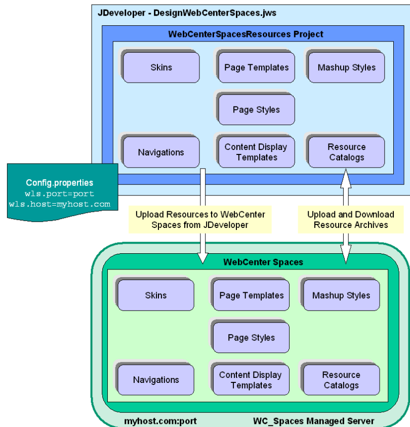
Figure 56–9 Designing Resources Using the WebCenterSpacesResources Project
