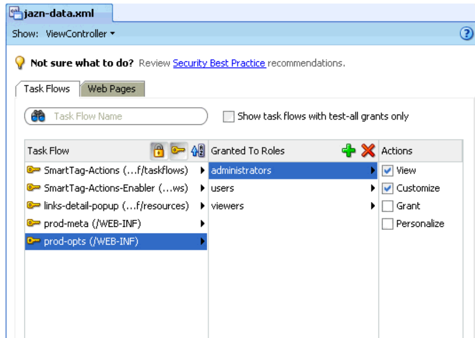
Figure 24–10 Task Flow Security Region in the jazn-data.xml File
