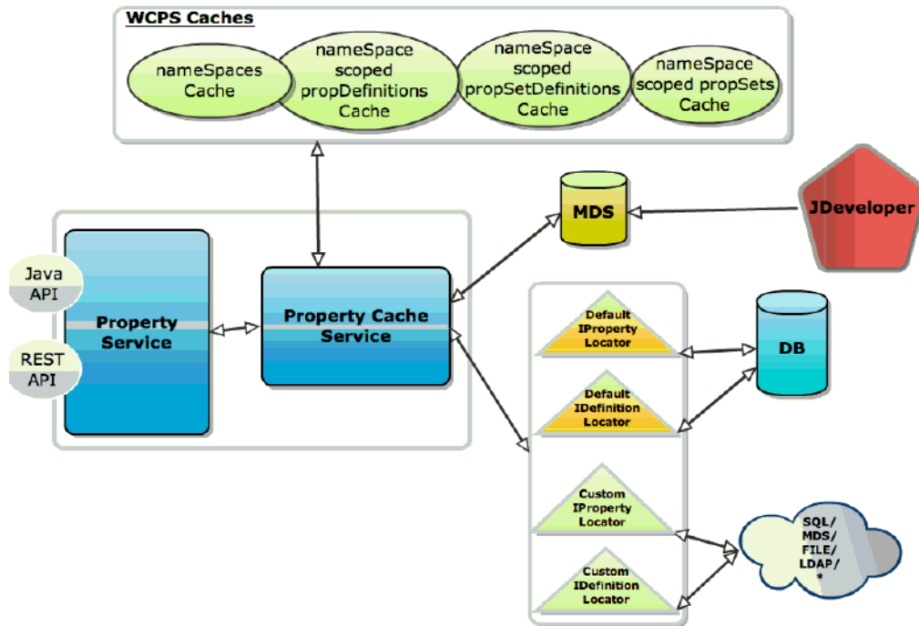
Figure 67–2 Property Service Architecture
