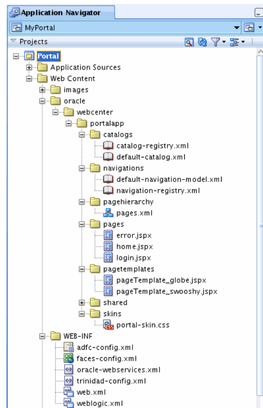
Figure 9–22 WebCenter Portal: Framework Application in the Application Navigator
