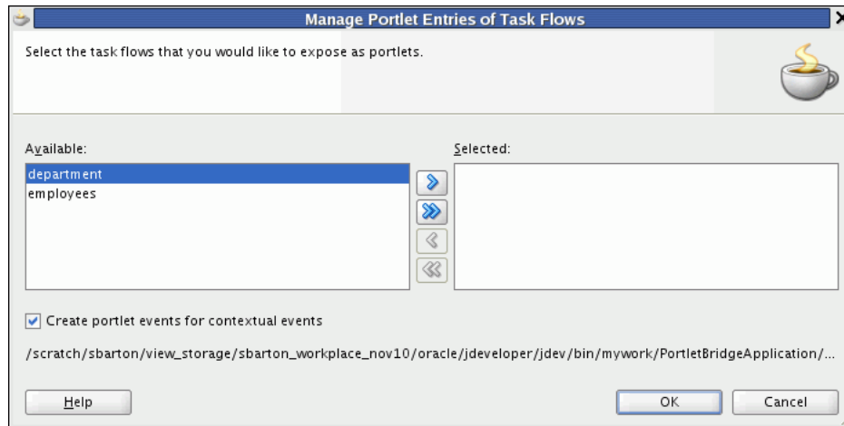
Figure 59–3 The Manage Portlet Entries of Task Flows Dialog
