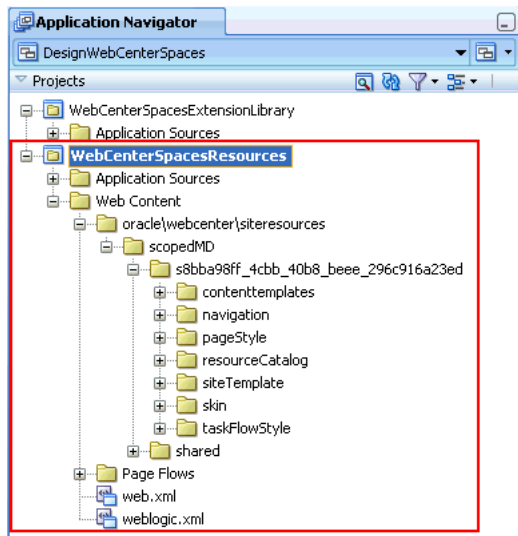
Figure 56–11 Exploring the WebCenterSpacesResources Project in JDeveloper
