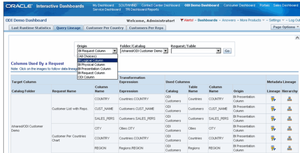
Figure 19–4 Resulting Dashboard
