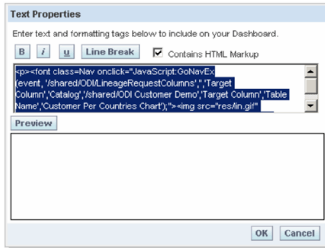
Figure 19–7 Text Properties Editor
