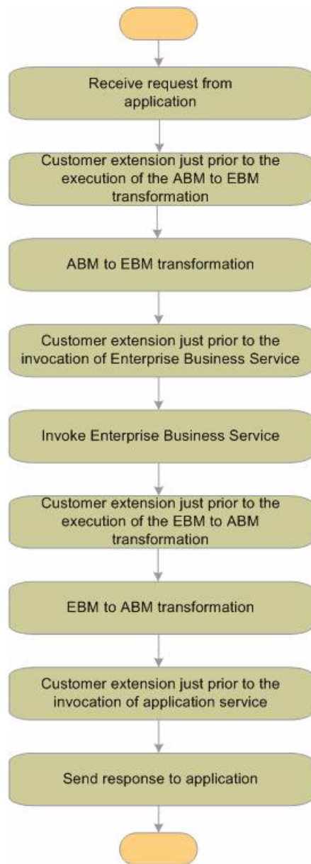
Figure 4–3 depicts the high-level flow of activities in a requester-specific ABCS. The diagram makes an assumption that the EBS with which it is interacting employs a fire-and-forget interaction style. The steps for running the extension to do additional transformations are optional.
