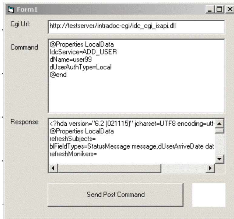
Figure 22–12 Visual Interface with Returned Results
