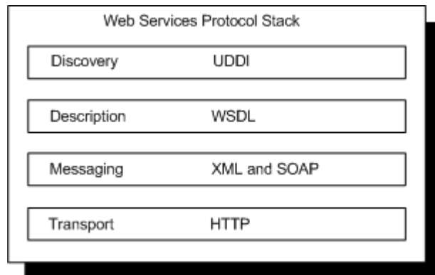
Figure 25–1 Layers of the Web Services Protocol Stack
