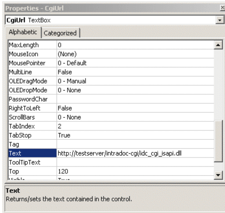
Figure 22-3 Edited CgiUrl TextBox Properties
