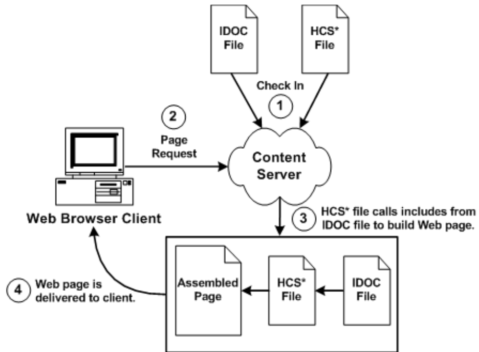
Figure 4-1 The Dynamic Server Page Process
