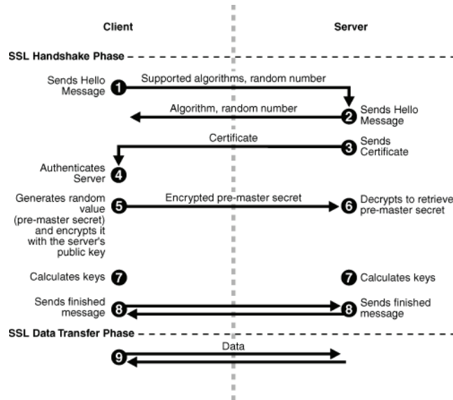
Figure 6–1 SSL Handshake
