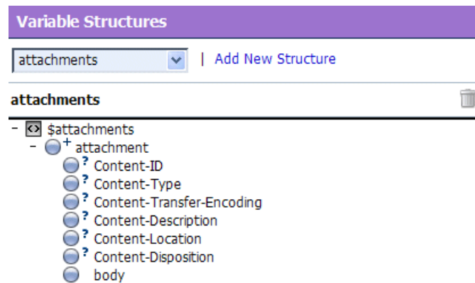
Figure 37–10 Variable Structures—attachments
