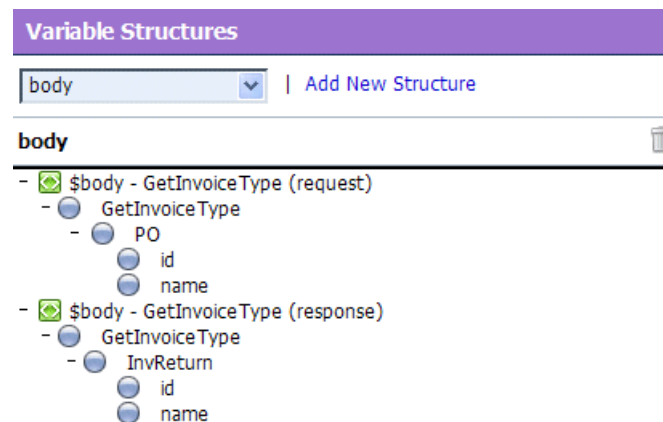
Figure 37-4 Variable Structures—body
