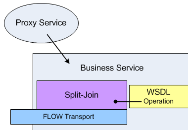
Figure 38–3 Split-Join framework
