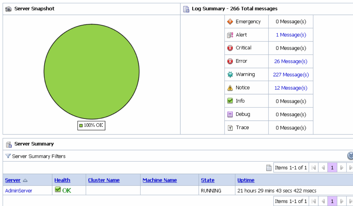
Figure 46–19 Server Health
