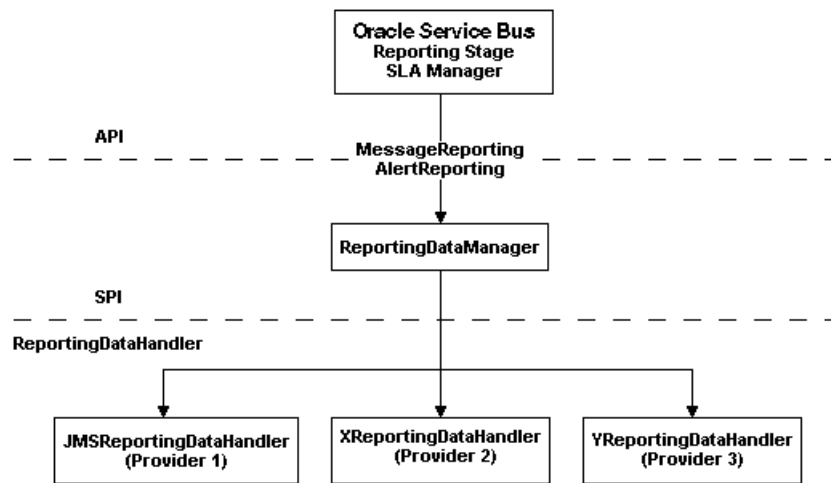
Figure 47-1 Reporting Framework
