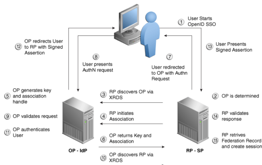
Figure 2-6 OpenID Processing Flow
