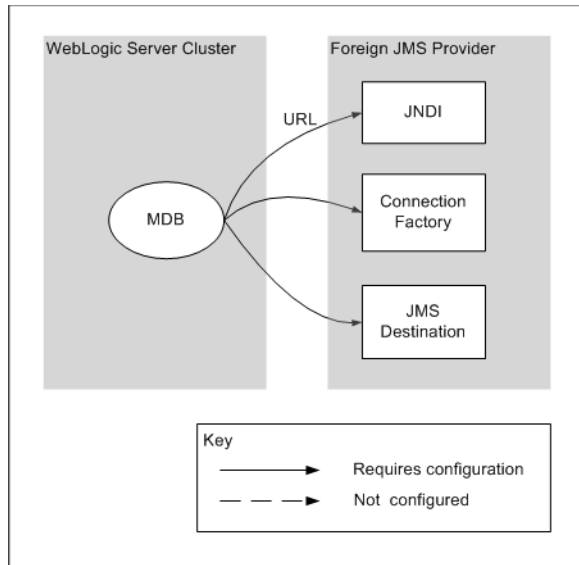
Figure 6-3 C. Destination on Foreign JMS Server—No Mappings
