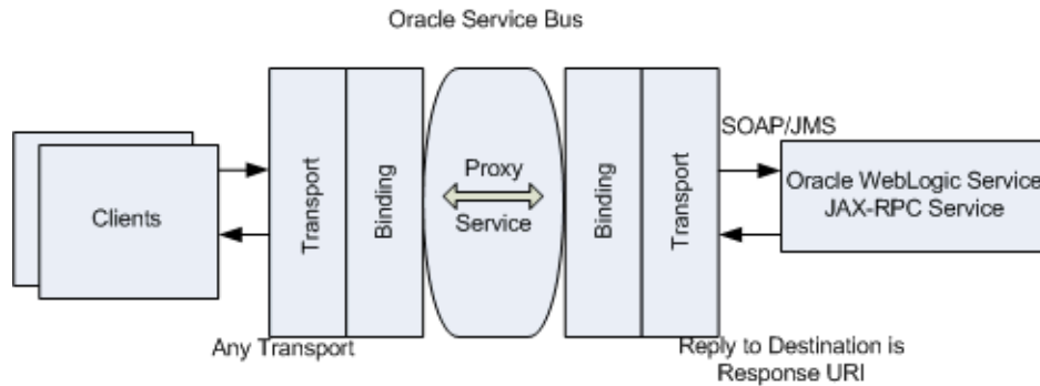
Figure 31-3 Oracle Service Bus as a Client of an Oracle WebLogic Server JAX-RPC Request/Response Service
