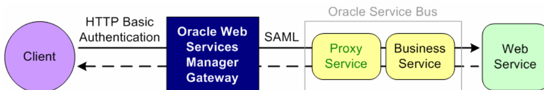
Figure 51–7 Identity Propagation with Oracle Web Services Manager Gateway
