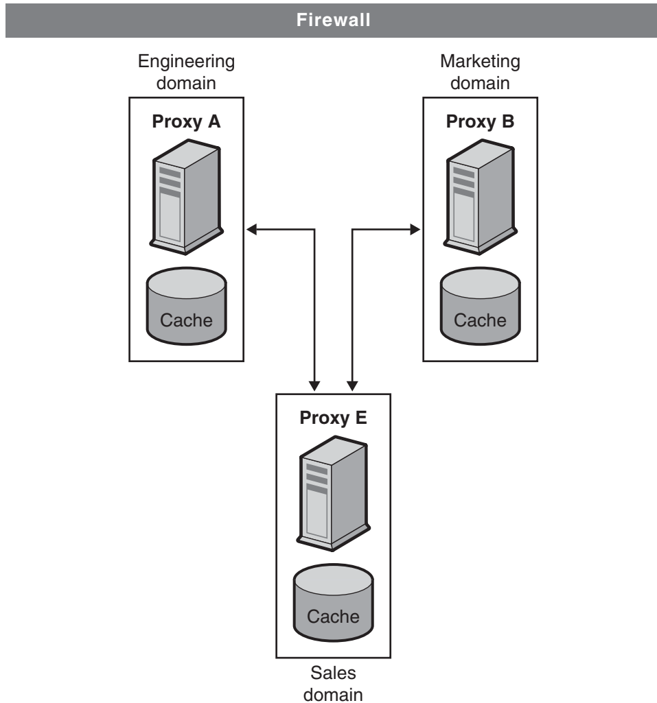
FIGURE 12-3 ICP Exchange
