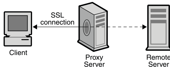
FIGURE 5-1 SSL Connection
