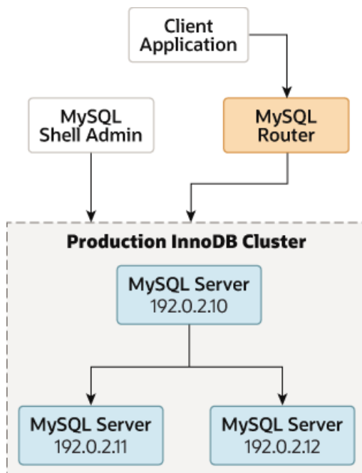
Figure 8.2 Production Deployment
